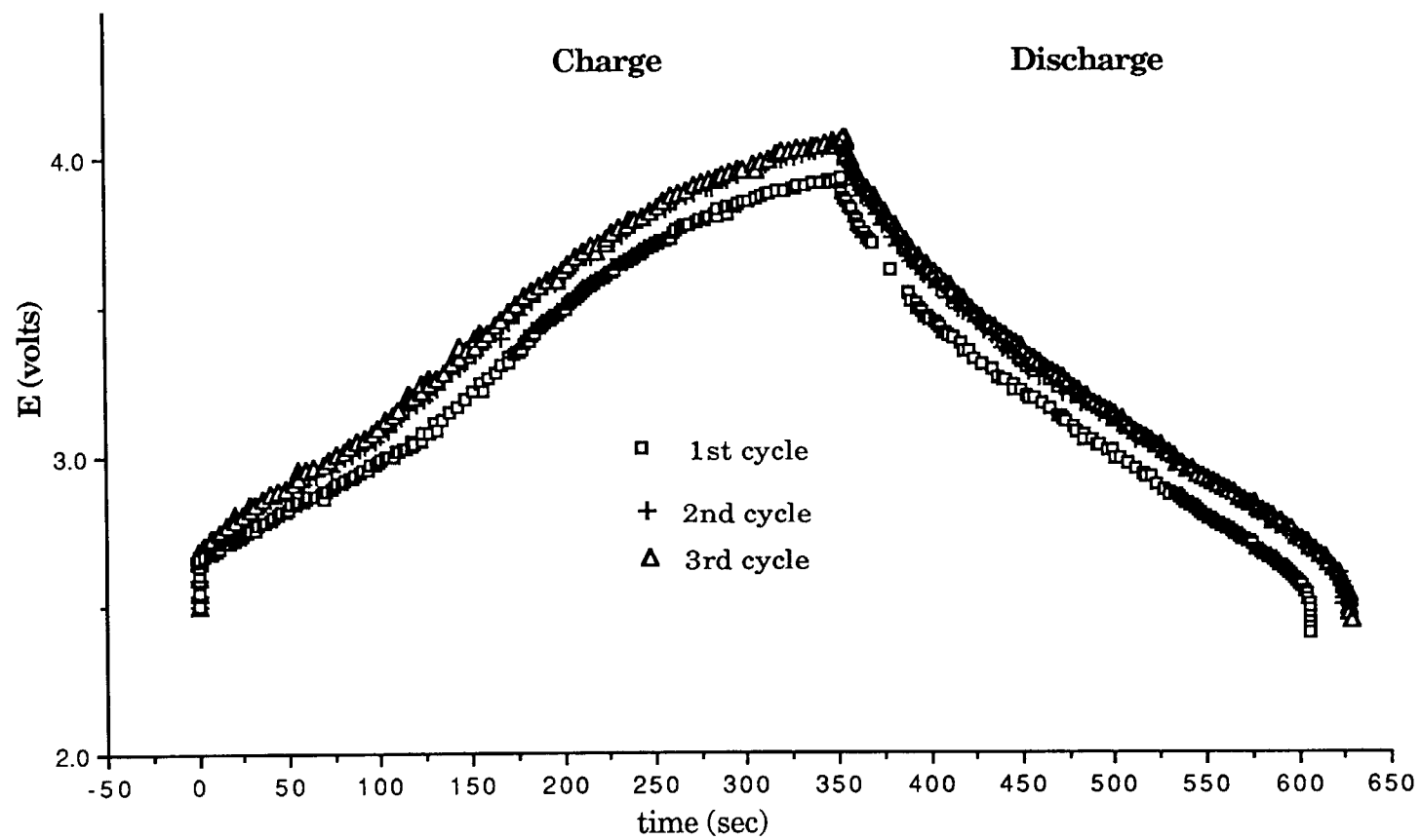
Fig. 38. Charge/Discharge Curves of Li/PPy Fibrillar Film Battery Using 2Q CV Charge.
