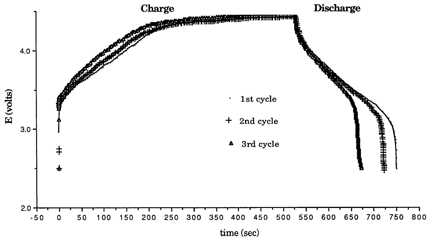
Fig. 35. Charge/Discharge Curves of Li/PPy Conventional Film Battery Using 3Q CV Charge.
