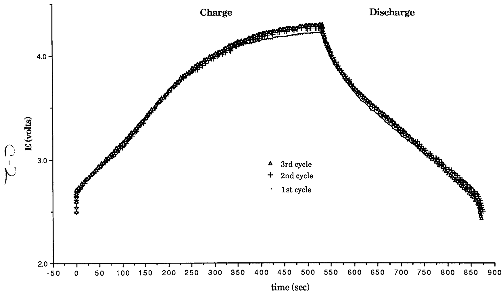
Fig. 39. Charge/Discharge Curves of Li/PPy Fibrillar Film Battery Using 3Q CV Charge.
