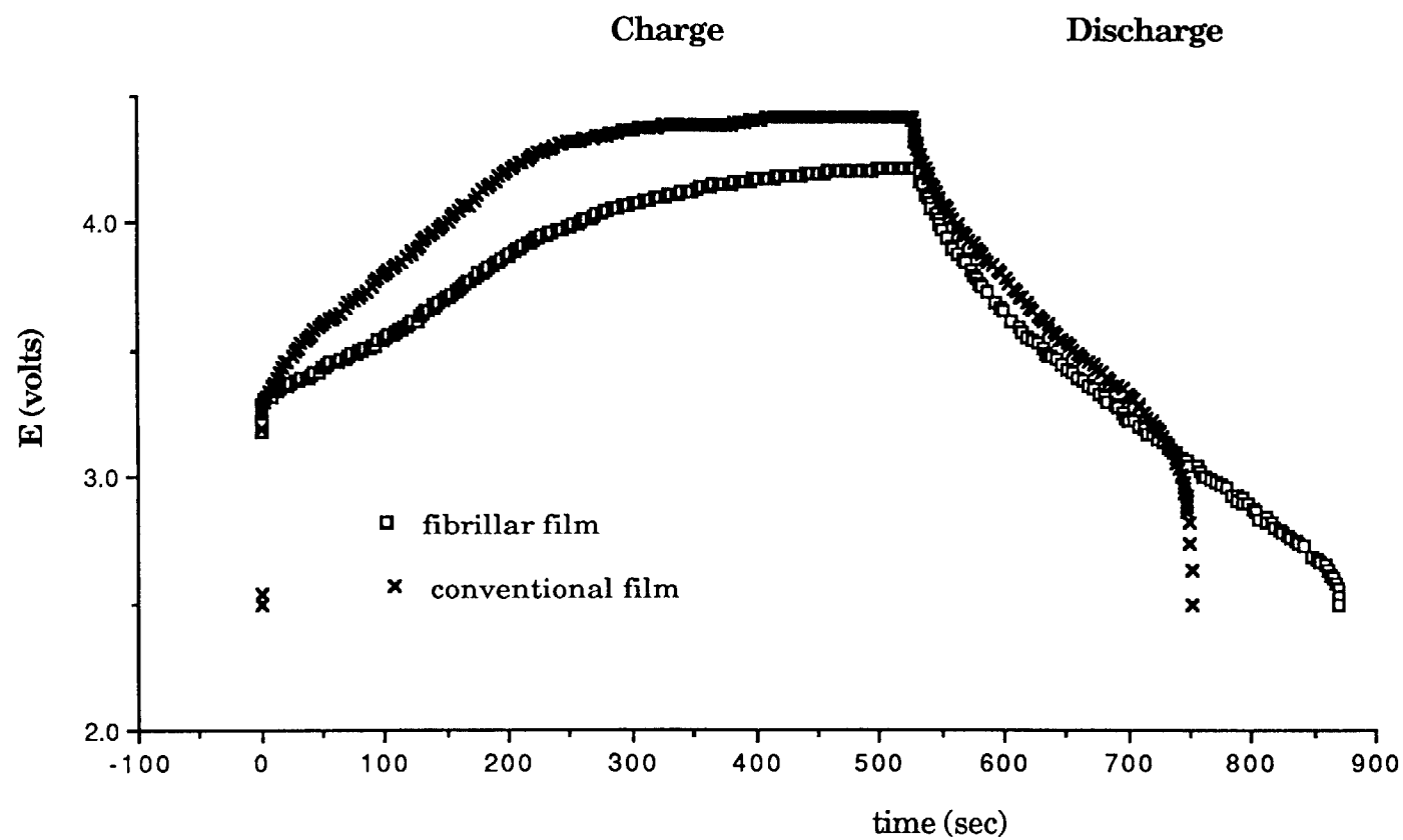
Fig. 46. Charge/Discharge Curves of Li/PPy Conventional Film Battery and Fibrillar Film Battery Using 3Q CV Charge.
