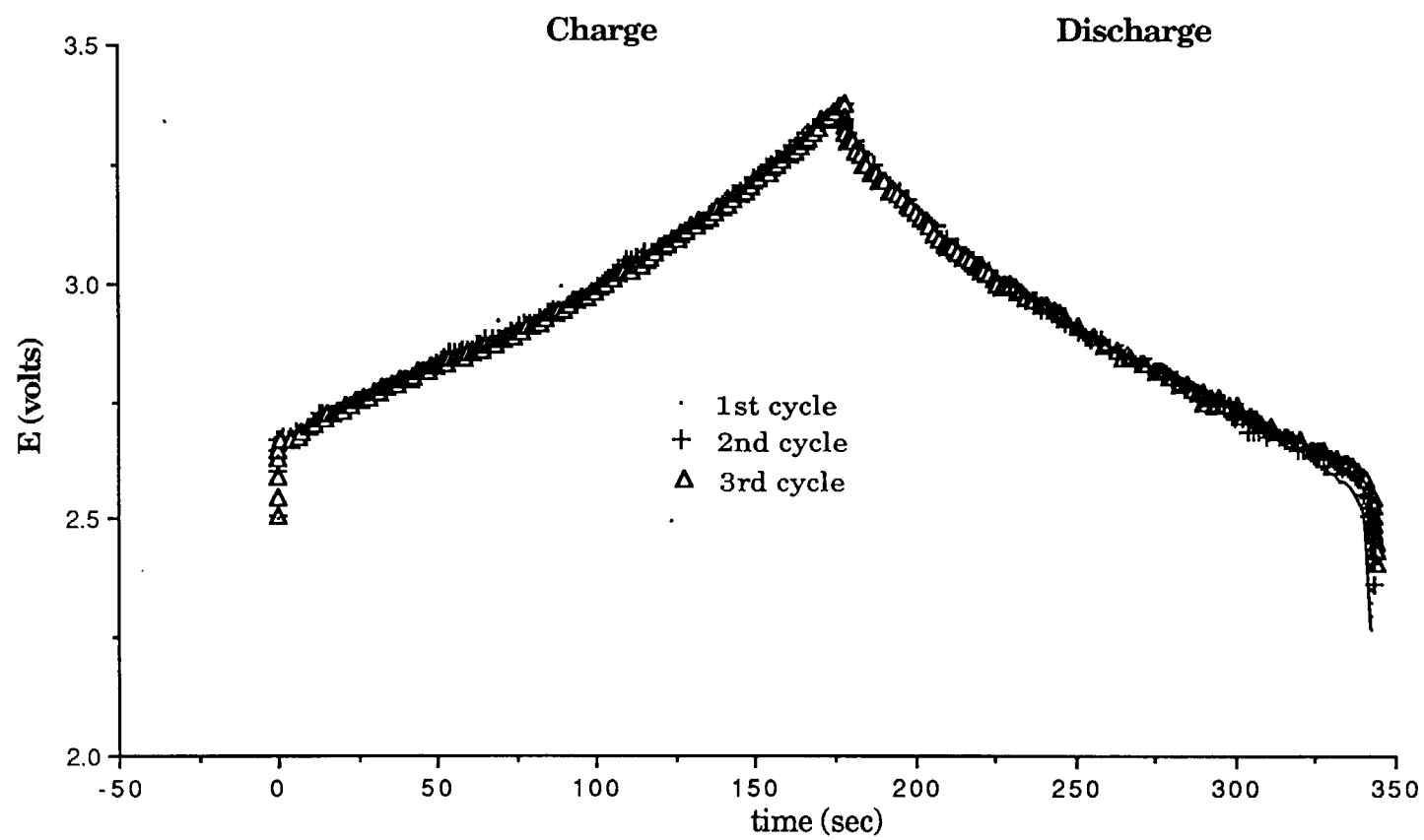
Fig. 37. Charge/Discharge Curves of Li/PPy Fibrillar Film Battery Using 1Q CV Charge. First Three Cycles.
