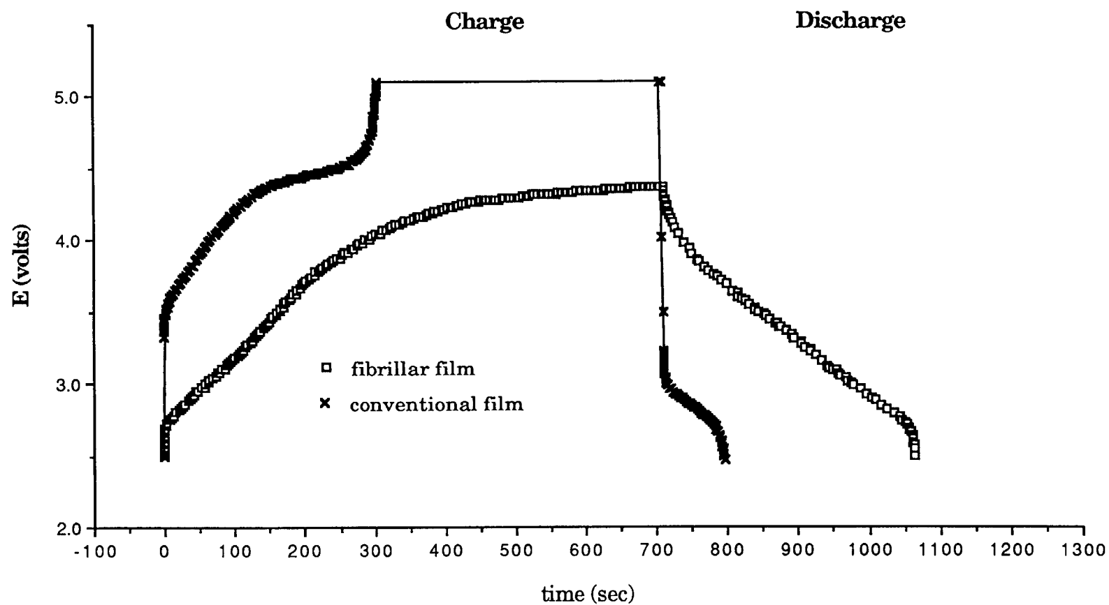
Fig. 47. Charge/Discharge Curves of Li/PPy Conventional Film Battery and Fibrillar Film Battery Using 4Q CV Charge.
