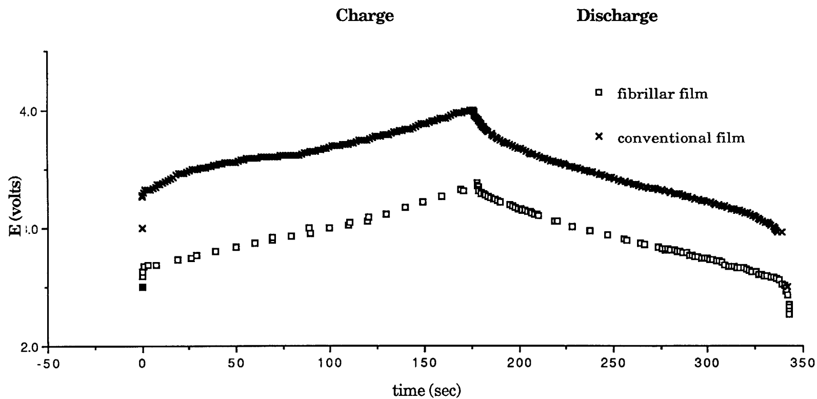
Fig. 44. Charge/Discharge Curves of Li/PPy Conventional Film Battery and Fibrillar Film Battery Using 1Q CV Charge.
