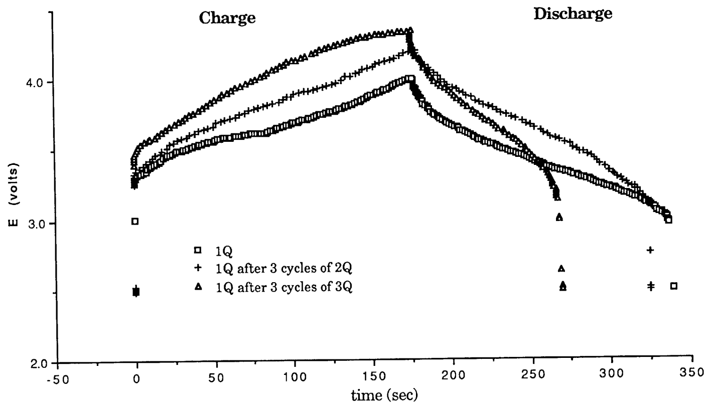
Fig. 42. Charge/Discharge Curves of Li/PPy Conventional Film Battery Using 1Q CV Charge Between 3 Cycles Each of 1Q, 2Q, 3Q, and 4Q CV Charge.
