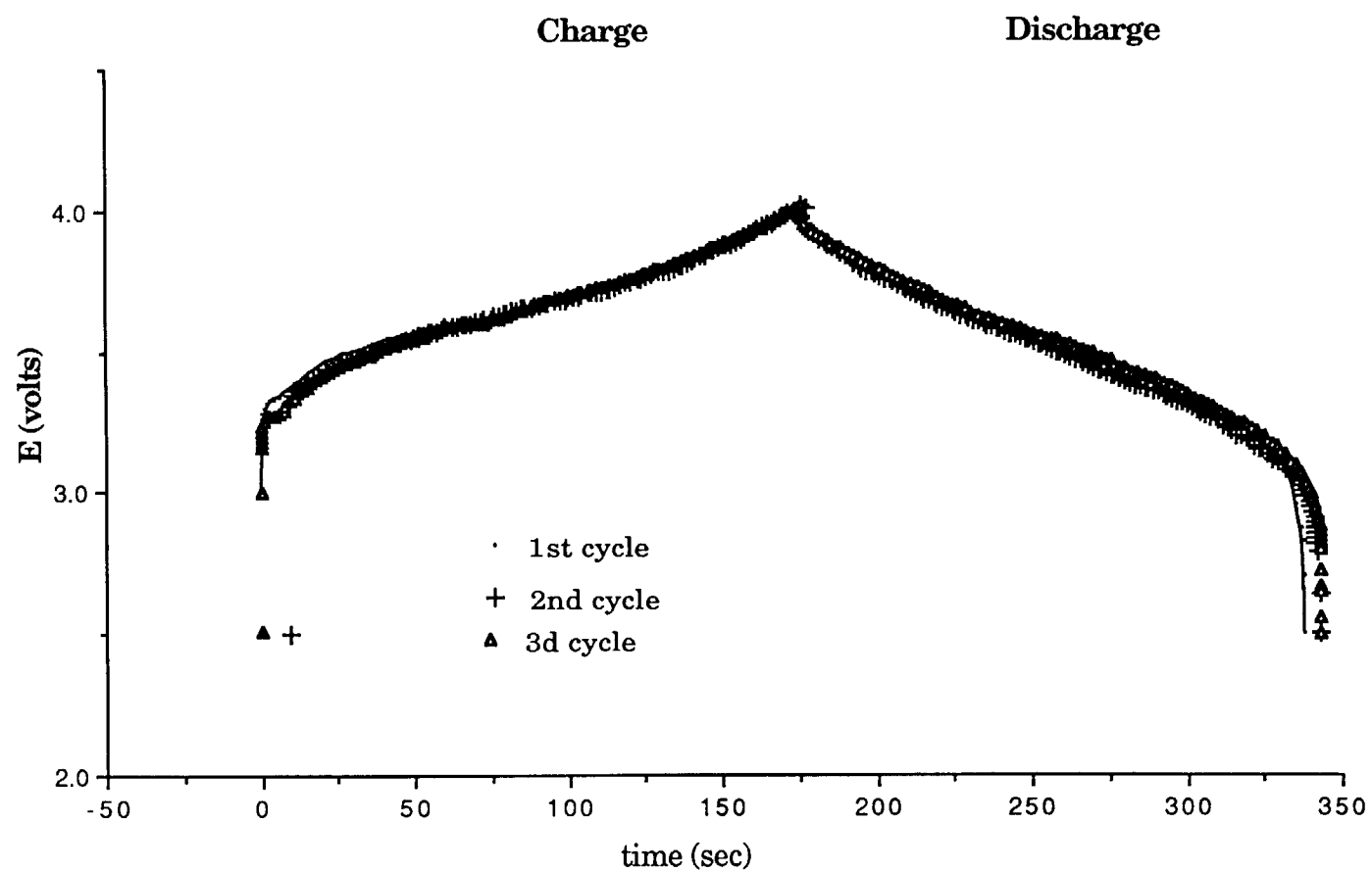
Fig. 33. Charge/Discharge Curves of Li/PPy Conventional Film Battery Using 1Q CV Charge. First Three Cycles.
