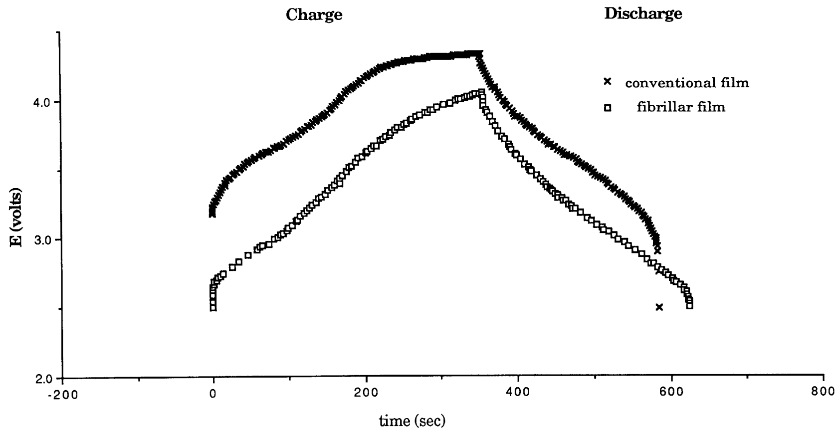
Fig. 45. Charge/Discharge Curves of Li/PPy Conventional Film Battery and Fibrillar Film Battery Using 2Q CV Charge.
