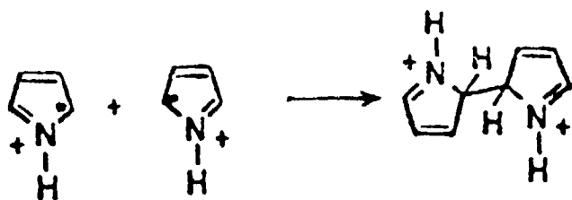
Fig. 2. Mechanism For the Electrochemical Polymerization of Pyrrole
