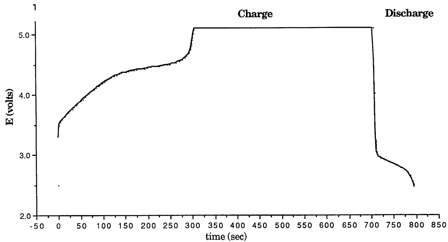
Fig. 36. Charge/Discharge Curve Of Li/PPy Conventional Film Battery Using 4Q CV Charge.
