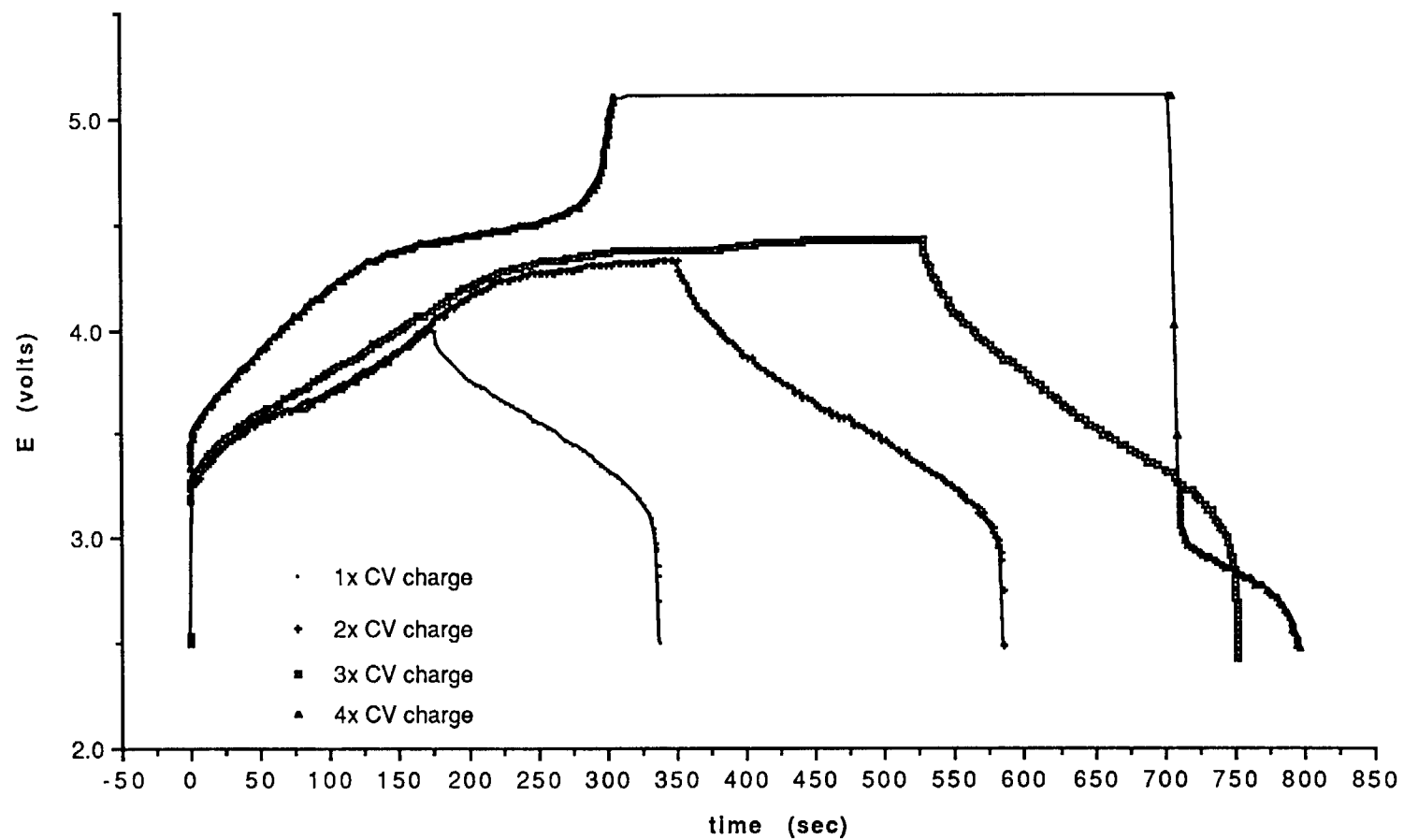
Fig. 48. Charge/Discharge Curves of Li/PPy Conventional Film Battery Using 1Q, 2Q, 3Q, and 4Q CV Charge.
