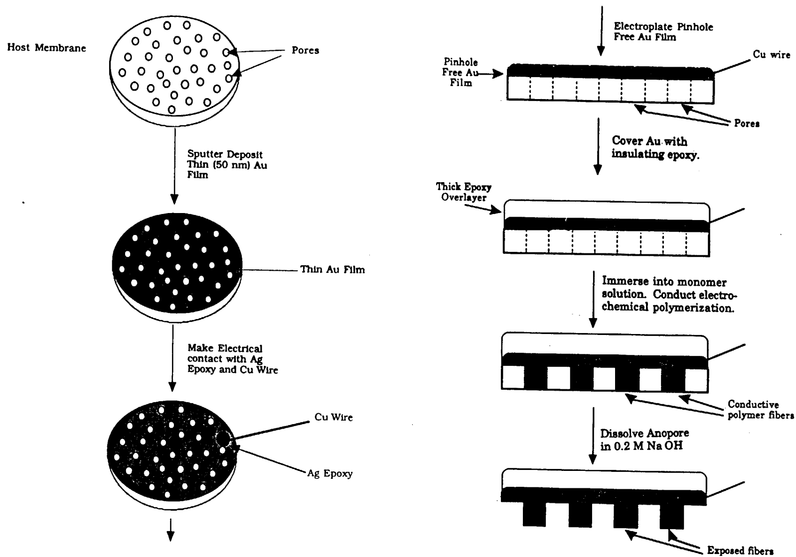
Fig. 10. Schematic of Preparation of Fibrillar Polypyrrole Electrode.
