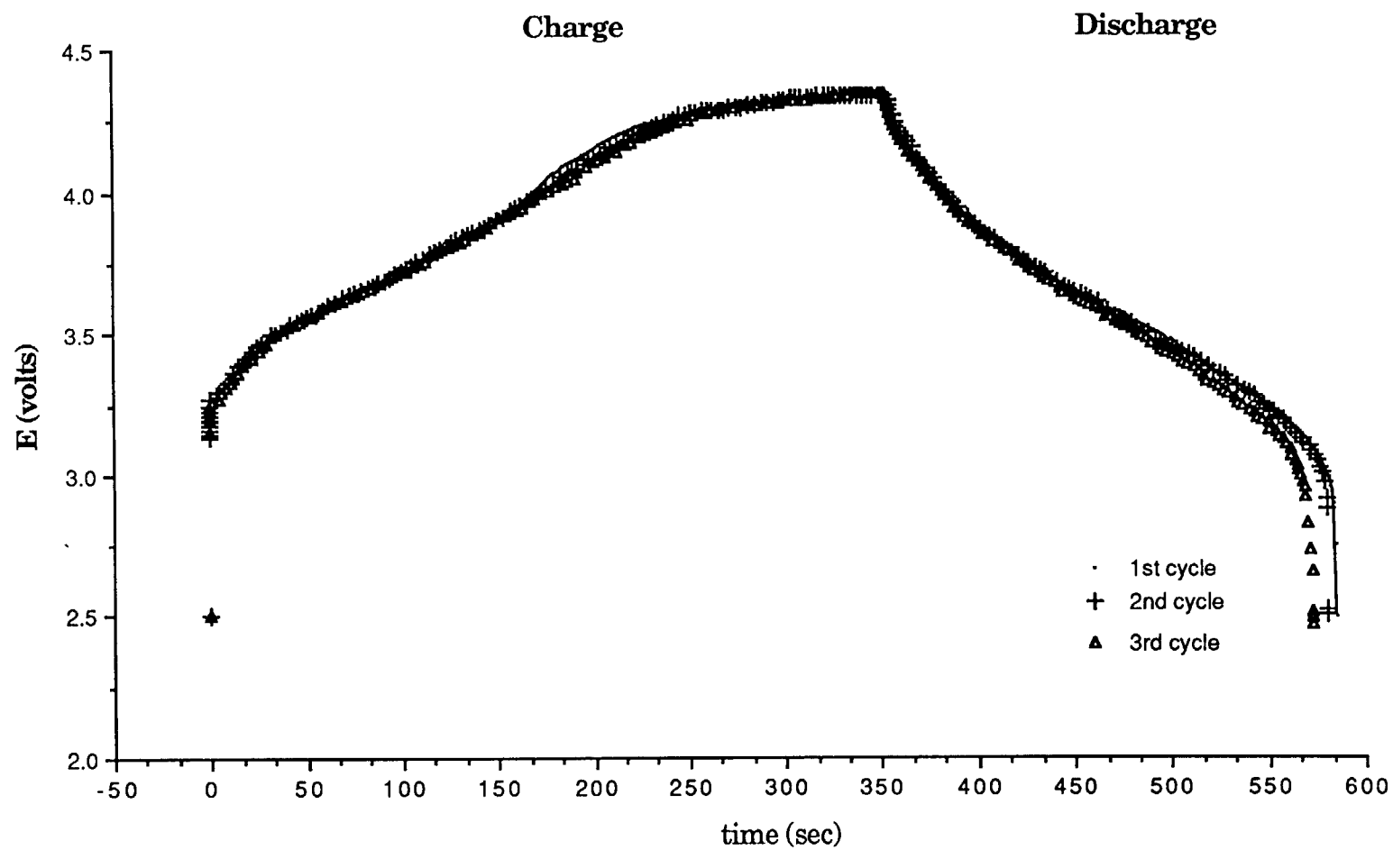
Fig. 34. Charge/Discharge Curves of Li/PPy Conventional Film Battery Using 2Q CV Charge.
