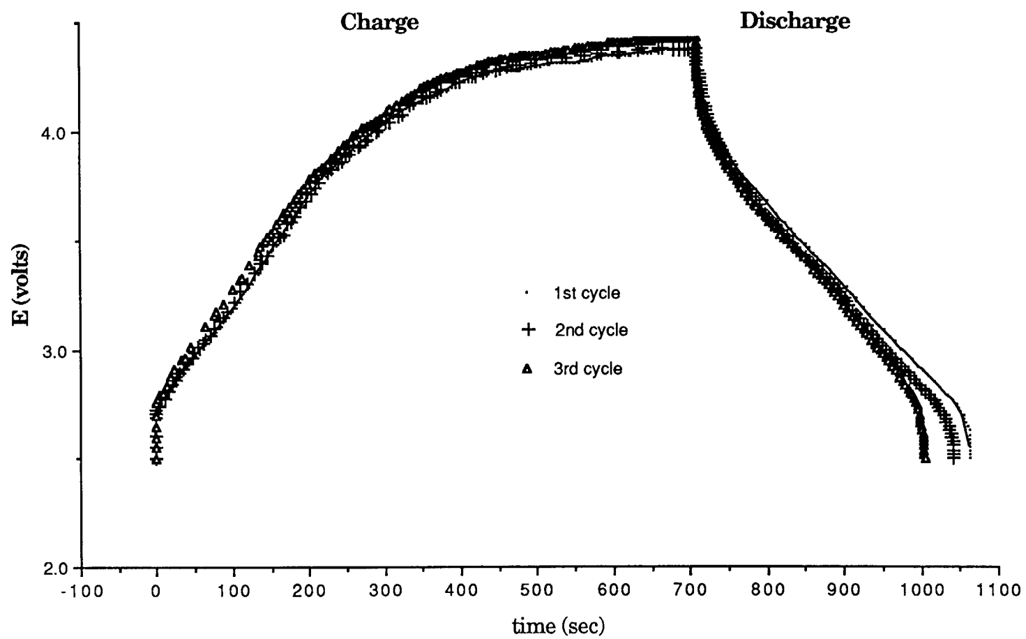
Fig. 40. Charge/Discharge Curves of Li/PPy Fibrillar Film Battery Using 4Q CV Charge.
