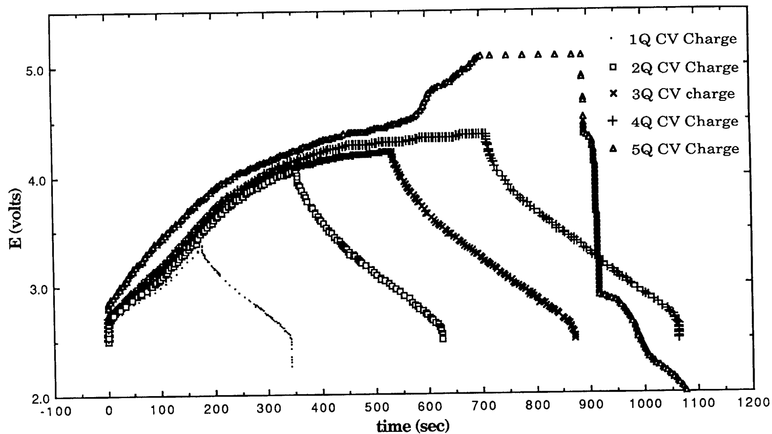
Fig. 49. Charge/Discharge Curves of Li/PPy Fibrillar Film Battery Using 1Q, 2Q, 3Q, 4Q, & 5Q CV Charge.
