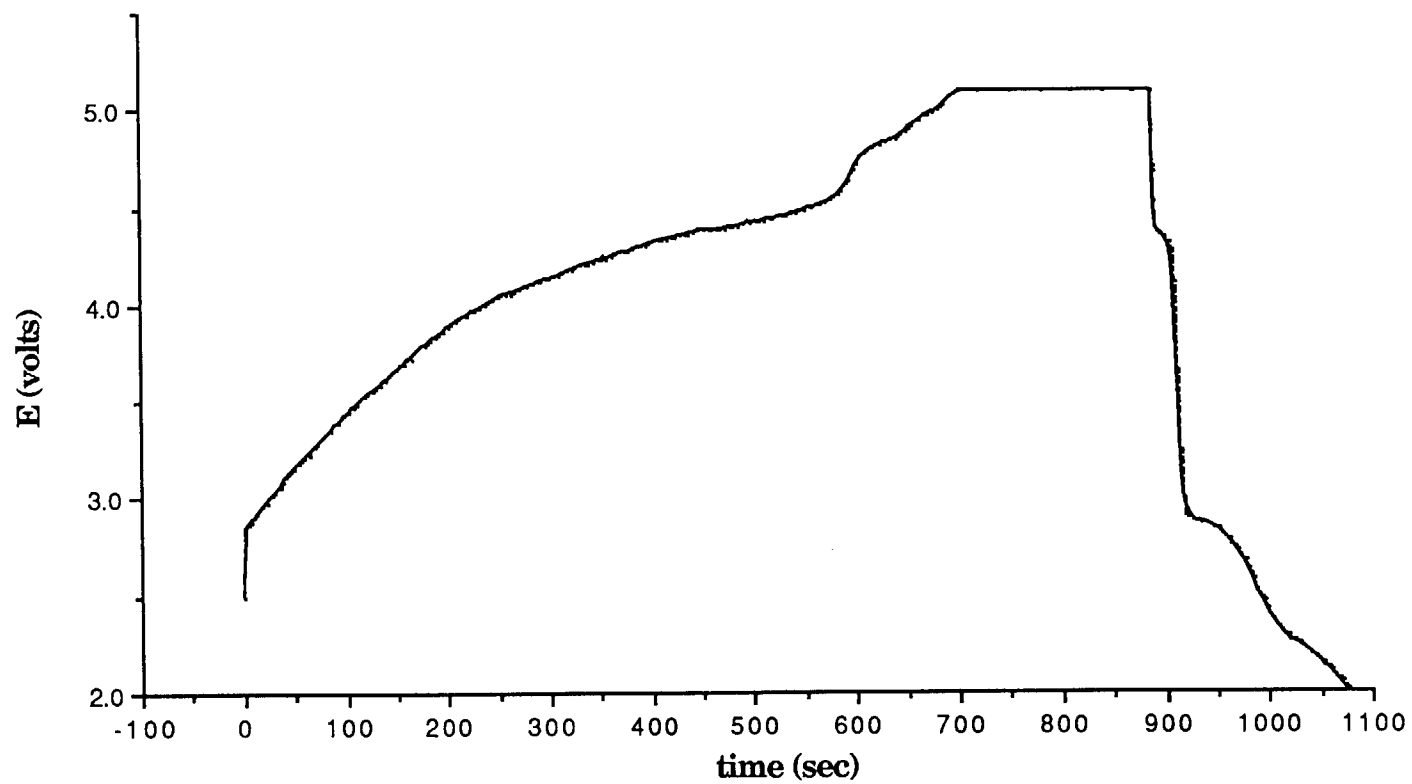
Fig. 41. Charge/Discharge Curve of Li/PPy Fibrillar Film Battery Using 5Q CV Charge.
