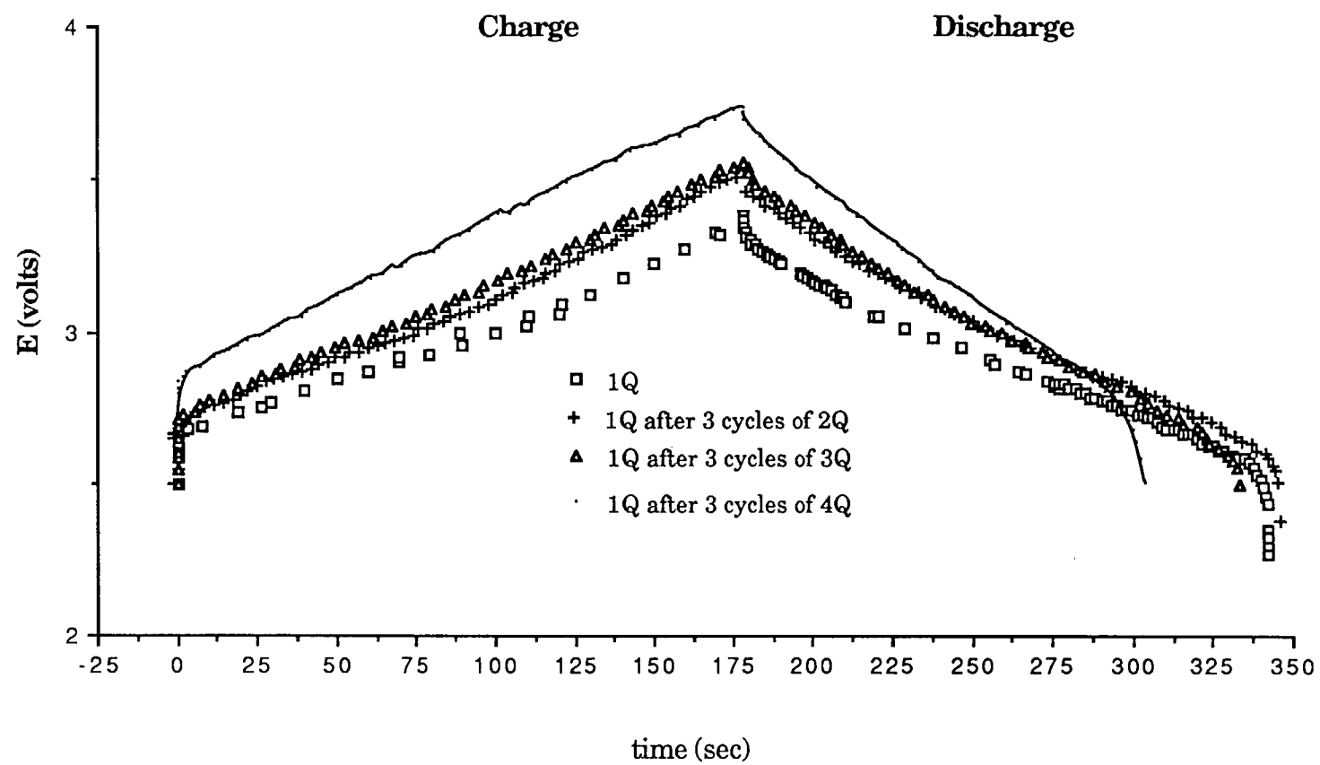
Fig. 43. Charge/Discharge Curves of Li/PPy Fibrillar Film Battery Using 1Q CV Charge Between 3 Cycles Each of 1Q, 2Q, 3Q, and 4Q CV Charge.
