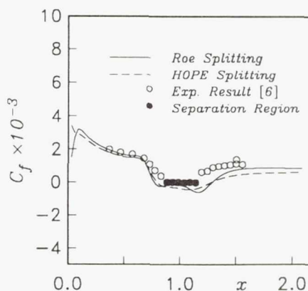
Fig. 8. Friction Coefficient at the Wall.
