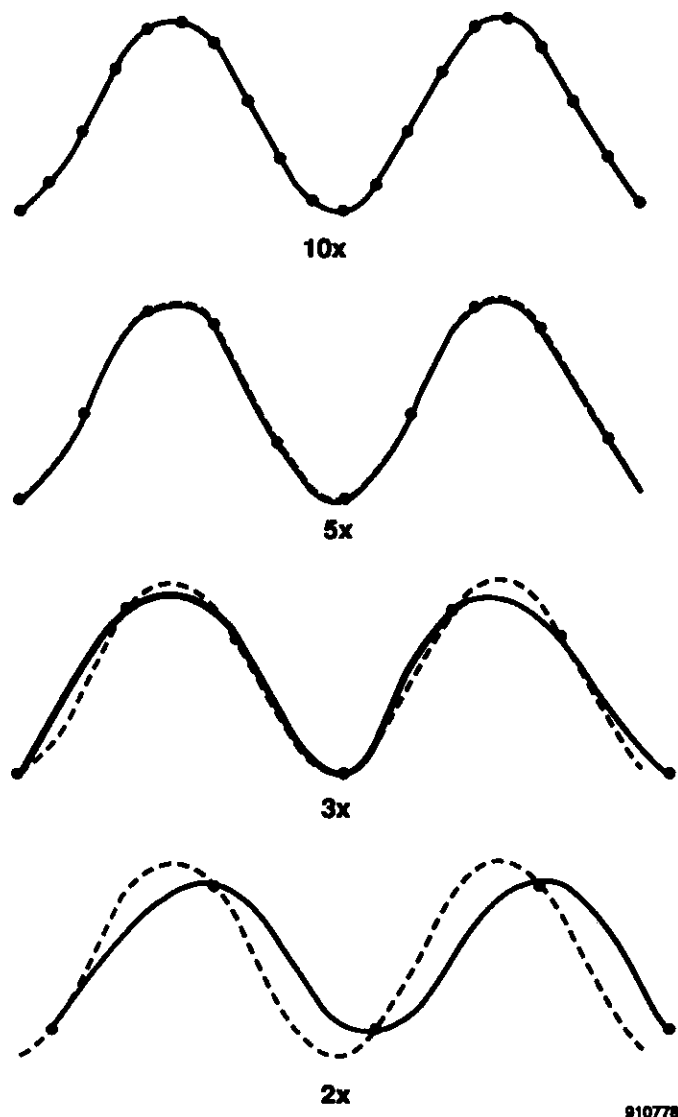
Figure 3-9. Comparison of different sampling rates.
