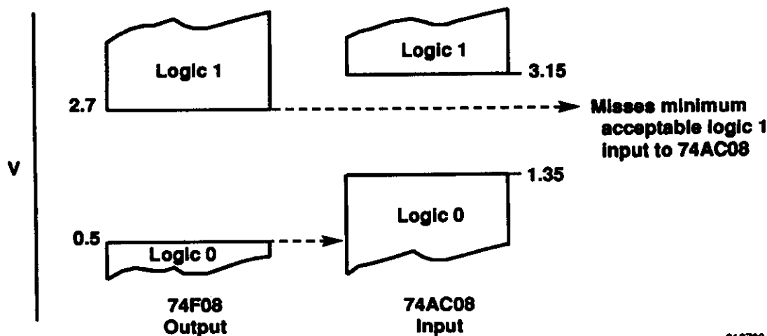
Figure 2-3. Logic family interfacing problem.
