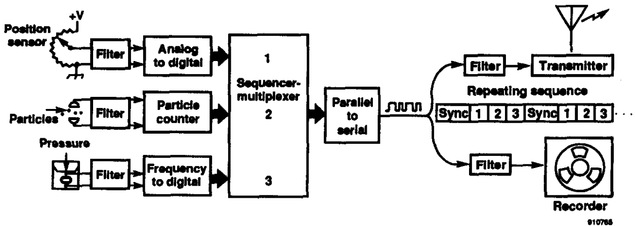
Figure 1-2. Simplified aircraft data acquisition system.
