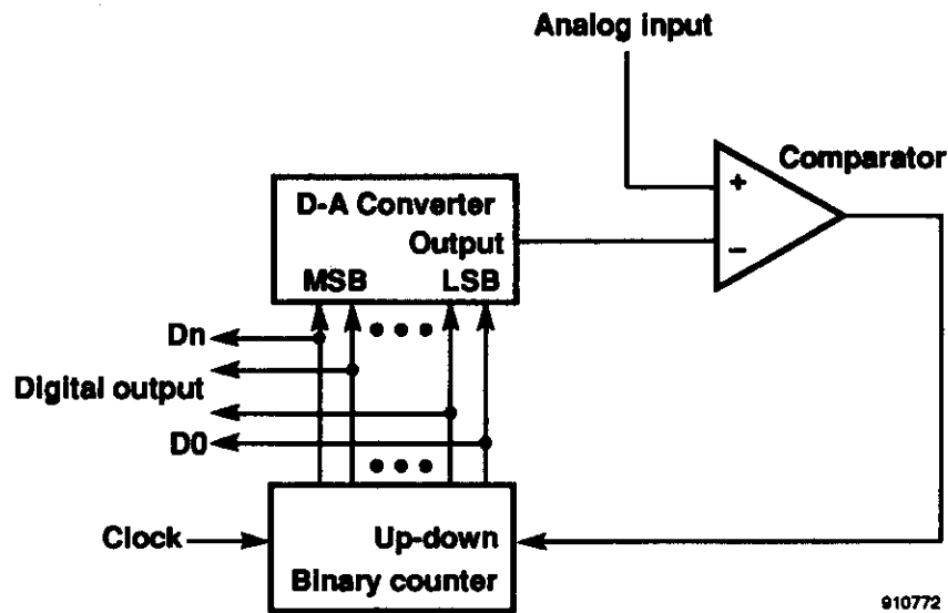
Figure 3-3. Tracking analog-to-digital converter.
