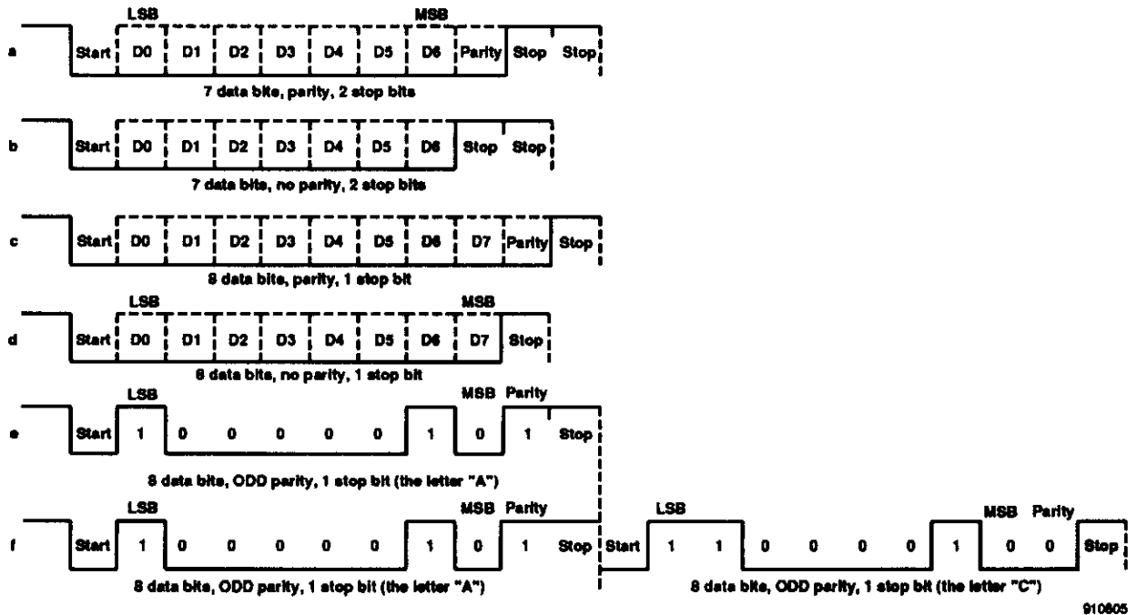
Figure 6-17. Examples of bit-sequential ASCII.
