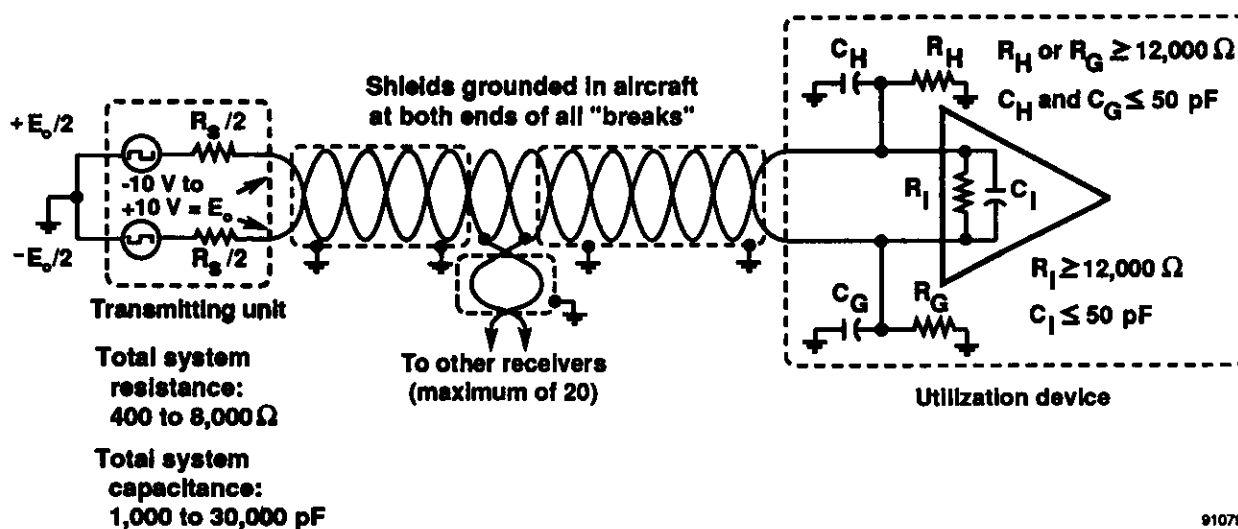
Figure 6-11. The ARINC 429 input-output circuit standards.
