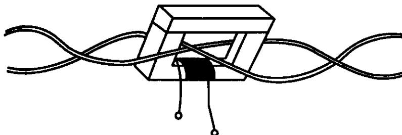
Figure 6-12. The ARINC 629 (DATAC) bus coupling.
