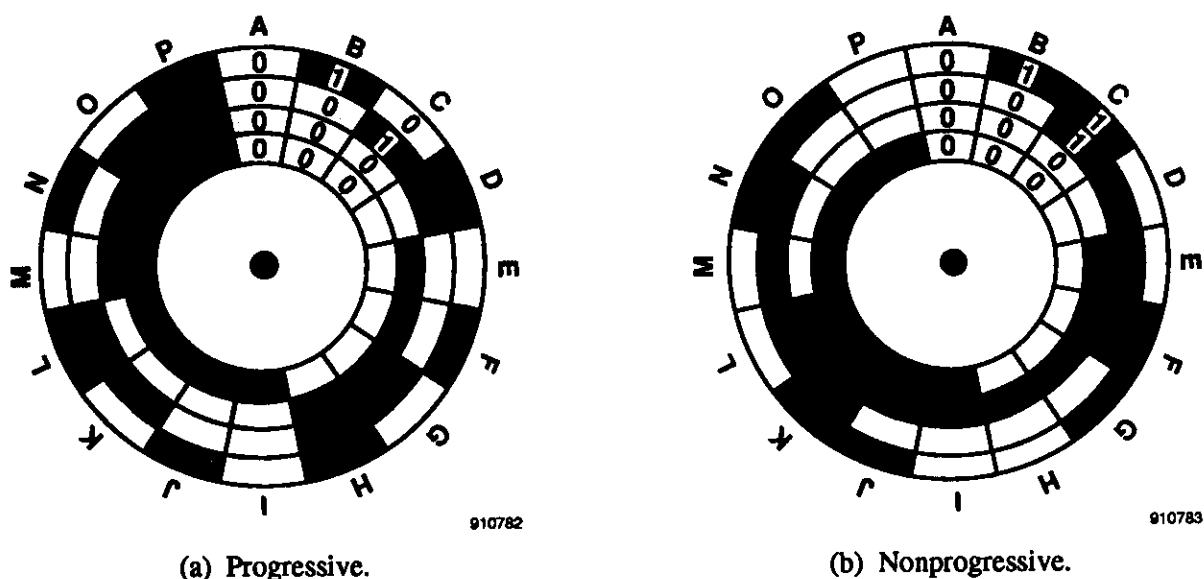
Figure 4-1. Encoded disks.
