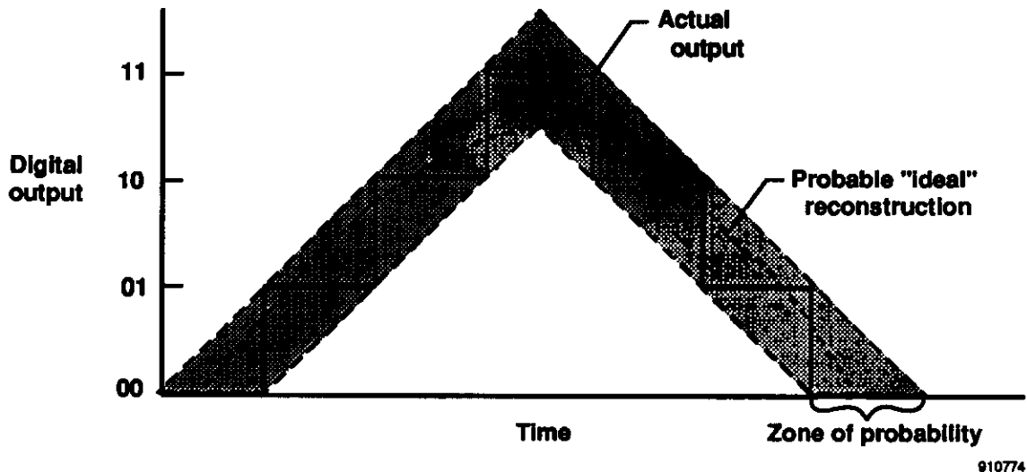
Figure 3-5. Digital-to-analog conversion.
