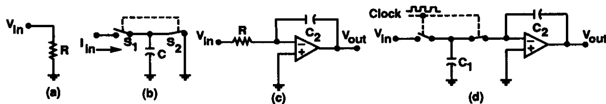
Figure 5-2. Representation of a switched capacitor as a resistor.
