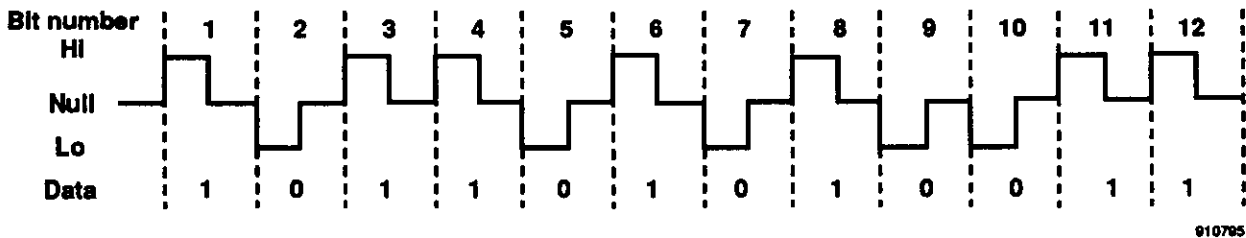
Figure 6-7. Bipolar RZ coding.
