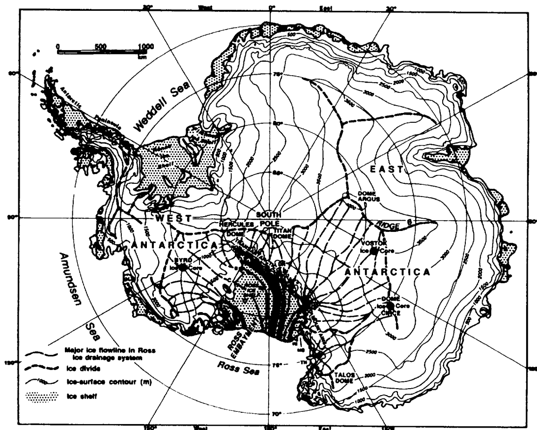
FIG. 1. Index map of Antarctica. Flowlines shown only for the Ross ice drainage system, which is defined as the portion of the Antarctic Ice Sheet that flows into the Ross Embayment. A, B, C, D, and E are West Antarctic ice streams. RG, Reedy Glacier; BG, Beardmore Glacier; DR, Dominion Range ice cap; HG, Hatherton Glacier; DG, Darwin Glacier; DV, Dry Valleys; RI, Ross Island; MS, McMurdo Sound; and TN, Terra Nova Bay. Adapted from Drewry (1983).
