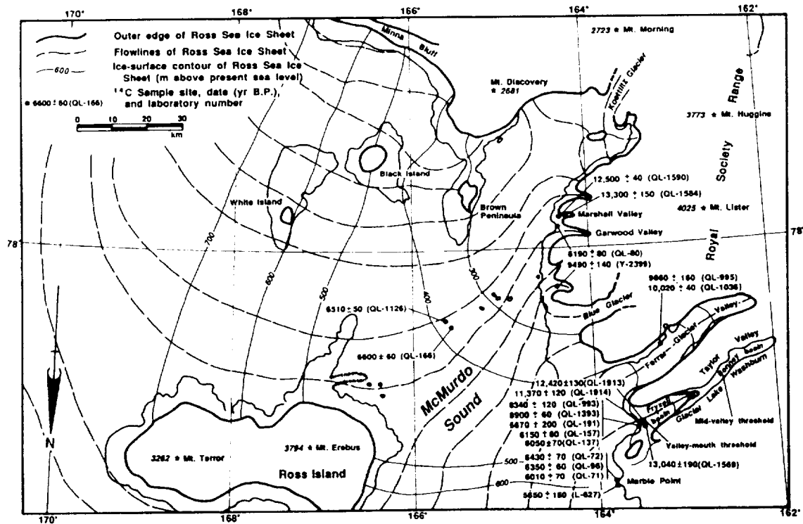
FIG. 5. Surface contours and flowlines of the grounded ice sheet that deposited Ross Sea drift in McMurdo Sound during late Wisconsin (stage 2) time. Adapted from Stuiver et al. (1981, Figs. 7–16).
