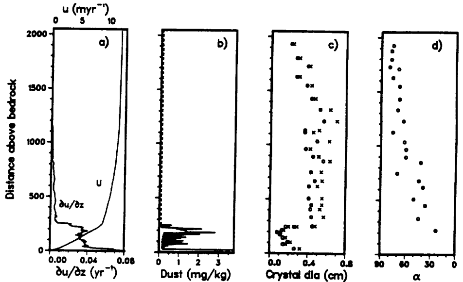
FIG. 2 (a) Profiles of horizontal velocities and shear strain rate derived from the inclinometer surveys of the Dye 3 borehole (Fig. 2a). The \partial u/\partial z profile can be divided into three zones: the bottom 25 m of silty ice with very high deformation rates; the immediately overlying 230 m of ice, deposited during the last glaciation; and the uppermost 1780 m of Holocene ice, with lower deformation rates. (b) Dust concentration, the bulk concentration of insoluble microparticles in the ice. (Hammer et al., 1985). In the silty ice the dust concentration is > 20 mg/kg. (c) Crystal diameter (Herron et al., 1985). The circles represent vertical dimensions and the x's represent the horizontal dimensions. (d) Fabric parameter \alpha , the half-apex angles of the cones containing 90% of the c-axis (Herron et al., 1985).
