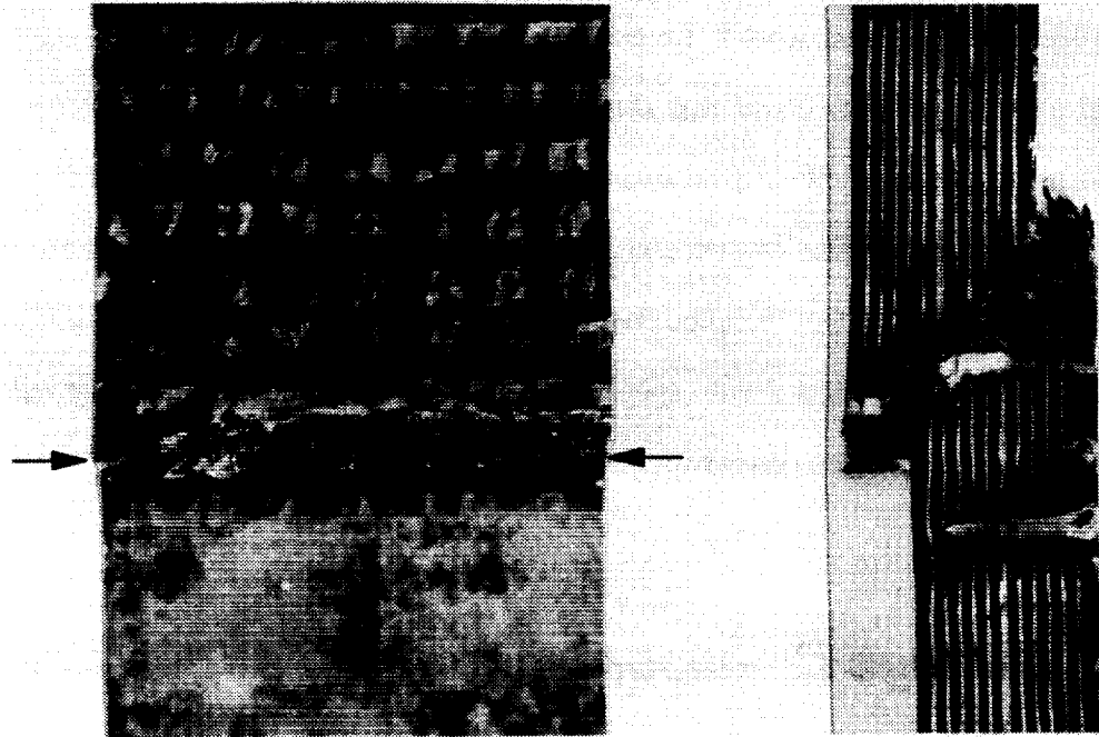
Figure 25. Fatigue Failure Patterns with Surface Damage Marked by Arrows (90° Specimens)
