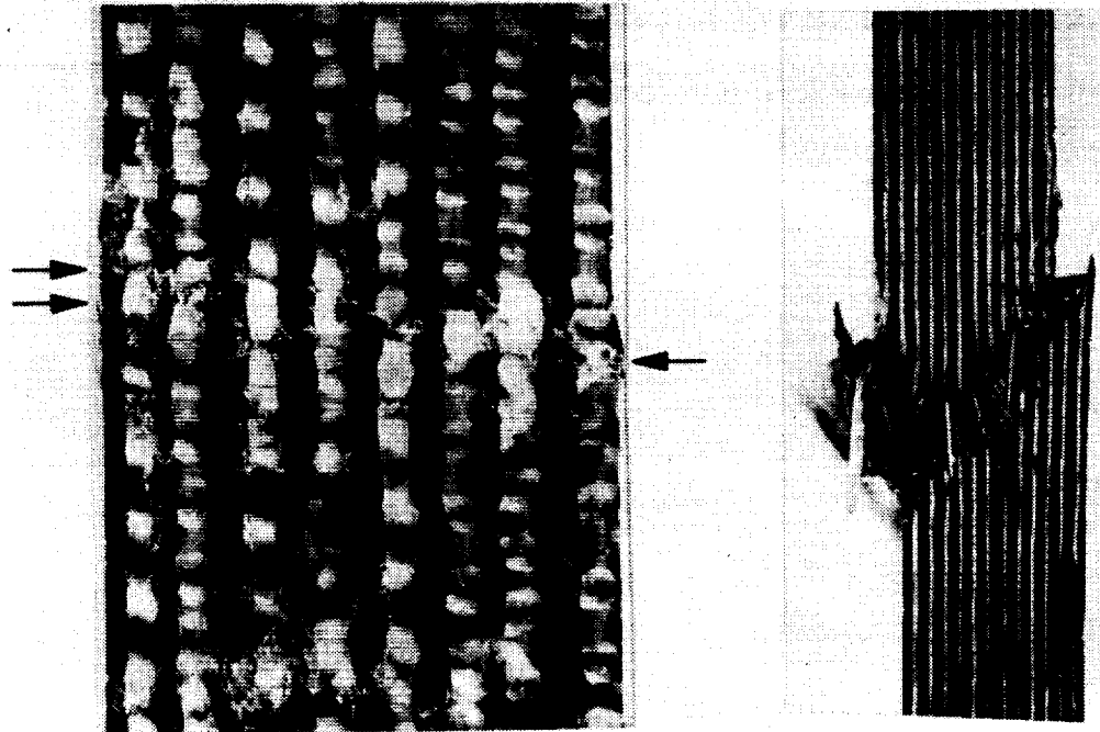
Figure 24. Fatigue Failure Patterns with Surface Damage Marked by Arrows (0° Specimens)
