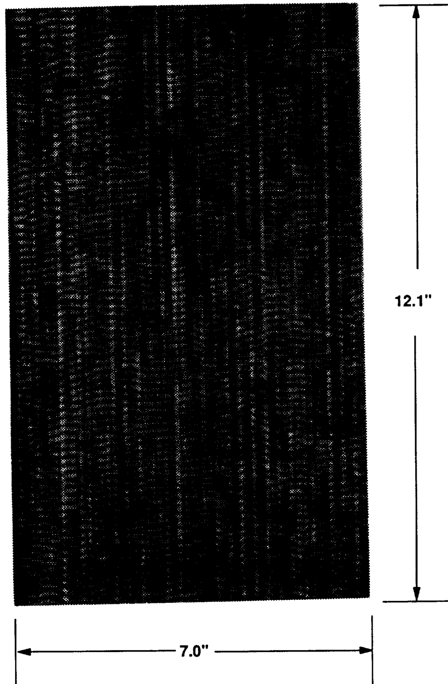
Figure 17. Ultrasonic C-Scan of Plate M
