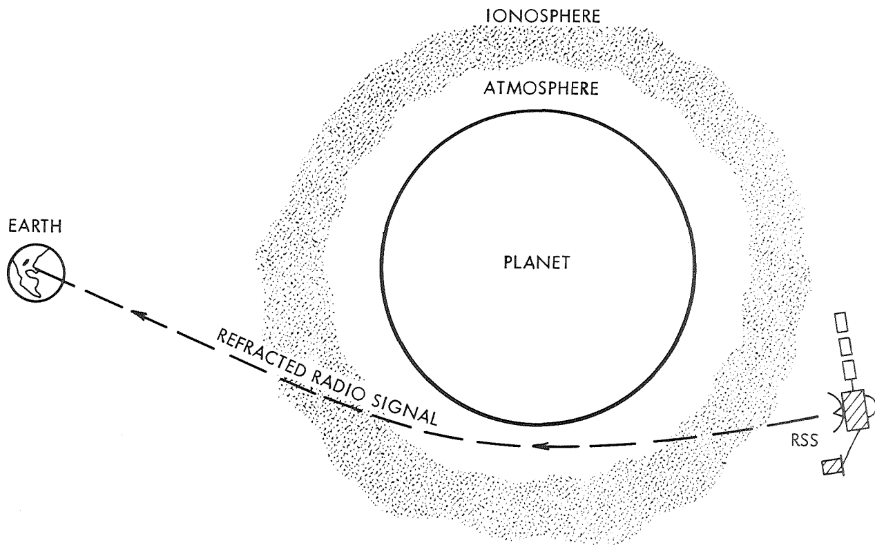
Figure 4-4. The Radio Science Subsystem uses the spacecraft radio transmitter to beam a signal through the ionosphere and neutral atmosphere for detection by the DSN antennas on Earth. The signal changes allow an estimate of the density, temperature, and pressure of the atmosphere.
