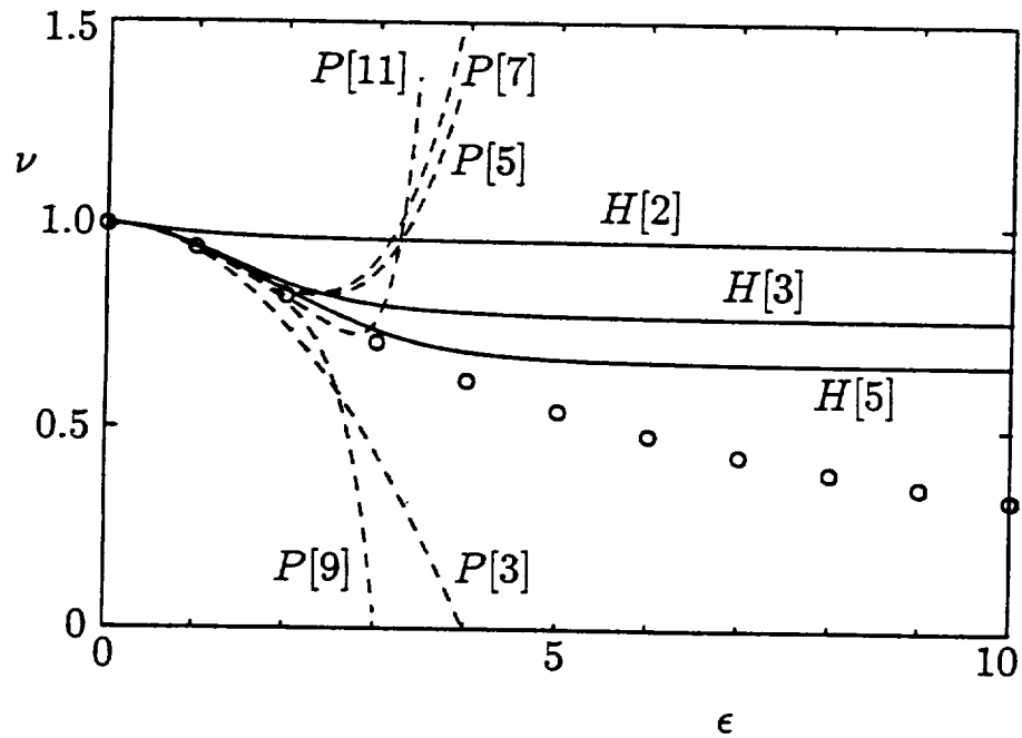
FIG 6. Comparison of hybrid (solid lines) frequency computations for the limit cycle of the van der Pol oscillator with perturbation (dashed lines) and numerical (circles) computations for a range of \epsilon values.
