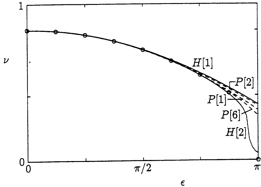
FIG 3. Comparison of hybrid (solid lines) frequency computations for the simple pendulum with perturbation (dashed lines) and numerical (circles) computations. The amplitude ranges from 0 to \pi .
