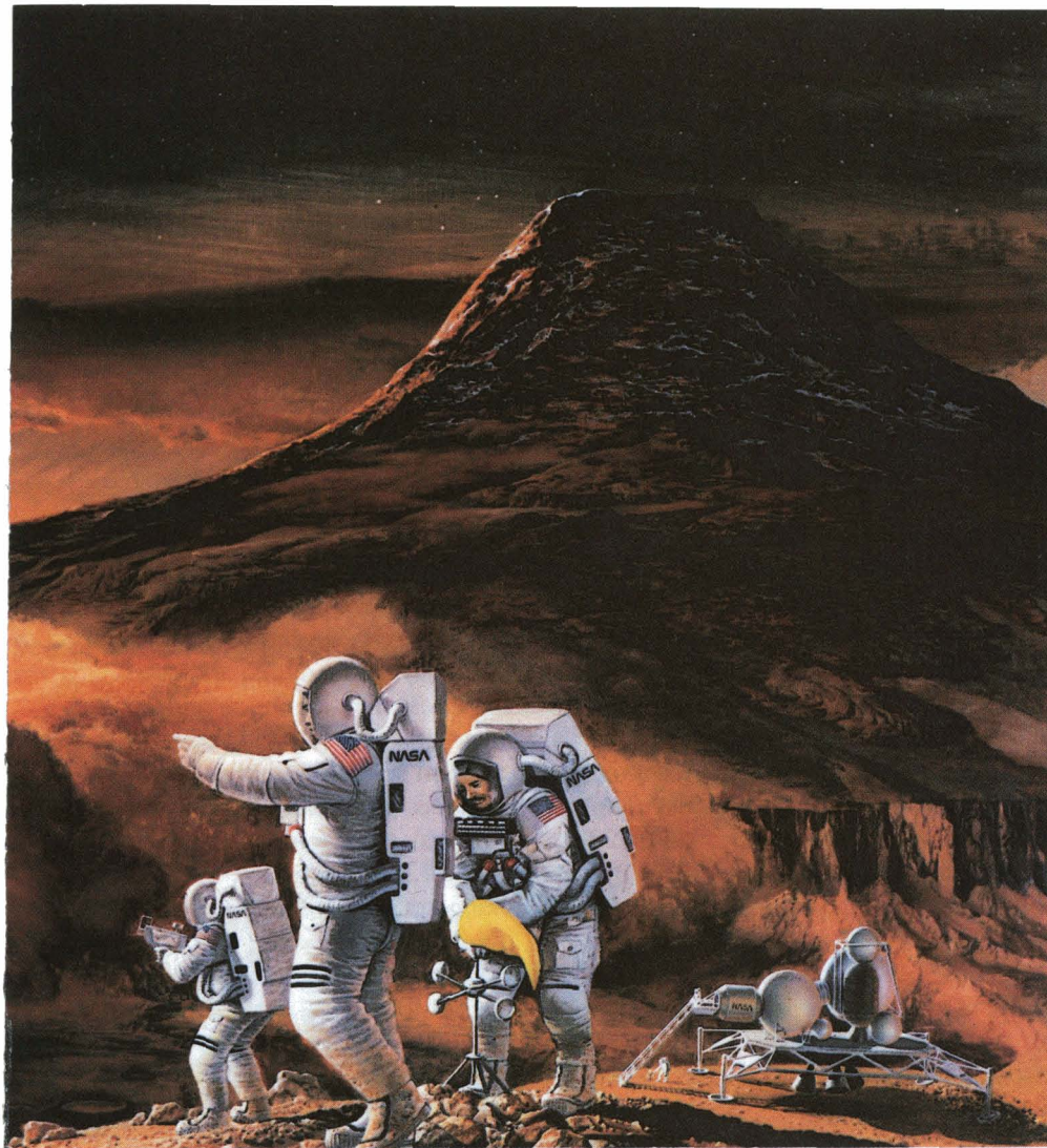
An artist's conception of the first human landing on Mars, circa 2019 in the vicinity of the mountain Olympus Mons. In the foreground, astronauts are conducting scientific observations and recording planetary features with a hand-held camera. In the background at right is the excursion vehicle in which the explorers descended to the surface from a much larger interplanetary transfer vehicle.
