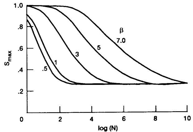
Figure 10.—Illustration of the effect on the S-N curve of varying the parameter \beta = 0.5, 1.0, 3.0, 5.0 and 7.0 , while holding all other parameters fixed.
