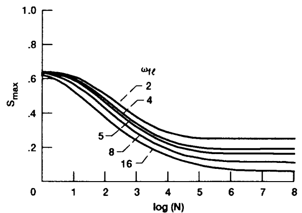
Figure 14.—Illustration of the effect on the S-N curve of varying the ratio \omega_L = 2, 4, 5, 8 , and 16 , at an angle of 15 degrees, while holding all other parameters fixed at the baseline values.
