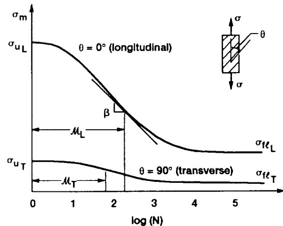
Figure 28.—A schematic depicting the expected S-N curves for a unidirectional metallic composite, when loaded longitudinally ( \theta = 0.0 ) and transversely ( \theta = 90 ).
