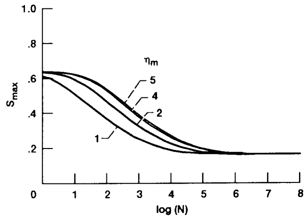
Figure 20.—Illustration of the effect on the S-N curve of varying the ratio \eta_m = 1, 2, 4 , and 5, at an angle of 15 degrees, while holding all other parameters fixed at the baseline values.
