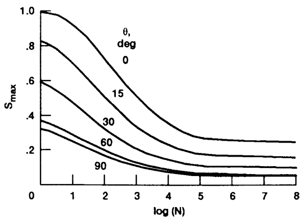
Figure 15.—Illustration of the effect on the S-N curve of varying the angle of fiber orientation \theta = 0, 15, 30, 60 , and 90 degrees with the ratio \omega_U = 3 and all other parameters fixed at the baseline values.
