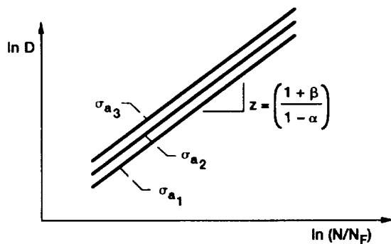
Figure 27.—A log-log plot of damage ( D ) versus remaining life ( N/N_F ) for various stress amplitudes.
