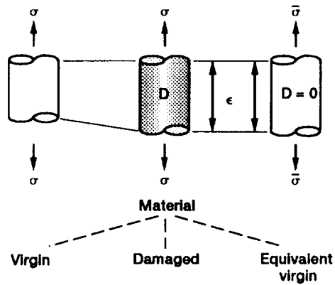
Figure 1.—Schematic of effective stress concept and equivalence in strain.
