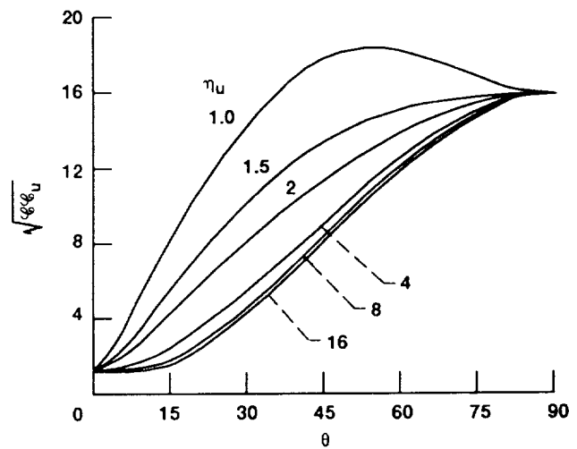
Figure 22.—Variation of \mathcal{K}_U with angle of orientation \theta , for varying ratios of \eta_U , i.e., 1.0, 1.5, 2.0, 4.0, 8.0, and 16.0, when \omega_U = 16.0 and all other parameters are those in table V.
