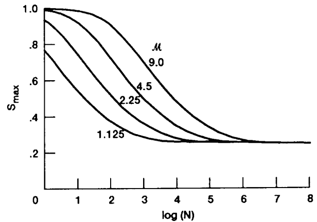
Figure 8.—Illustration of the effect on the S-N curve of varying the parameter M = 1.125, 2.25, 4.5, 9.0 , while holding all other parameters fixed.
