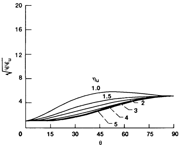
Figure 21.—Variation of \mathcal{K}_U with angle of orientation \theta , for varying ratios of \eta_U , i.e., 1.0, 1.5, 2.0, 3.0, 4.0, and 5.0, when \omega_U = 5.0 and all other parameters are those in table V.
