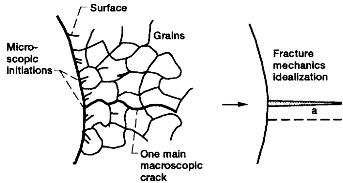
(b) Fatigue damage: nucleation of slip bands, microcracks and transgranular defects.
