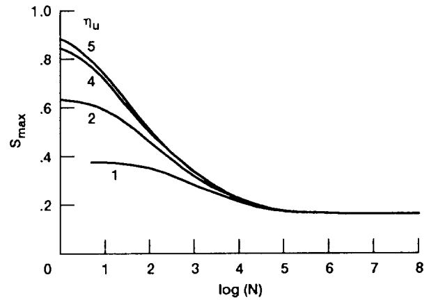
Figure 18.—Illustration of the effect on the S-N curve of varying the ratio \eta_U = 1, 2, 4 , and 5, at an angle of 15 degrees, while holding all other parameters fixed at the baseline values.
