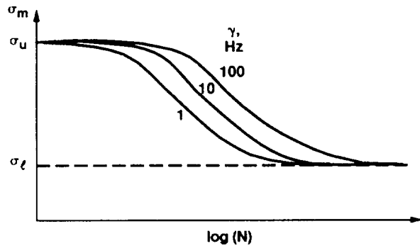
Figure 23.—Schematic of typical S-N curve for an isotropic metallic material, assumed to be known experimentally. Assuming R = \sigma_{\min}/\sigma_{\max} and the mean stress \bar{\sigma} to be held constant.
