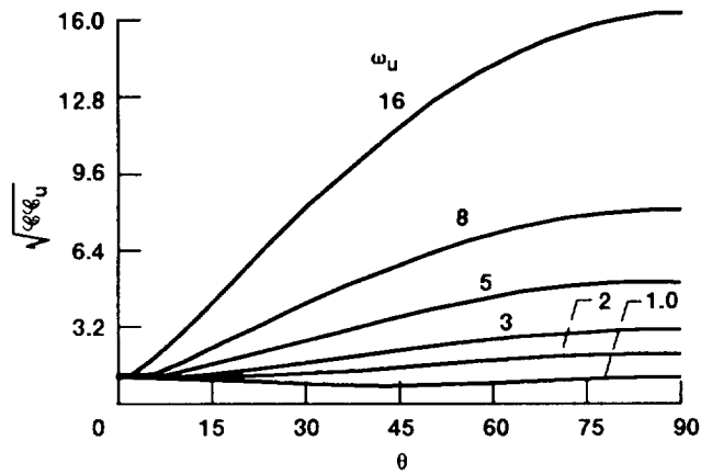
Figure 17.—Shows \mathcal{K}_U versus angle of orientation \theta , for varying ratios of \omega_U , i.e., 1.0, 2.0, 3.0, 5.0, 8.0, and 16.0, when \eta_U = 2.0 and all other parameters are those in table V.
