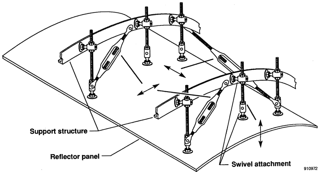
Fig. 4: Heater reflector panel attachment
