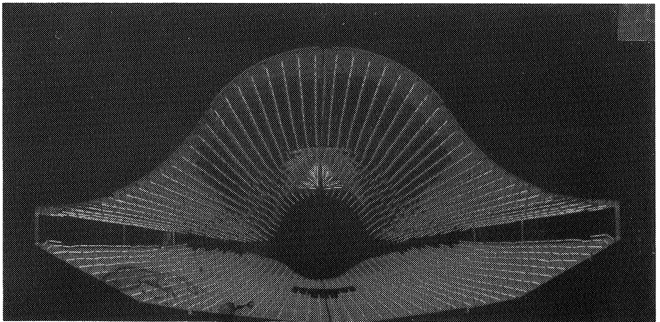
Fig. 3: Polished stainless-steel reflectors for YF-12 forebody test
