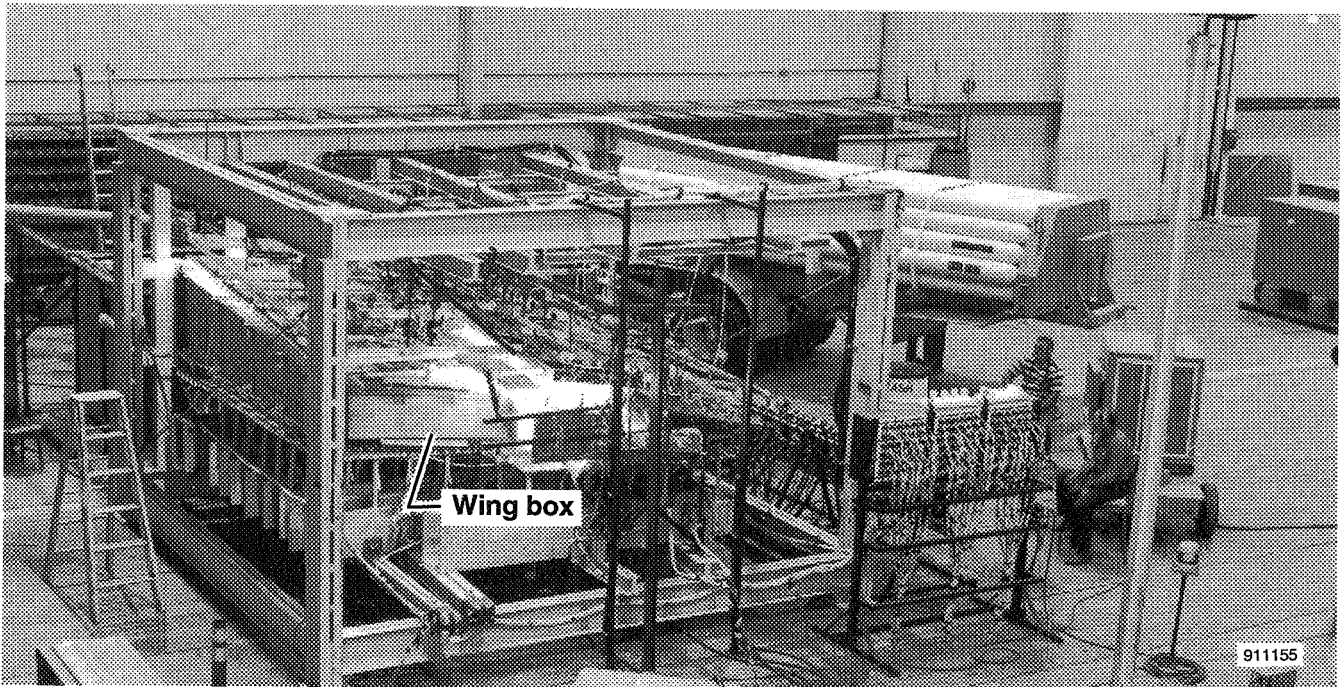
Fig. 29: Shuttle wing—elevon combined heating and loading test
