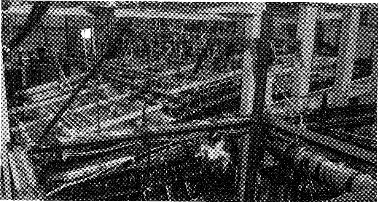
Fig. 28: Shuttle wing—elevon heating system
