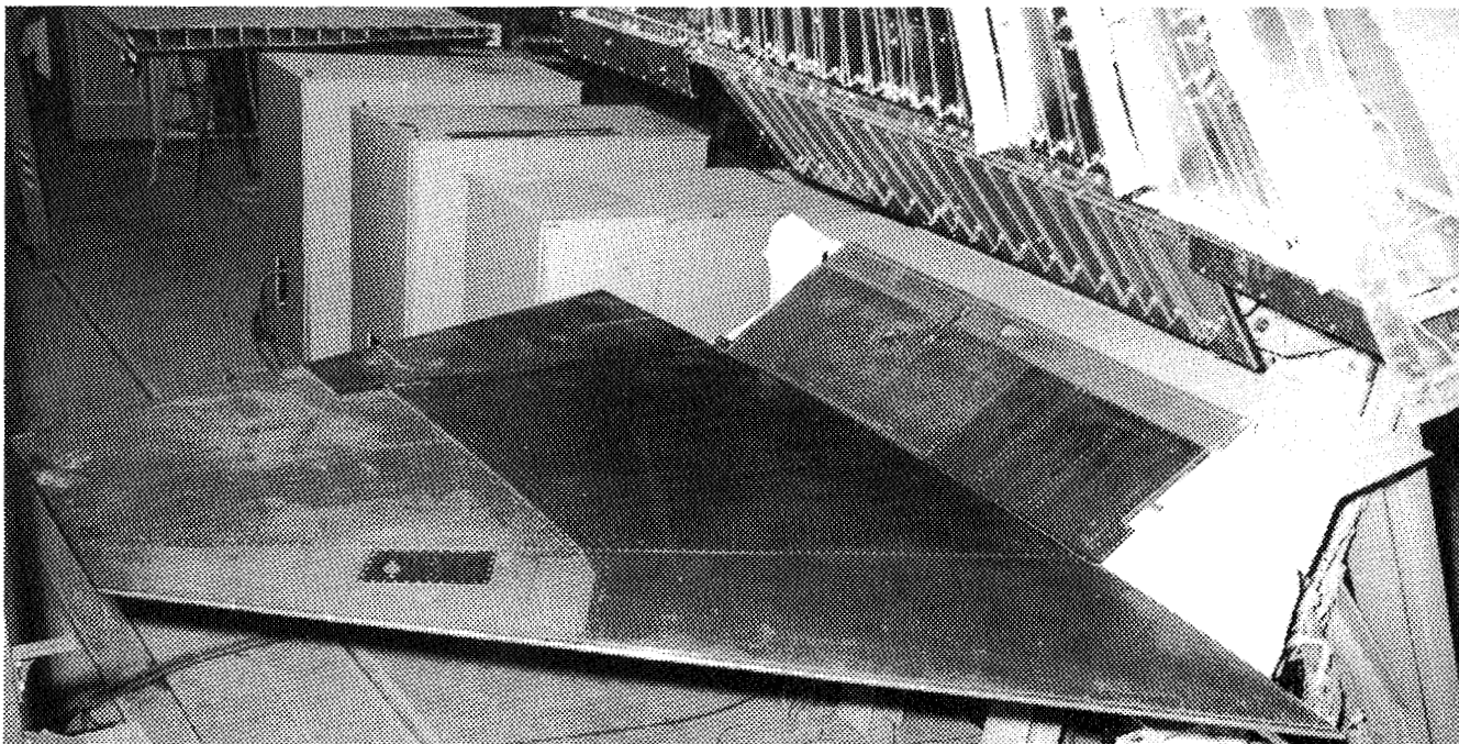
Fig. 20: X-15 wing as removed from aircraft
