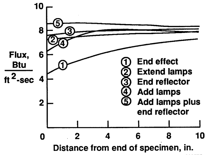
Fig. 16: Infrared heater end effects
