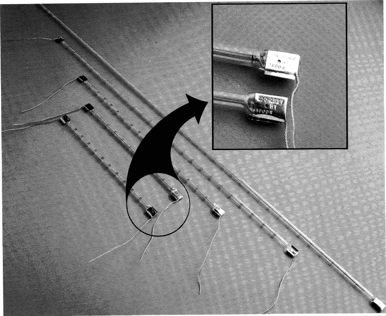
Fig. 1: Typical infrared quartz lamps
