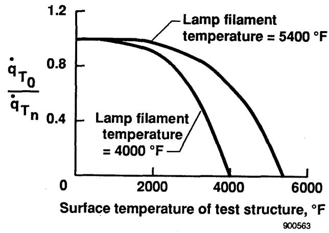
Fig. 14: Ratio of radiant heat flux
