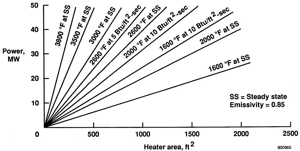
Fig. 17: Power required as a function of heater area
