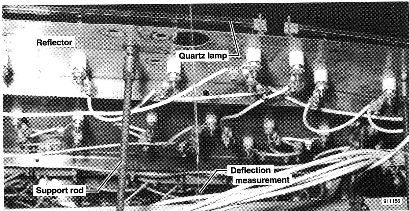
Fig. 5: Close up view of backside of stainless-steel reflector
