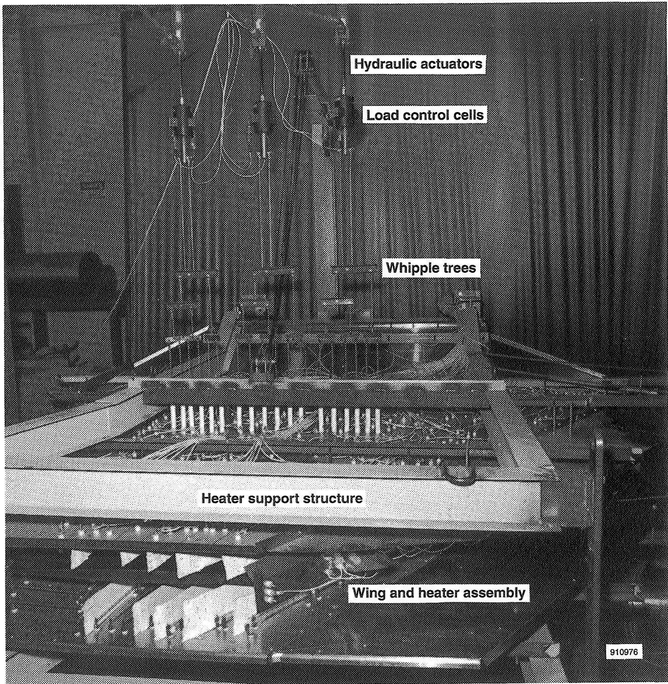
Fig. 25: Combined heating and loading test setup
