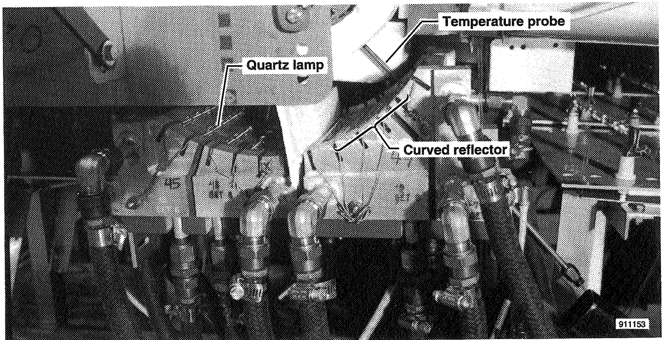
Fig. 9: Curved water cooled aluminum reflector
