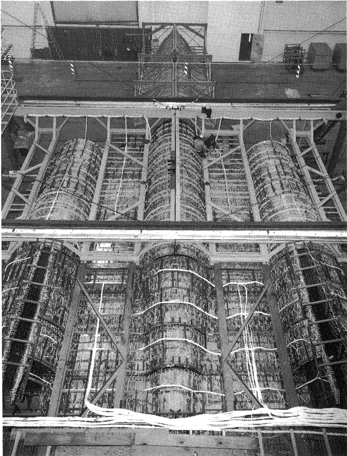
Fig. 31: Overhead view of YF-12 heater system
