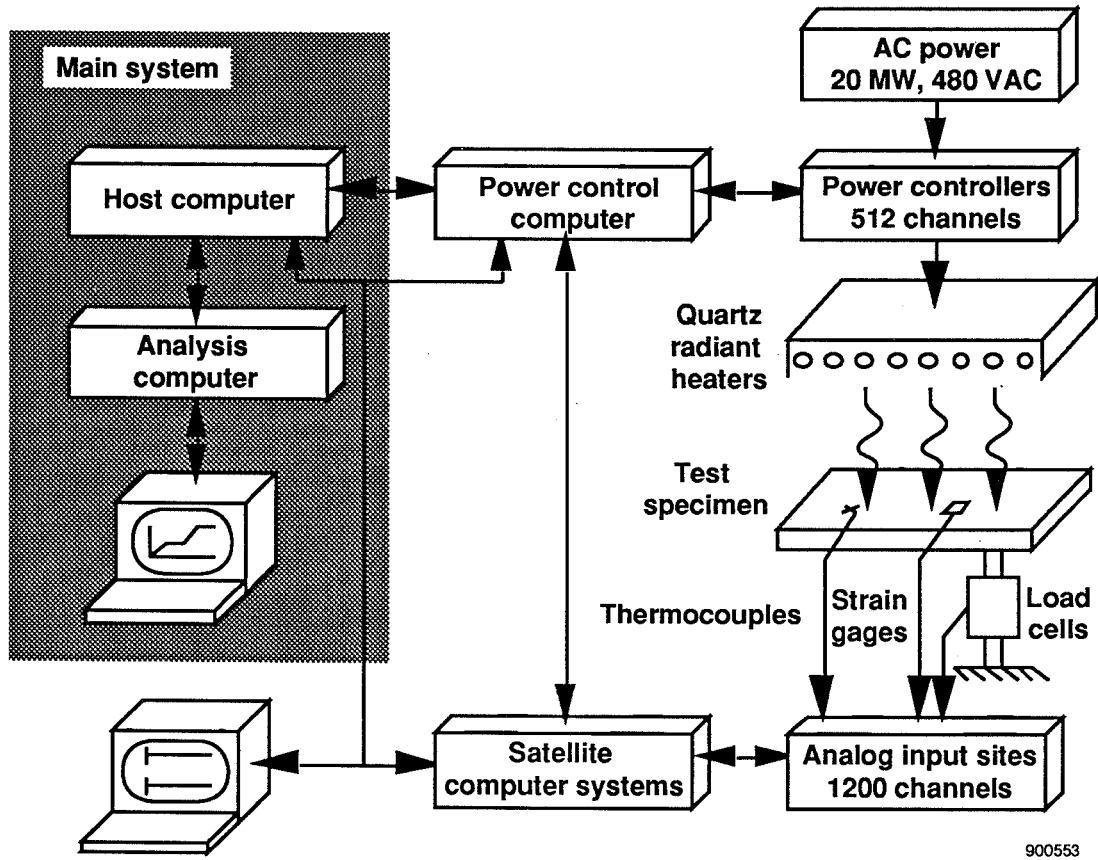
Fig. 18: Data acquisition and control system
