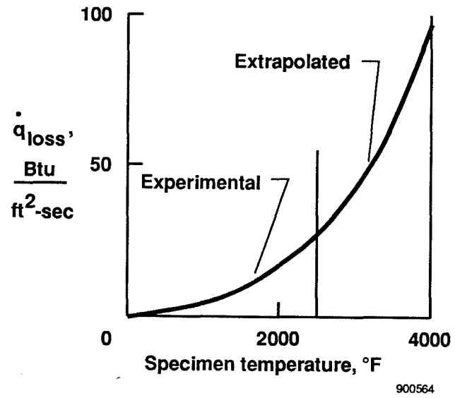
Fig. 15: Heat flux loss
