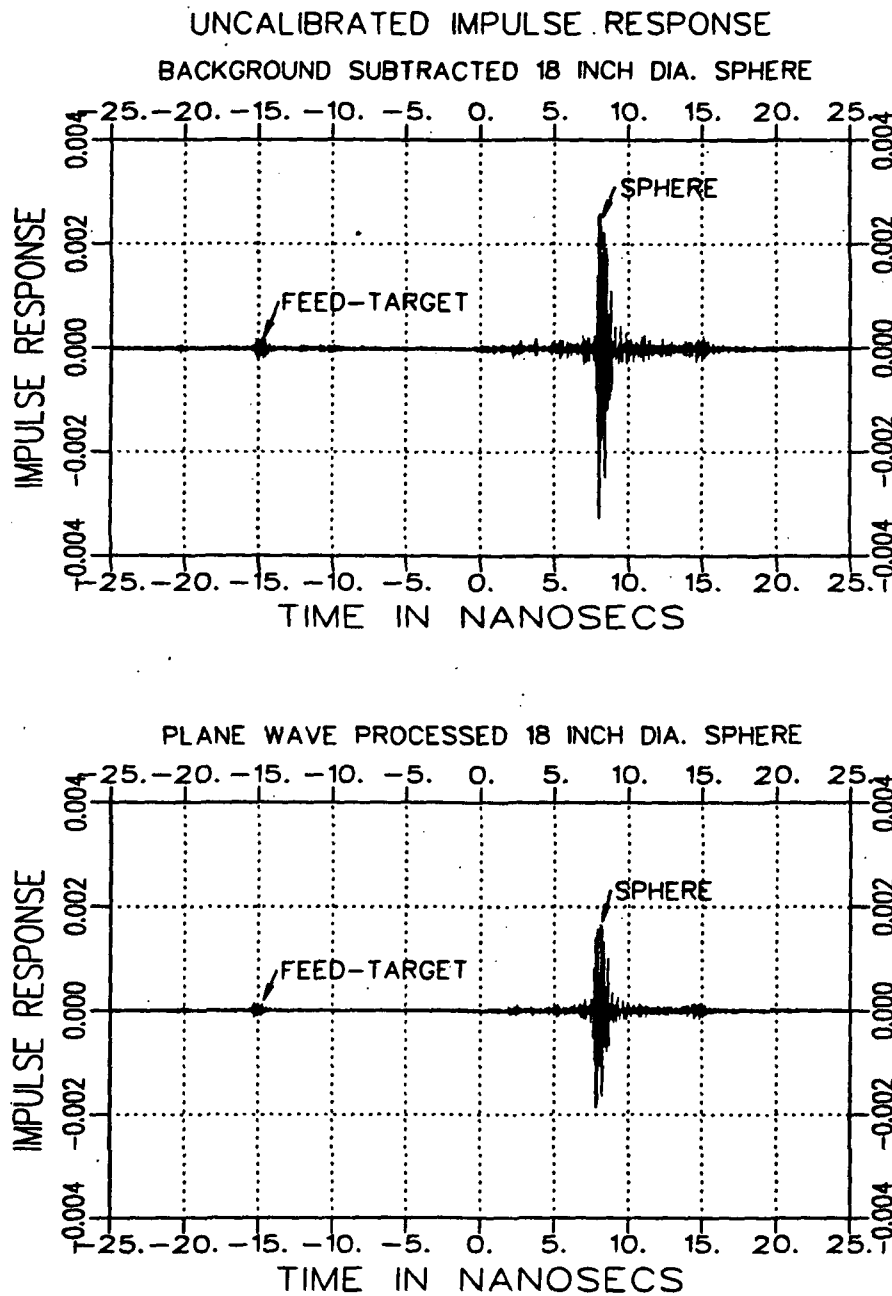
Figure 5.4: Uncalibrated 109 degree bistatic impulse response of single scan position background subtracted 18 inch diameter sphere, and plane wave processed 18 inch diameter sphere plus background. (40,120) Taper.
