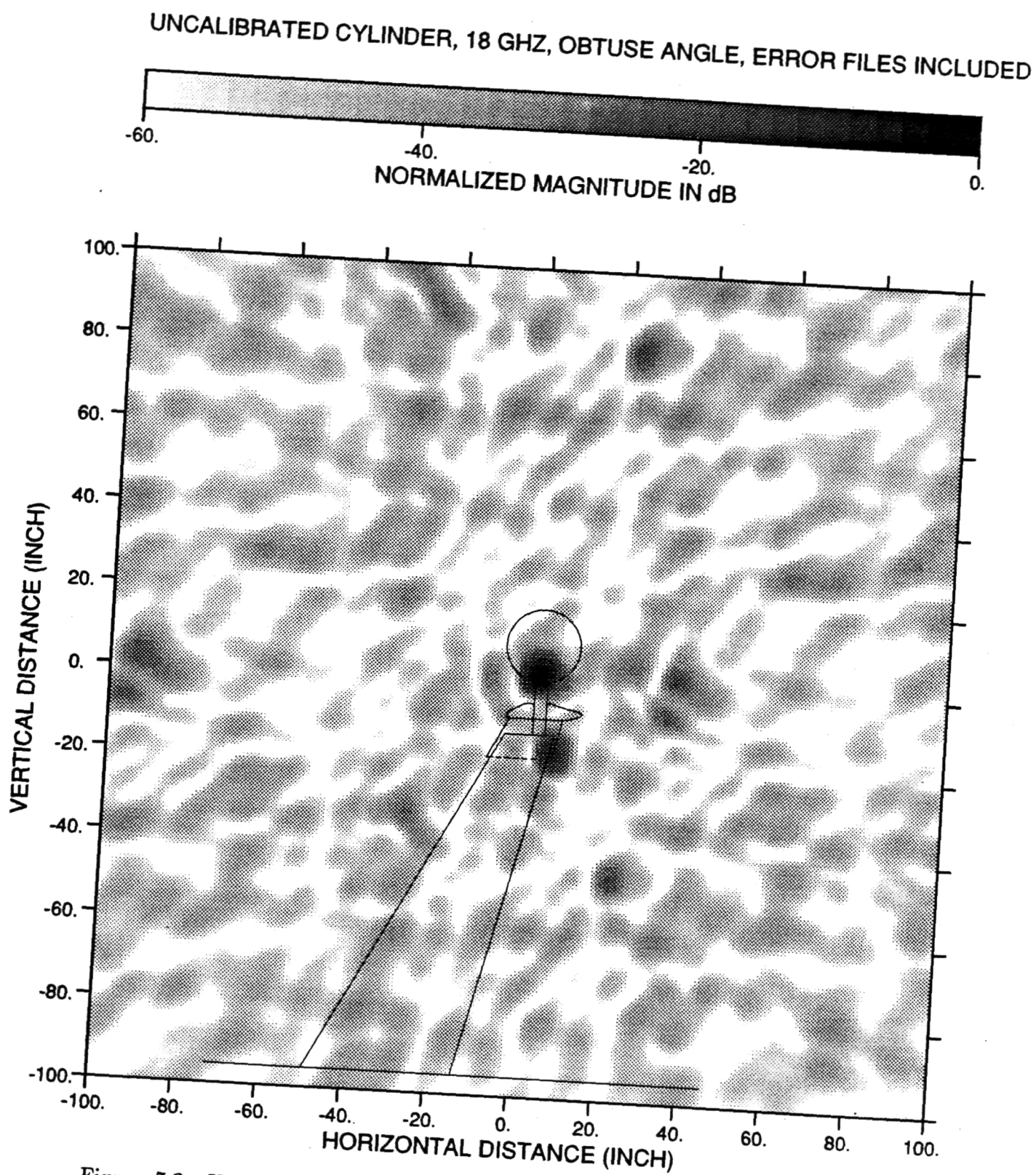
Figure 7.2: Uncalibrated cylinder backprojection plot. 18 GHz, Obtuse bistatic angle, Erroneous files included, Normalized by -42 dB
