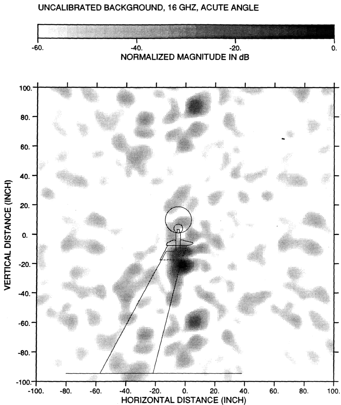
Figure 7.8: Uncalibrated background backprojection plot. 16 GHz, Acute bistatic angle, Erroneous files removed, Normalized by -71 dB
