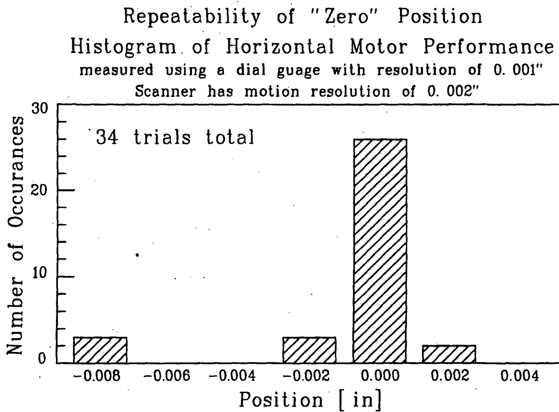
Figure 3.4: Histogram of horizontal motor pair performance indicating "zero" repositioning precision.
