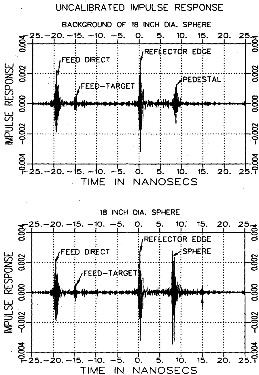
Figure 5.3: Uncalibrated 109 degree bistatic impulse response of an 18 inch diameter sphere plus background, and background alone. Single scan position measurements.
