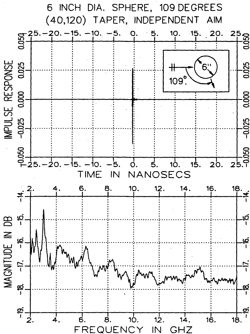
Figure 5.9: Calibrated, 7 point smoothed 109 degree bistatic RCS magnitude and impulse response of a 6 inch diameter sphere, (40,120) Taper, Independent Aim.
