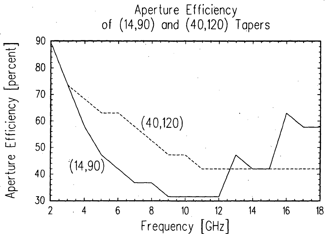
Figure 4.5: Aperture efficiency of ( x\%=14, \text{MPD}=90 ) and ( x\%=40, \text{MPD}=120 ) taper functions projected to the target zone as a function of frequency.
