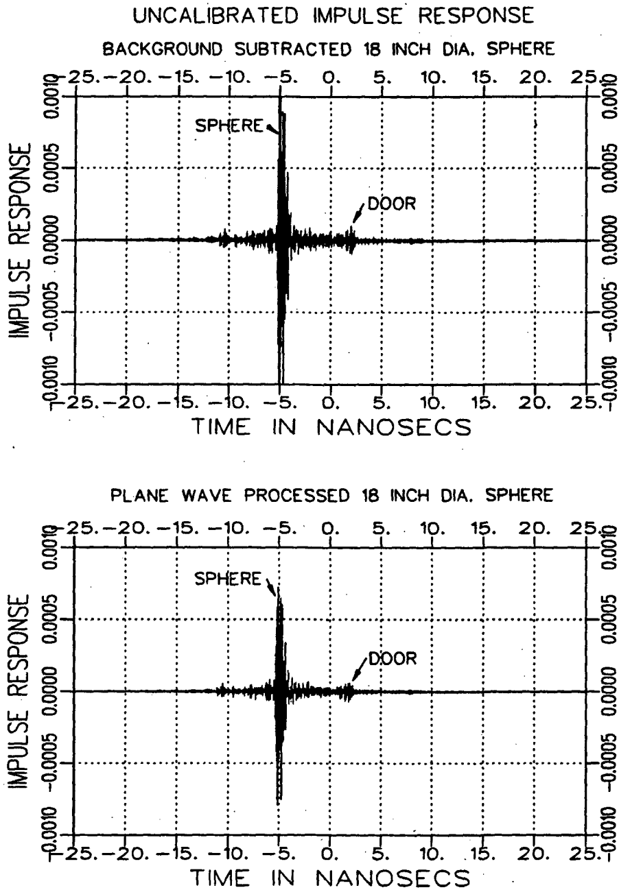
Figure 5.6: Uncalibrated 65 degree bistatic impulse response of single scan position background subtracted 18 inch diameter sphere, and plane wave processed 18 inch diameter sphere plus background. (40,120) Taper.
