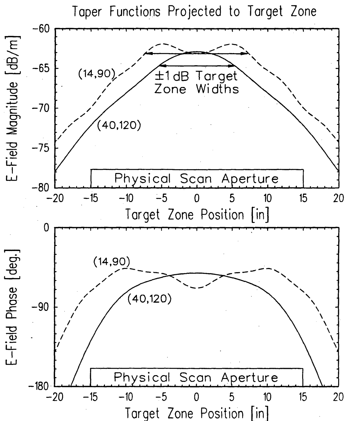
Figure 4.4: Taper functions ( x\%=14, \text{MPD}=90 ) and ( x\%=40, \text{MPD}=120 ) projected to the target zone, 18 GHz.
