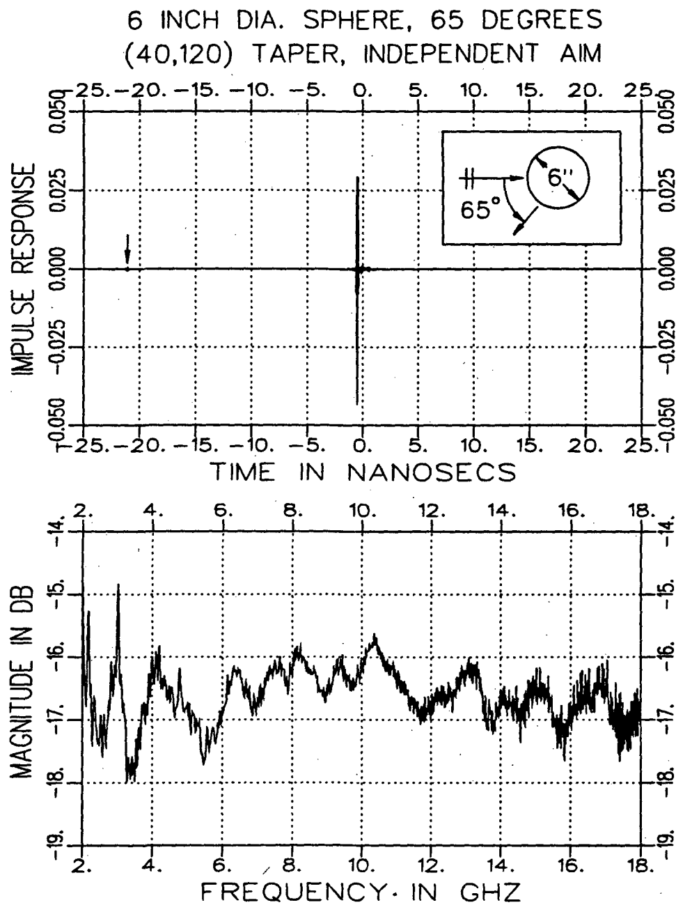
Figure 5.7: Calibrated, unsmoothed 65 degree bistatic RCS magnitude and impulse response of a 6 inch diameter sphere, (40,120) Taper, Independent Aim.
