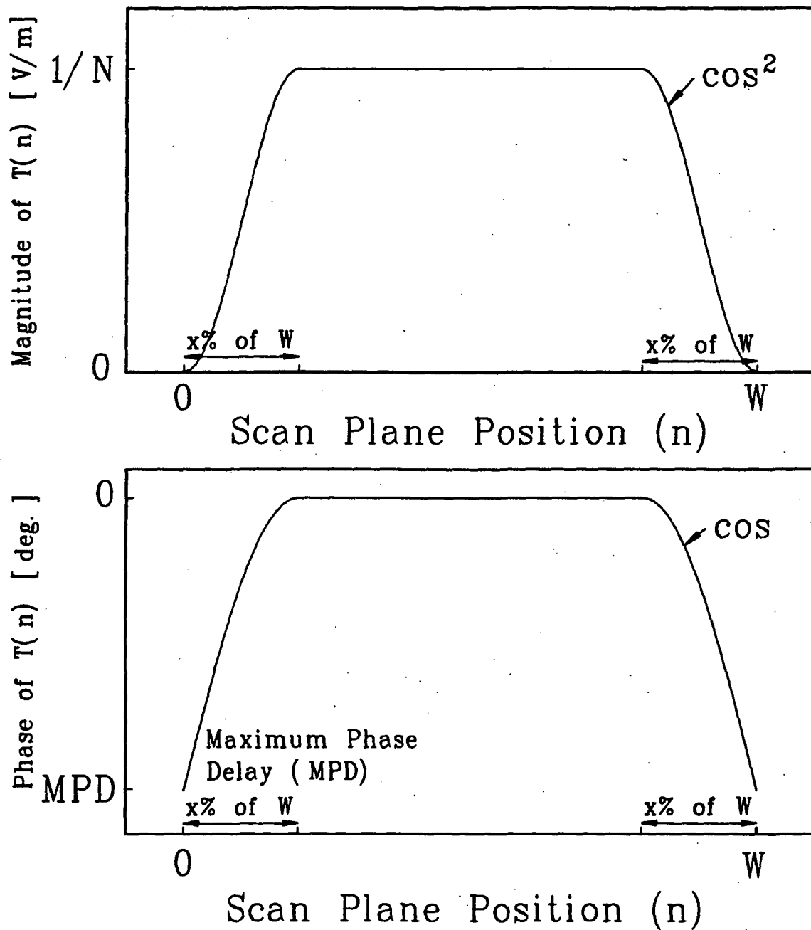
Figure 4.2: Visualization of the aperture taper function.
