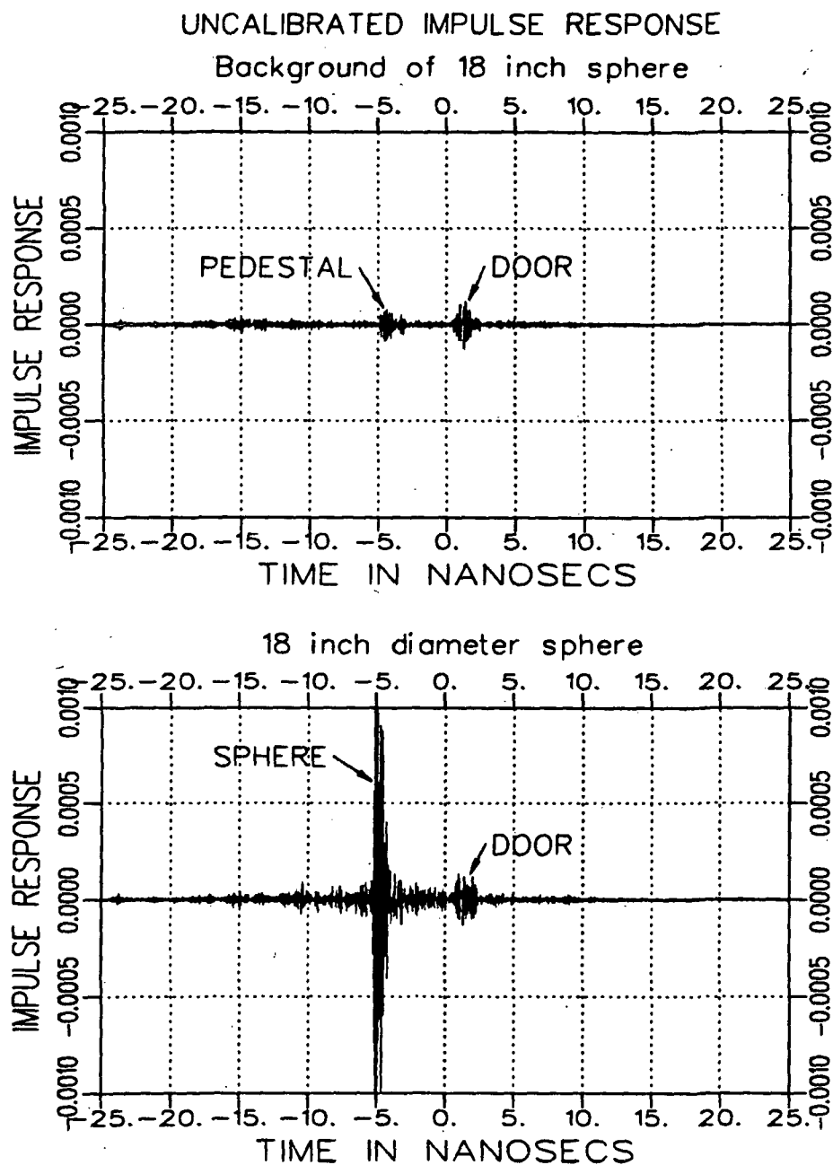
Figure 5.5: Uncalibrated 65 degree bistatic impulse response of an 18 inch diameter sphere plus background, and background alone. Single scan position measurements.
