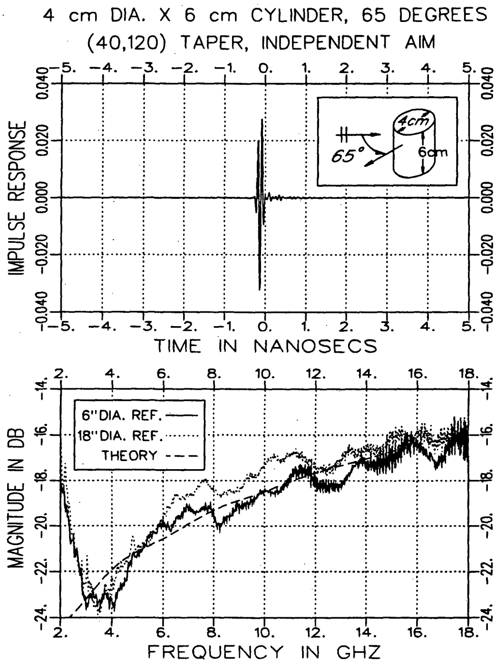
Figure 5.18: Calibrated 65 degree bistatic RCS magnitude and impulse response of a 6 cm tall, 4 cm diameter cylinder for 6 and 18 inch diameter reference targets with exact bistatic RCS magnitude overlay. Independent Aim, (40,120) Taper.
