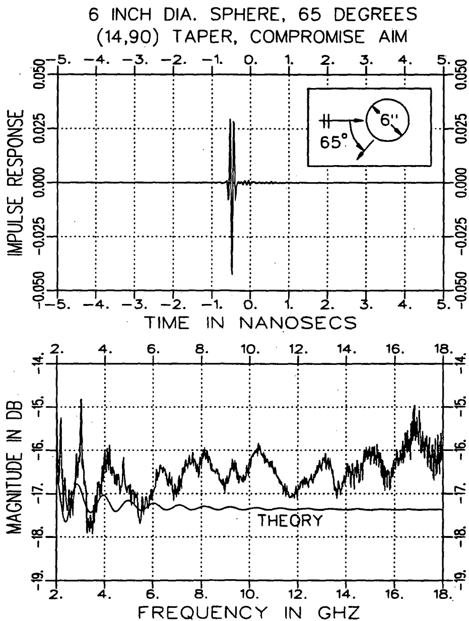
Figure 5.15: Worst calibrated 65 degree bistatic RCS magnitude and impulse response of a 6 inch diameter sphere with theoretical bistatic RCS magnitude overlay. (14,90) Taper, Compromise Aim, 18 inch diameter sphere reference target.
