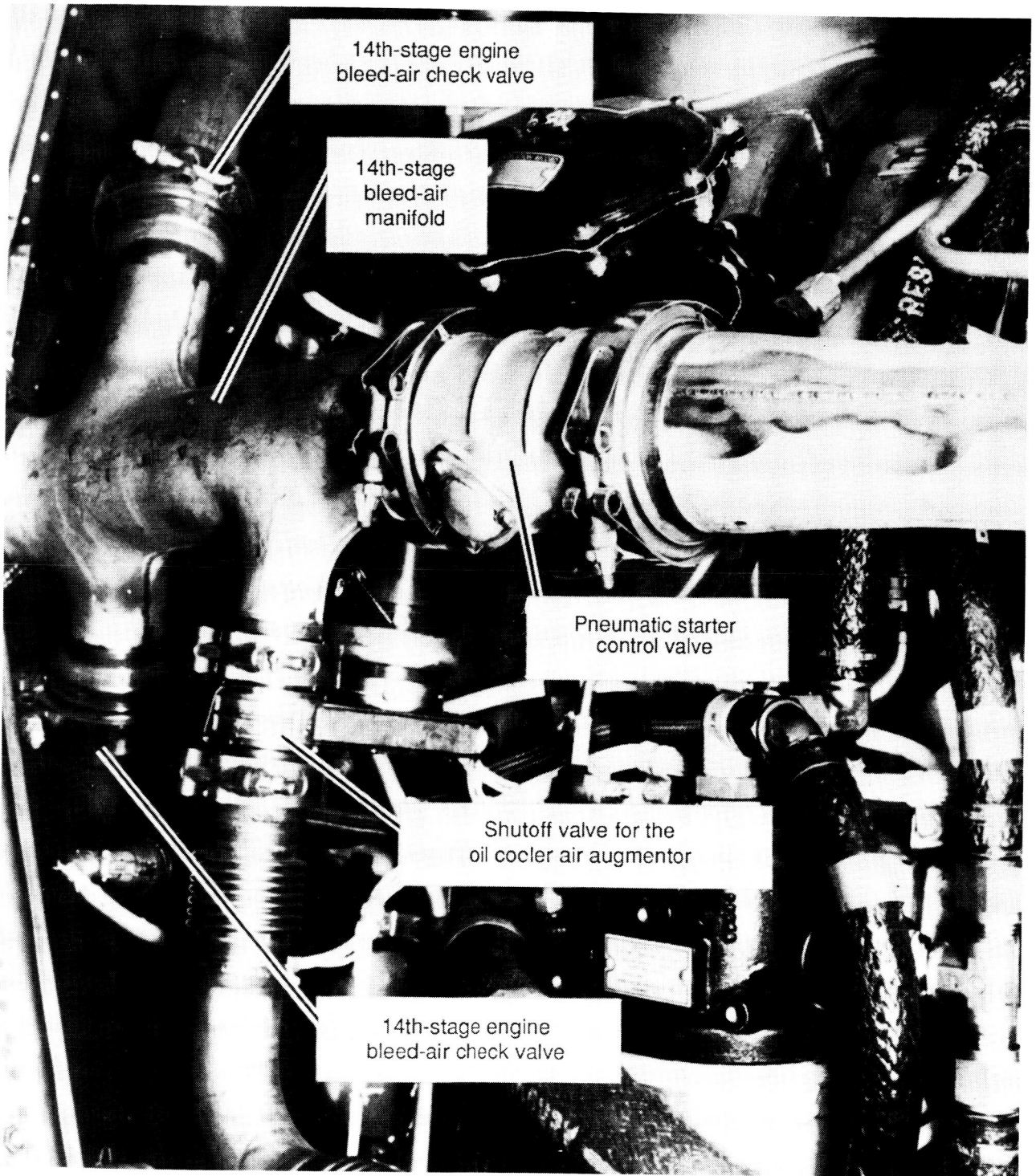
Figure 4. NASA Electra 14th-stage bleed-air manifold configuration with shutoff valve for oil cooler air augmentor.
