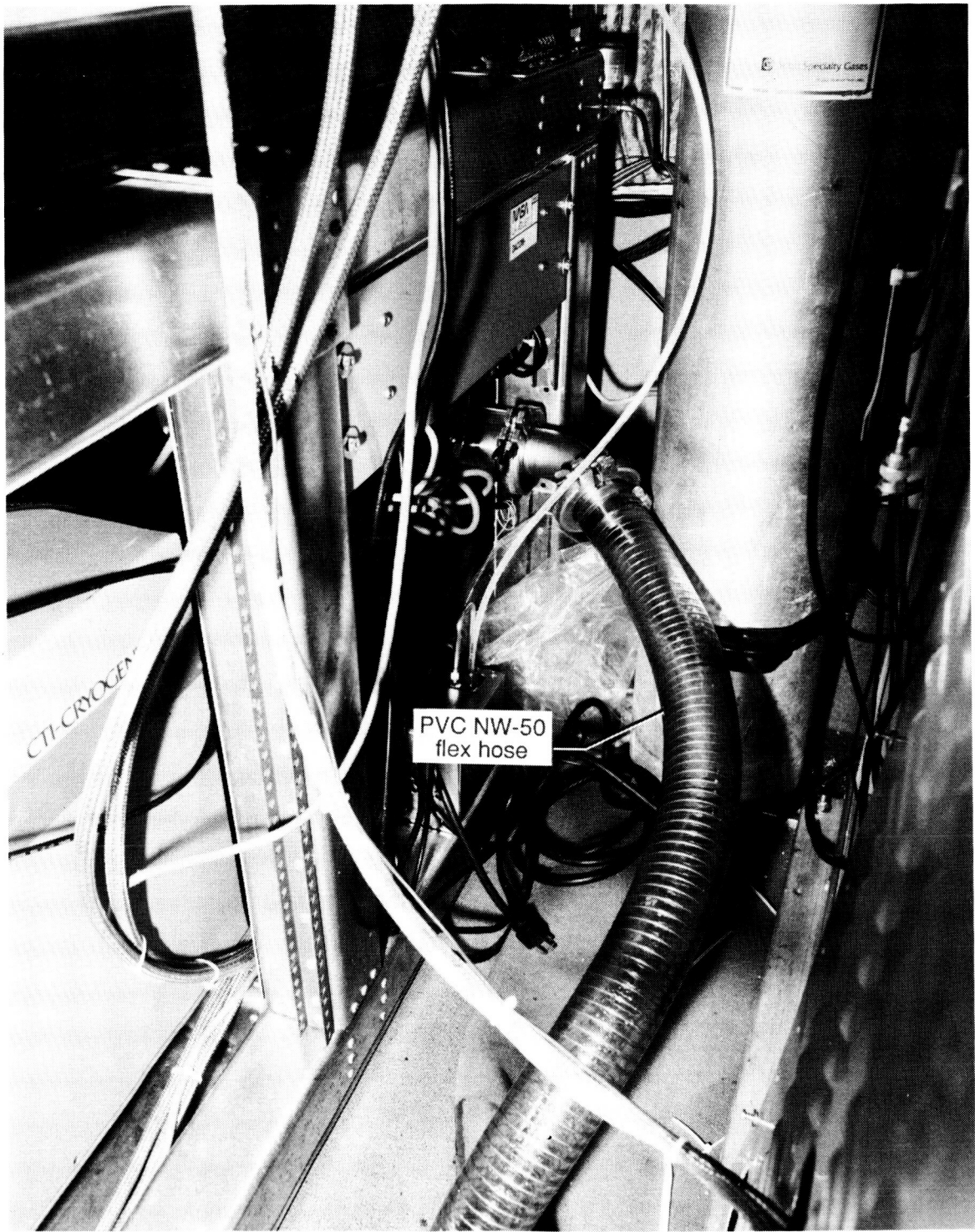
Figure 15. Venturi vacuum line (PVC flex hose) terminating at DACOM system (ABLE-2B mission).
