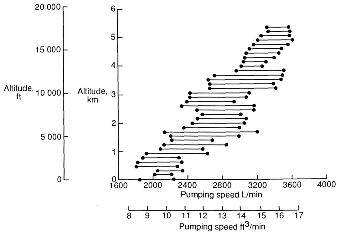
Figure 39. Pumping speed as function of altitude for DACOM-8 venturi during test flights. ABLE-3B mission, flights 1 to 5 (spirals and level); engine no. 2.
