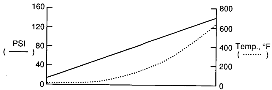
Figure 3. Characteristics of 14-stage compressor used on NASA Electra. 83 percent efficiency; 9.64:1 compression ratio; 554°F temperature rise; 470 ft 3 air/sec. (Based on ref. 14.)
