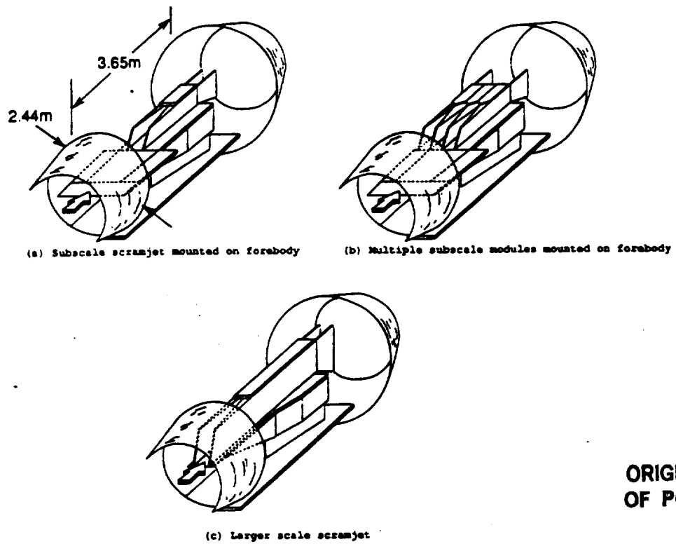
Figure 8.- Scramjet tests planned for the 2.44-meter ETT
