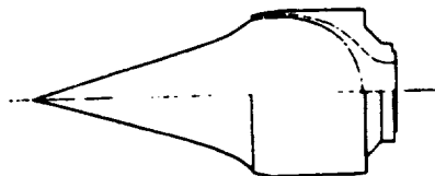
(a) FIXED GEOMETRY, LC CONTRACTION RATIO, ALL-EXTERNAL COMPRESSSION
