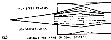
(c) VARIABLE INLET CONE CONCEPT
