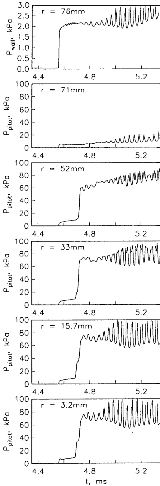
Figure 22: Comparison of wall pressure and Pitot pressure with experiment (case 4, x = 24 \text{ m} ). The experimental data is taken from Shinn and Miller (1978).
