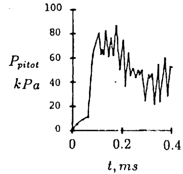
Figure 22: Comparison of wall pressure and Pitot pressure with experiment (case 4, x = 24 \text{ m} ). The experimental data is taken from Shinn and Miller (1978).
