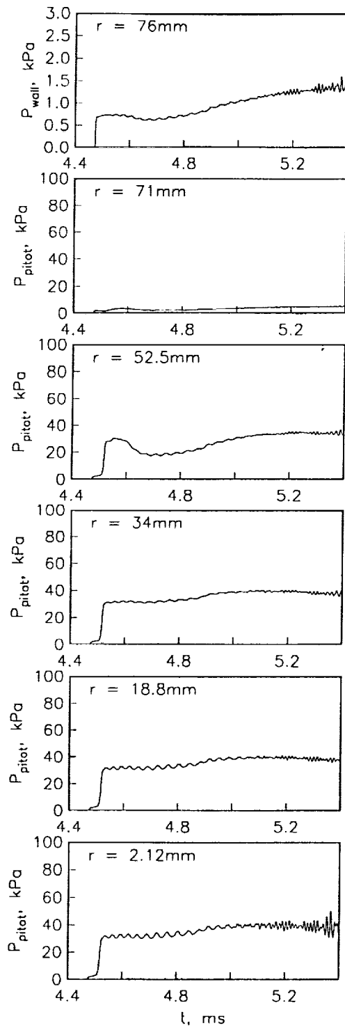
Figure 19: Comparison of wall pressure and Pitot pressure with experiment (case 3, x = 24 \text{ m} ). The experimental data is taken from Shinn and Miller (1978).
