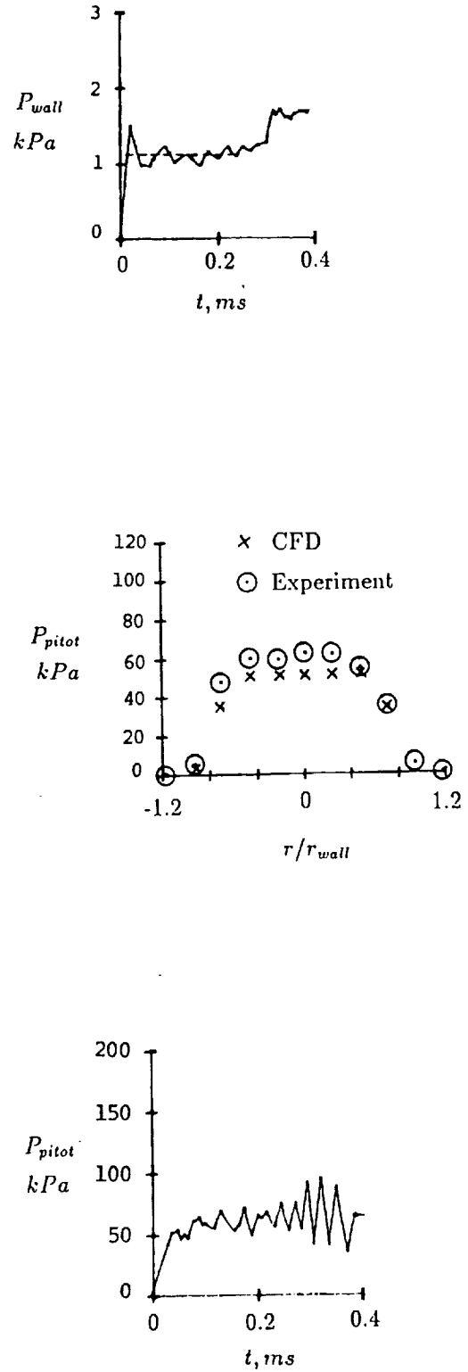
Figure 12: Comparison of wall pressure and Pitot pressure with experiment (case 1, x = 24 \text{ m} ). The experimental data is taken from Shinn and Miller (1978).
