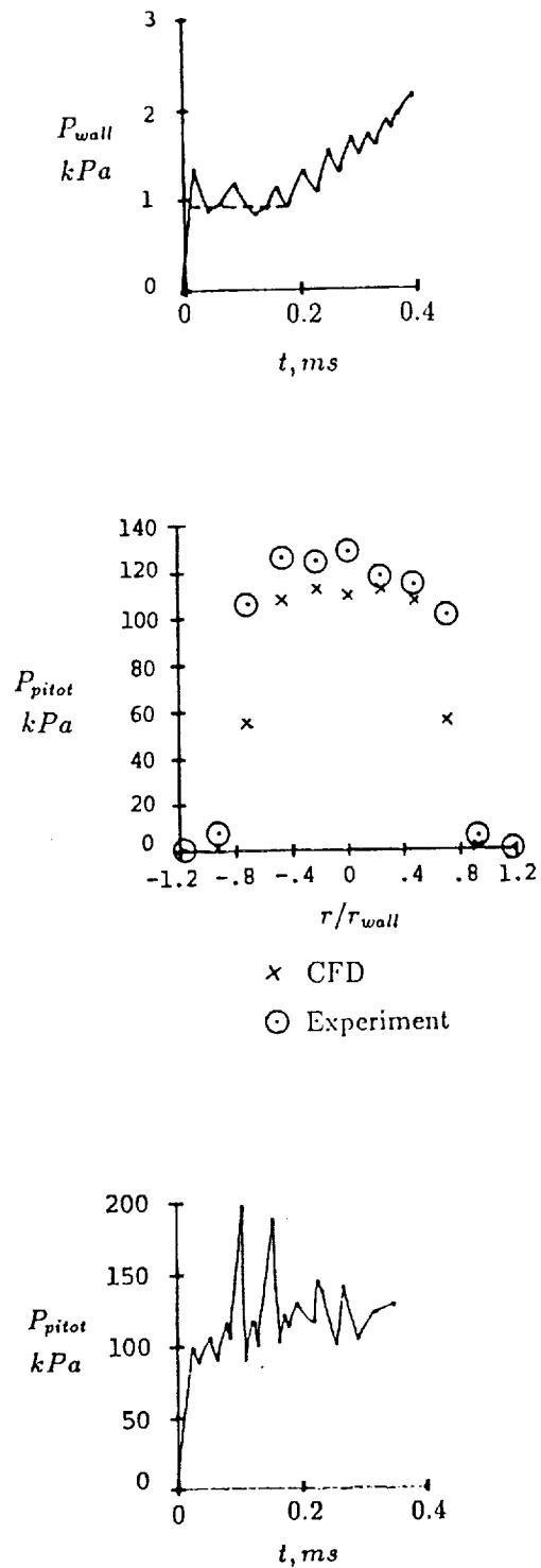
Figure 16: Comparison of wall pressure and Pitot pressure with experiment (case 2, x = 24 \text{ m} ). The experimental data is taken from Shinn and Miller (1978).
