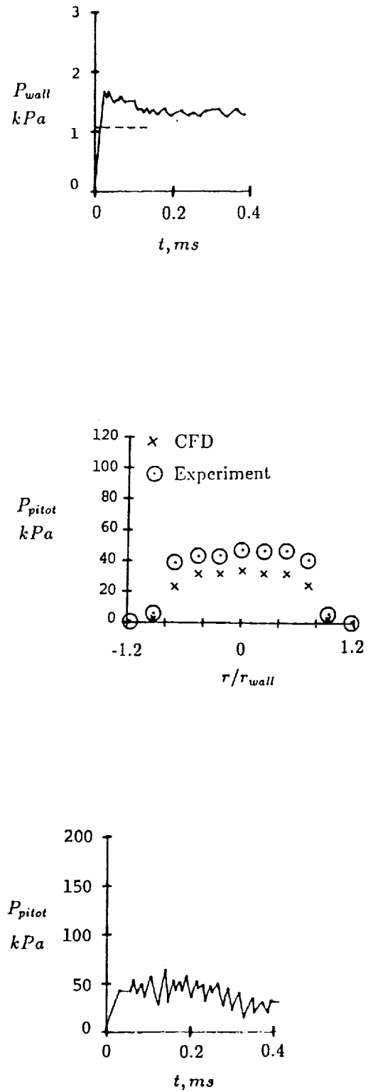
Figure 19: Comparison of wall pressure and Pitot pressure with experiment (case 3, x = 24 \text{ m} ). The experimental data is taken from Shinn and Miller (1978).
