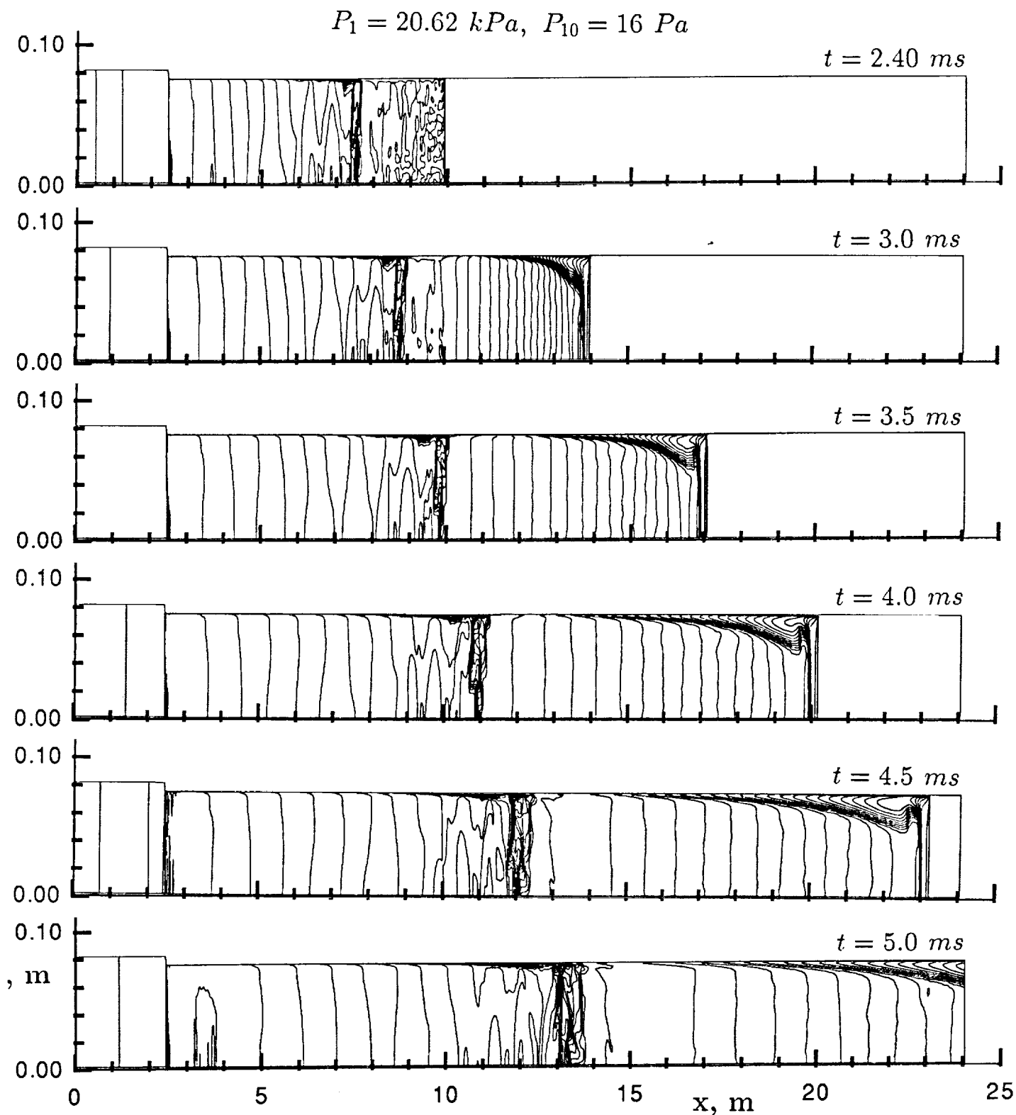
Figure 14: Density contours showing the unsteady expansion of the test gas for case 2.
