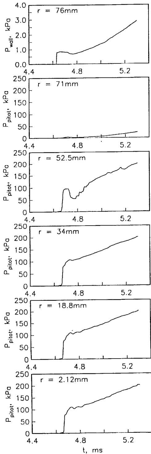
Figure 16: Comparison of wall pressure and Pitot pressure with experiment (case 2, x = 24 \text{ m} ). The experimental data is taken from Shinn and Miller (1978).
