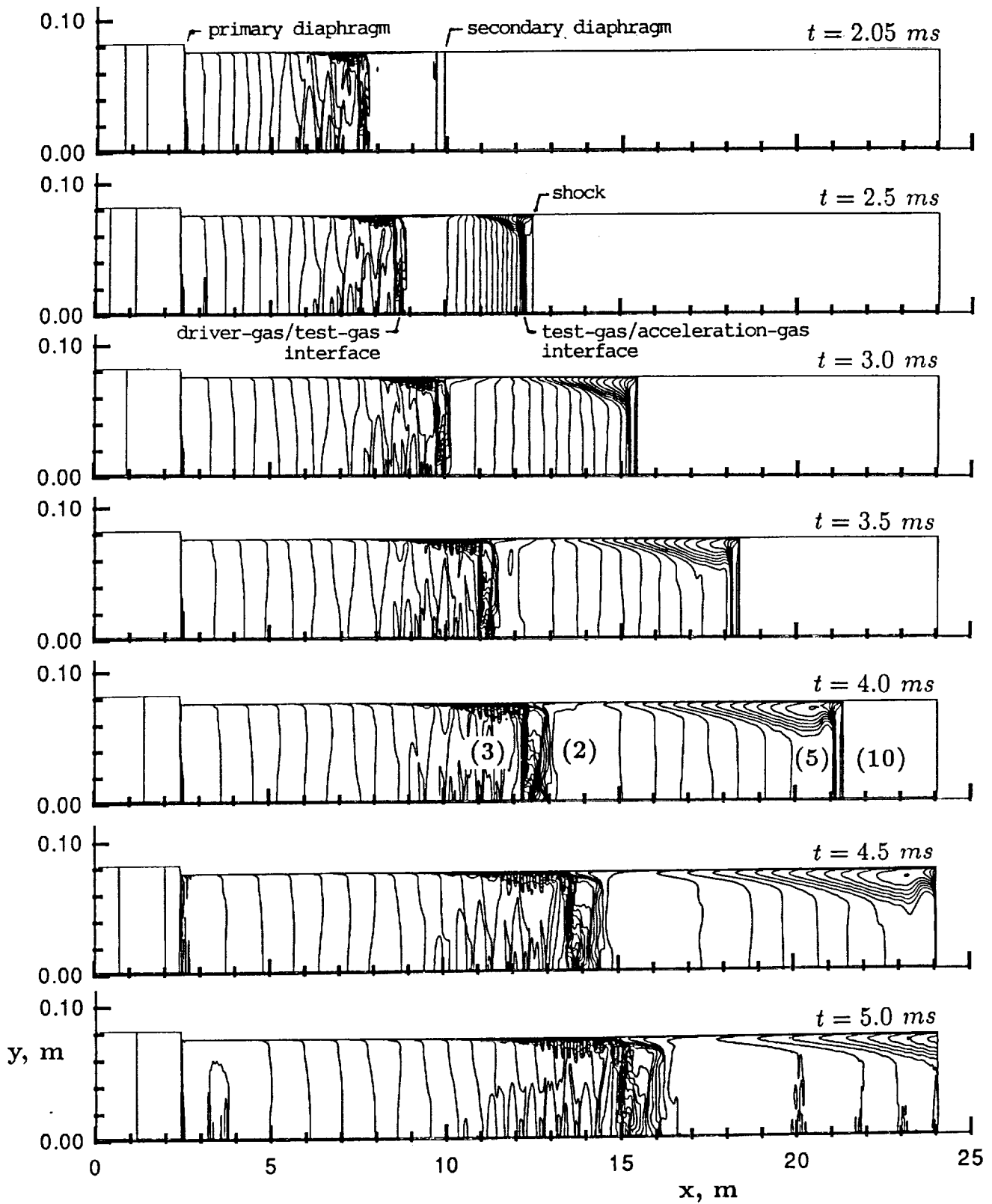
Figure 8: Density contours showing the unsteady expansion of the test gas for case 1.
