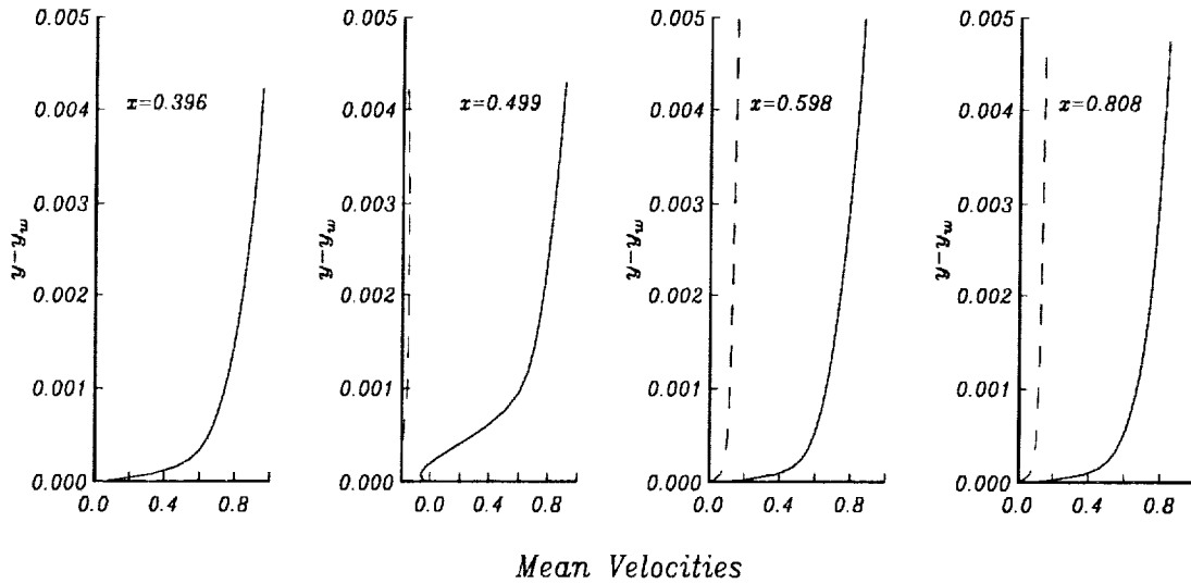
Figure 3: Streamwise variation of mean velocity profiles for 10° compression ramp using a two-equation turbulence model: \tilde{u}/U_\infty , —; \tilde{v}/U_\infty , — —.
