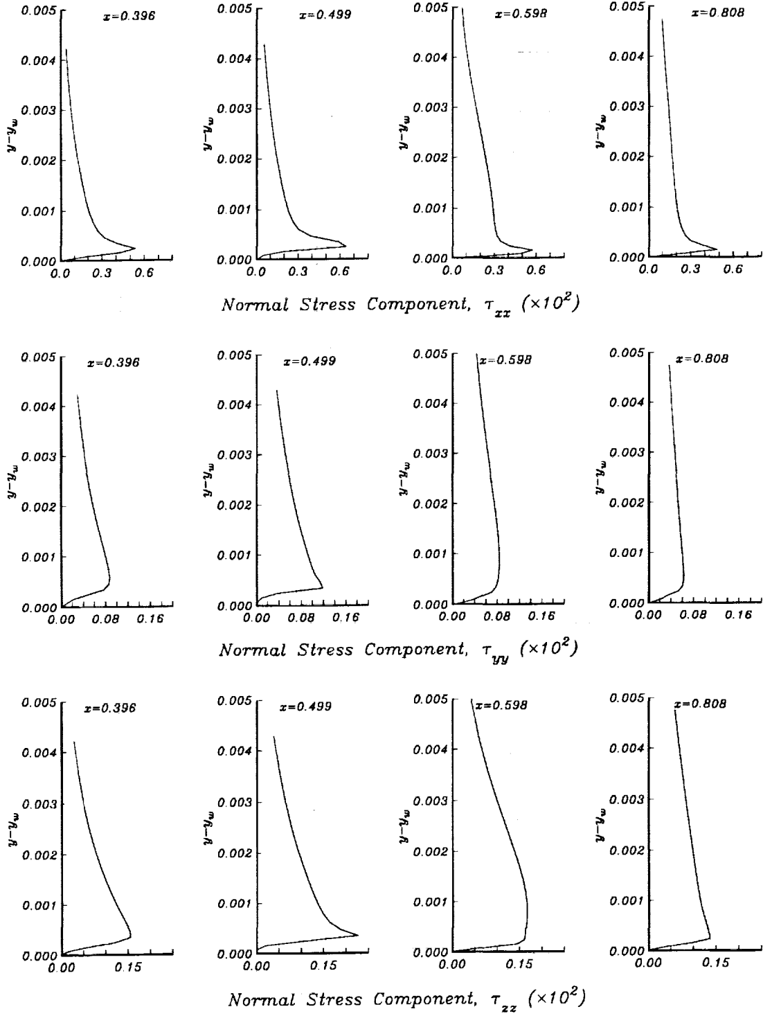
Figure 10: Normal Reynolds stress component profiles for 10° compression ramp.
