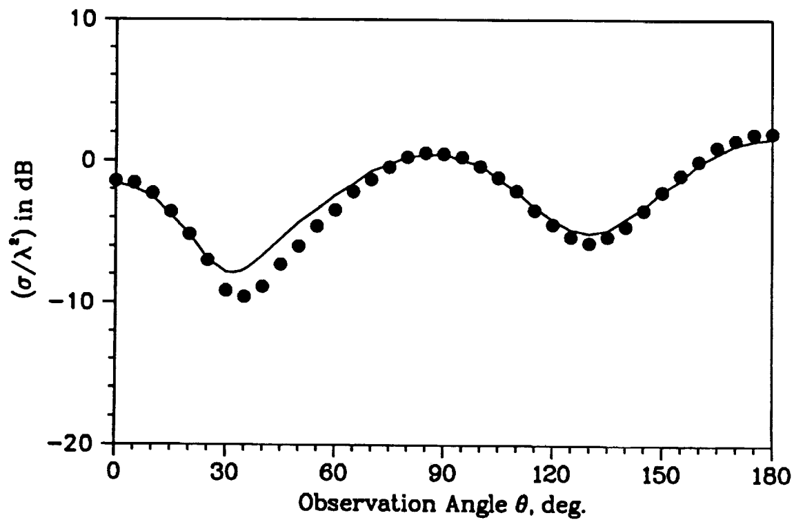
Figure 8: RCS pattern in the x-z plane for the geometry in figure 6 with the air-filled section replaced with dielectric having \epsilon_r = 2 - j2 . The solid curve is the FE-ABC pattern and the black dots are MoM data for the E_z^{inc} = 0 polarization.
