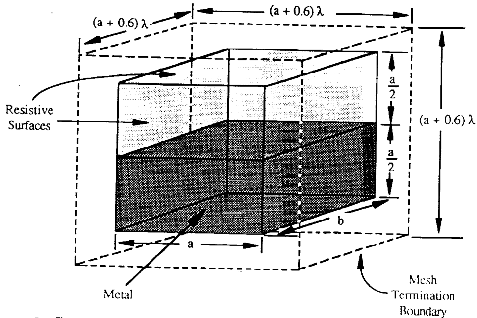
Figure 6: Geometry of a cube ( a=b=0.5\lambda ) consisting of a metallic section and an air-filled section, where the latter is bounded by a resistive surface having R = Z_0 . The outer cube drawn with dashed lines represents the surface on which the ABC was enforced.
