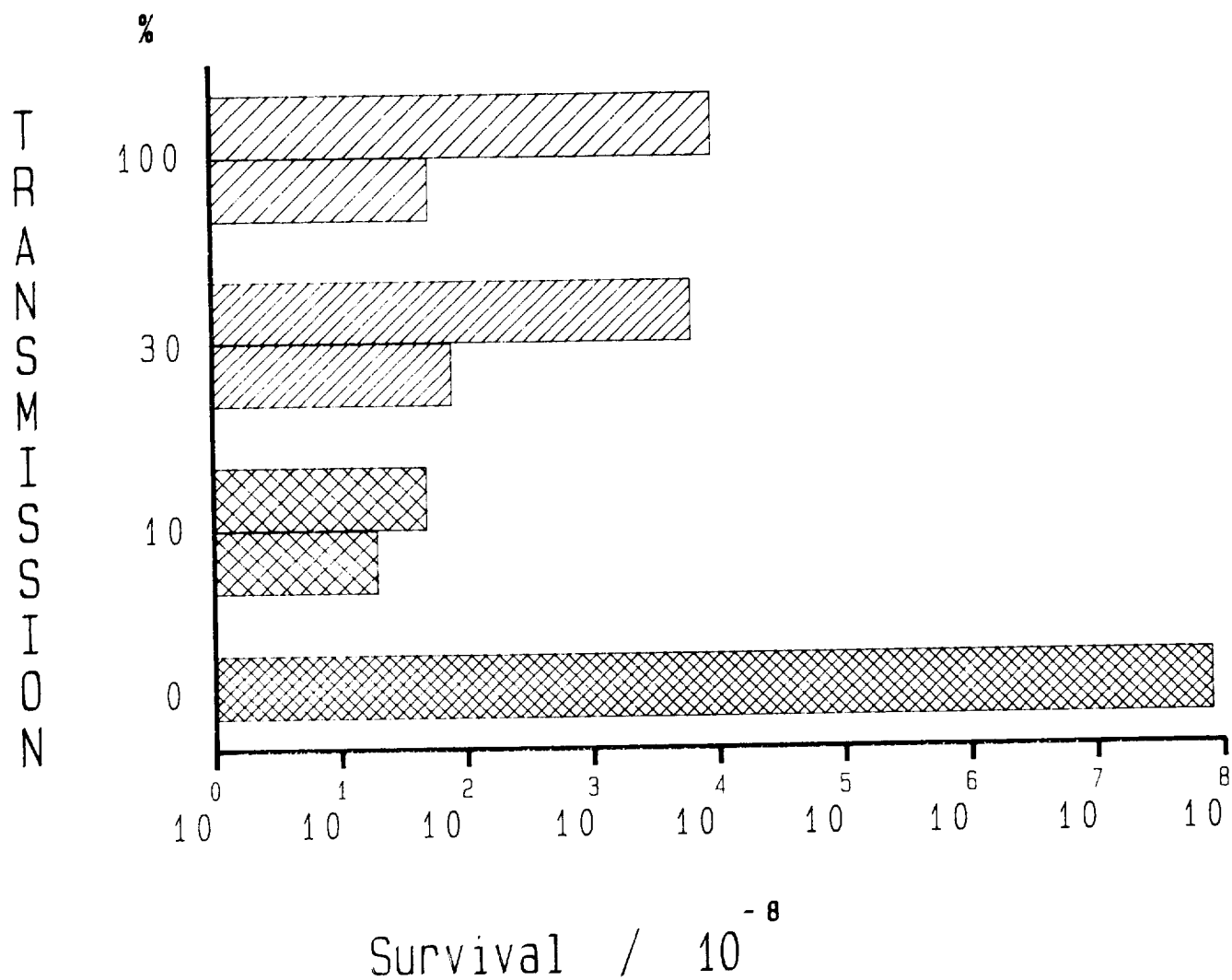
Fig. 1. Survival of Bacillus subtilis spores exposed to the space environment for nearly 6 years during the LDEF mission (April 7, 1984 - January 12, 1990). Spores were exposed in multilayers in the presence of 5 % glucose on quartz discs beneath a perforated dome without any further cover (100 % transmission), or beneath neutral density filters (30 % or 10 % transmission for solar UV-light of wavelengths >170 nm), or beneath an aluminum plate of 2 mm (0 % transmission). Non-covered samples received a solar UV-irradiation of 1 \times 10^9 \text{ J/m}^2 .
