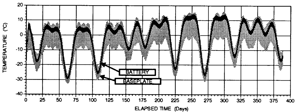
Figure 7: Battery and baseplate temperature for first 388 days
