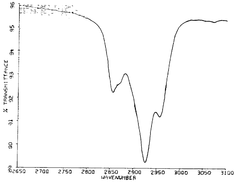
Figure 9. 3.4 \mu spectrum of CaF 2 window.
