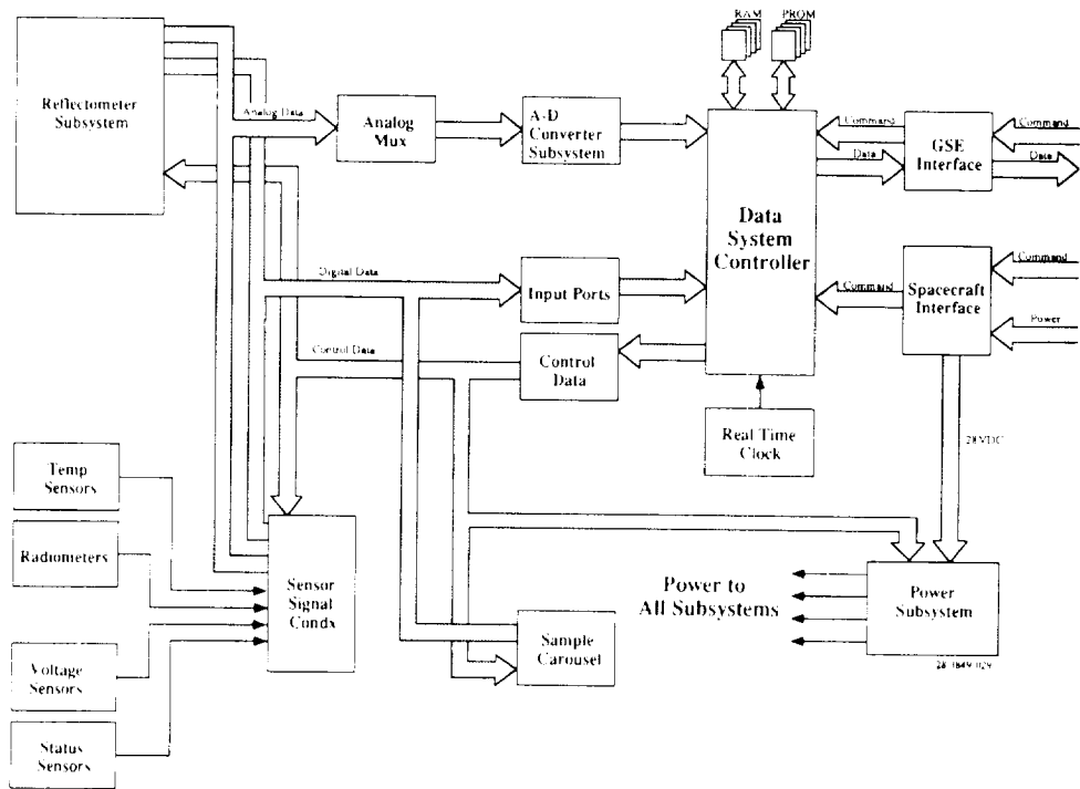
Figure 5 - TCSE Data and Control System
