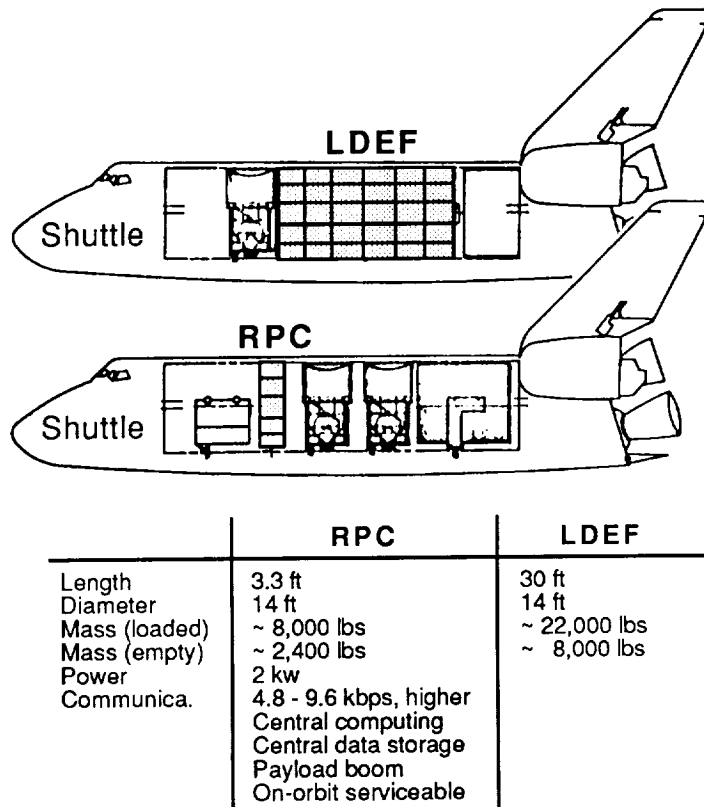
Figure 3. RPC and LDEF Comparison
