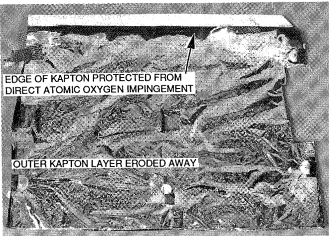
FIGURE 19. SEGMENT OF MLI BLANKET AFTER FLIGHT
