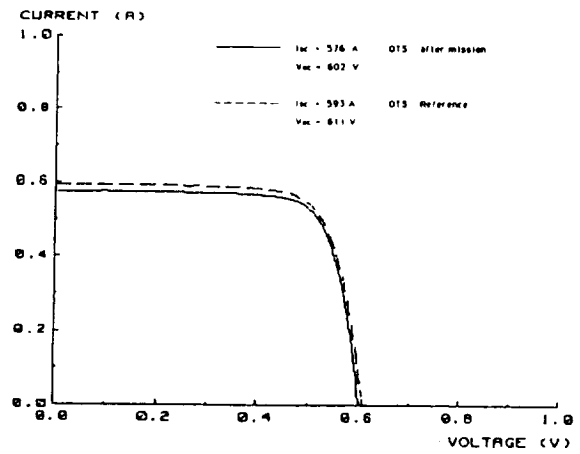
Figure 23: IV - Characteristic OTS solar cell module
