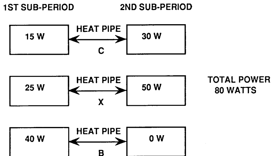
Figure 4. Heater Power Input
