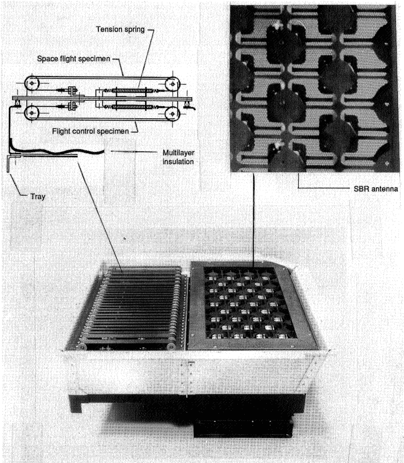
Figure 1. Space-based radar phased-array antenna experiment.
