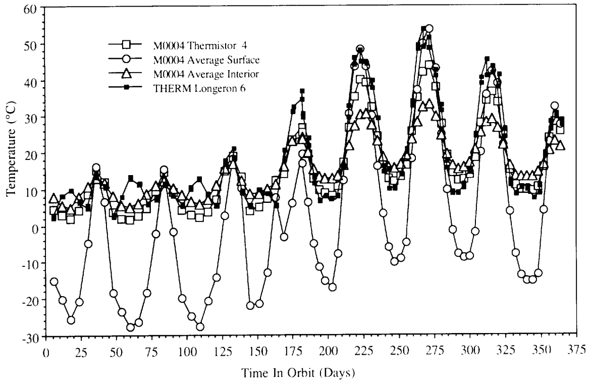
Figure 4. Comparison of M0004 and selected THERM experiment temperature data
