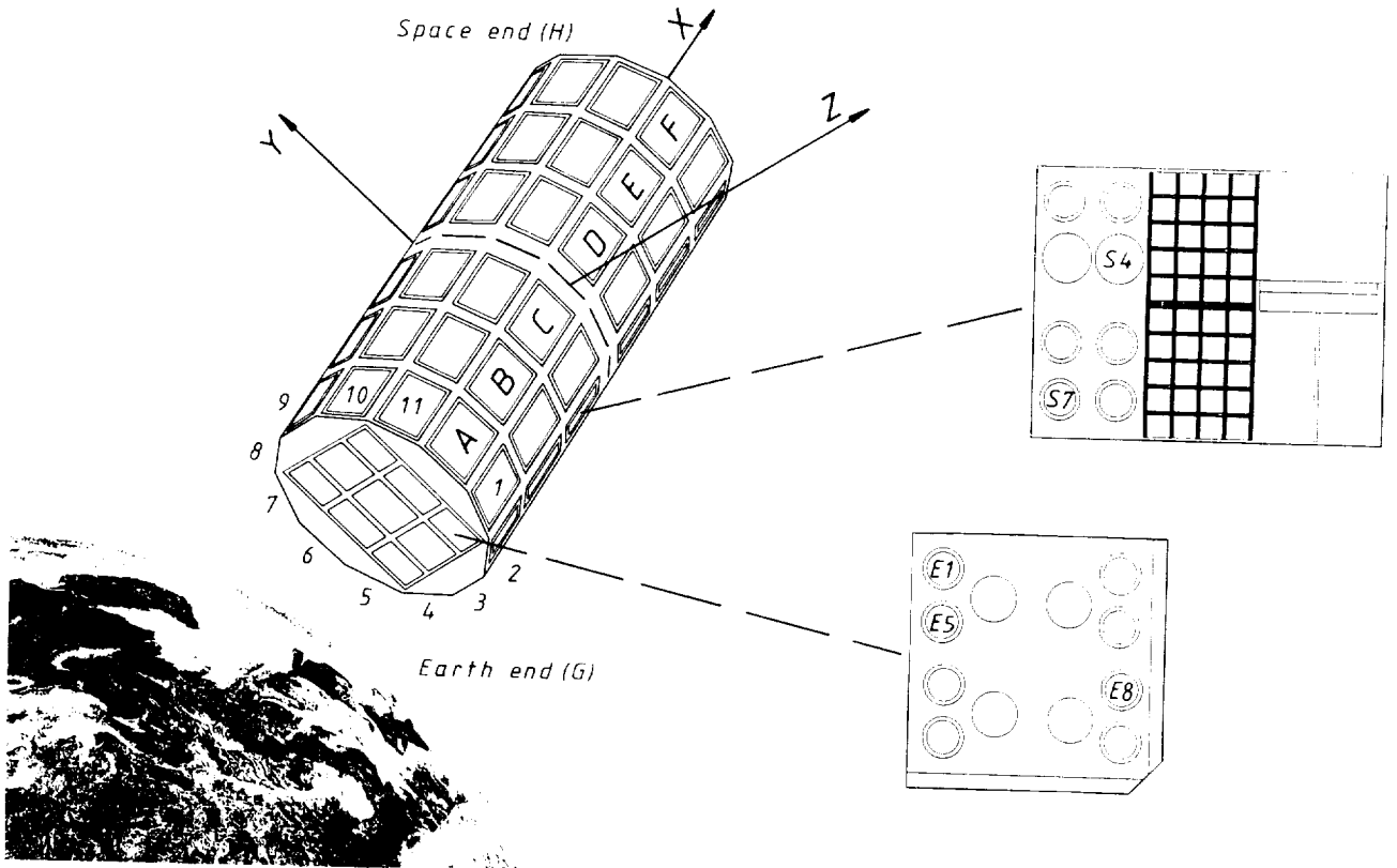
Fig. 1 Location of Biostack experiment units E1, E5, E8, S4, and S7 on the trays G2 and C2 of the LDEF and its orientation in orbit. The velocity vector is in direction of the y-axis; row 9 is therefore the leading and row 3 the trailing edge. The LDEF is gravity gradient stabilized.
