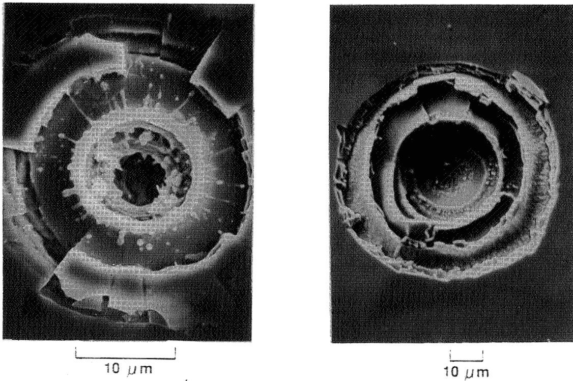
FIGURE 13. Impact craters from sample #3 revealing details of the multilayer structure of the coating. Note the melted areas in the smaller crater on the left.
