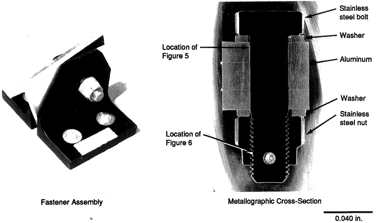
Figure 4. Unassembled Intercostal Fastener Assembly
