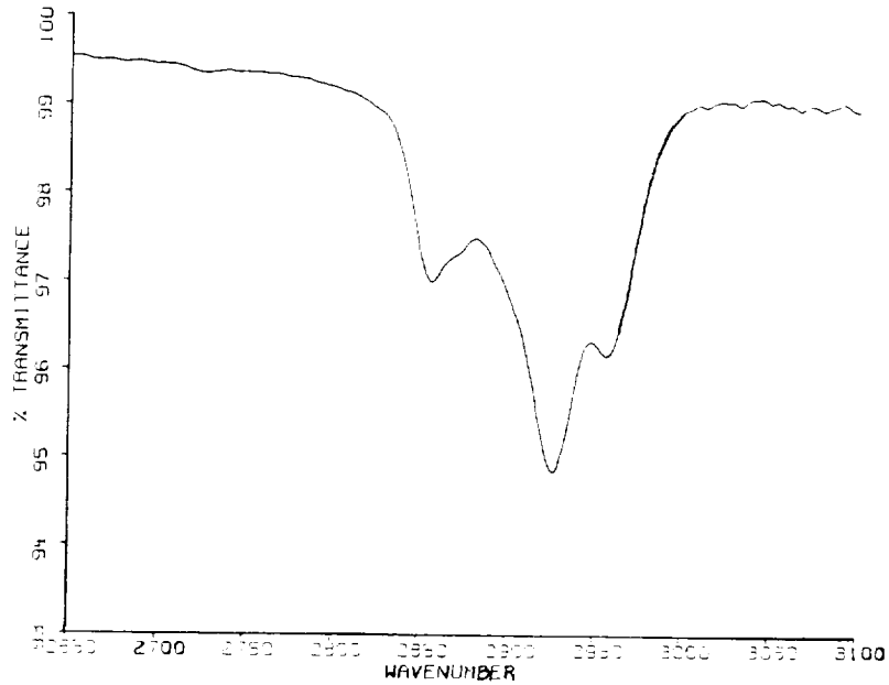
Figure 10. 3.4 \mu spectrum of both surfaces of MgF 2 window.
