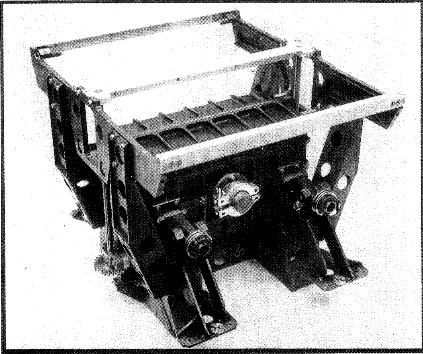
Fig. 1. FRECOPA CANISTER IN CLOSED POSITION
