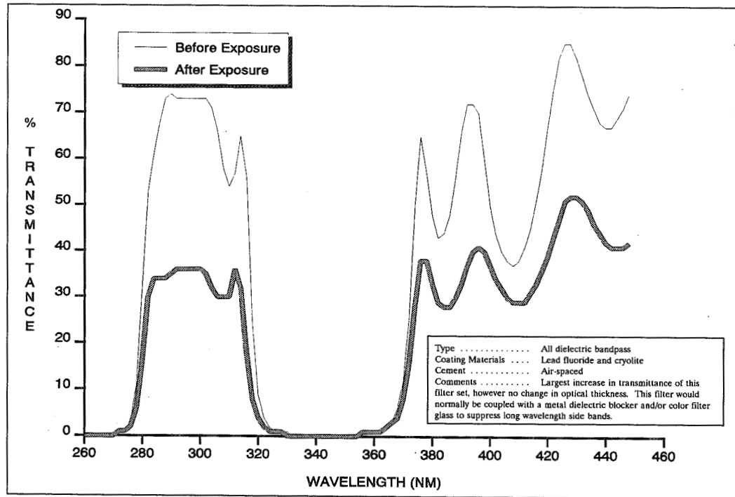
LDEF Filter No. 9
