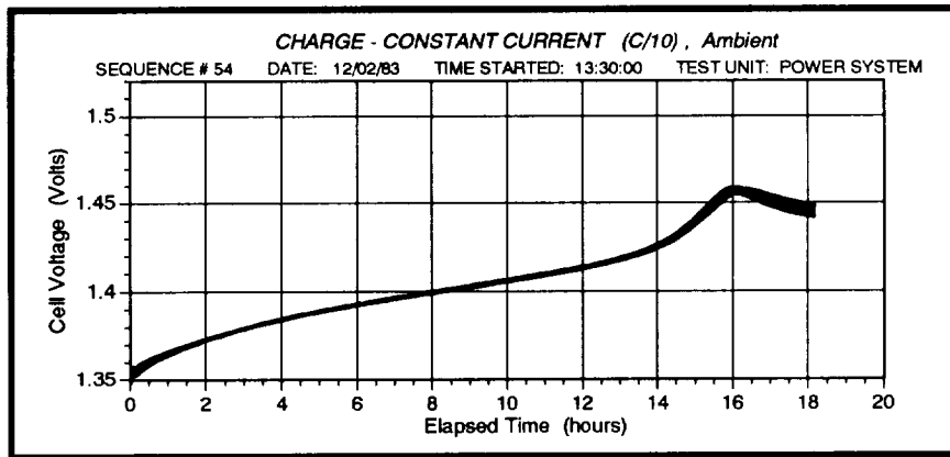
Figure 14: Pre-flight Capacity Charge
