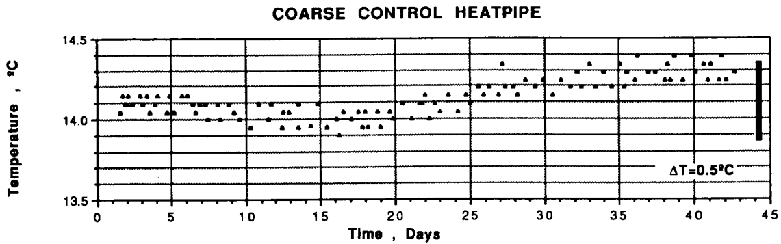
FIGURE 14. TEMPERATURE HISTORIES OF VCHPs
