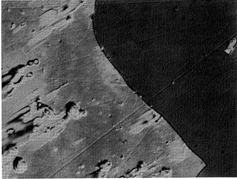
Figure 5. Photograph of MgF 2 window, back surface, 1000X.
