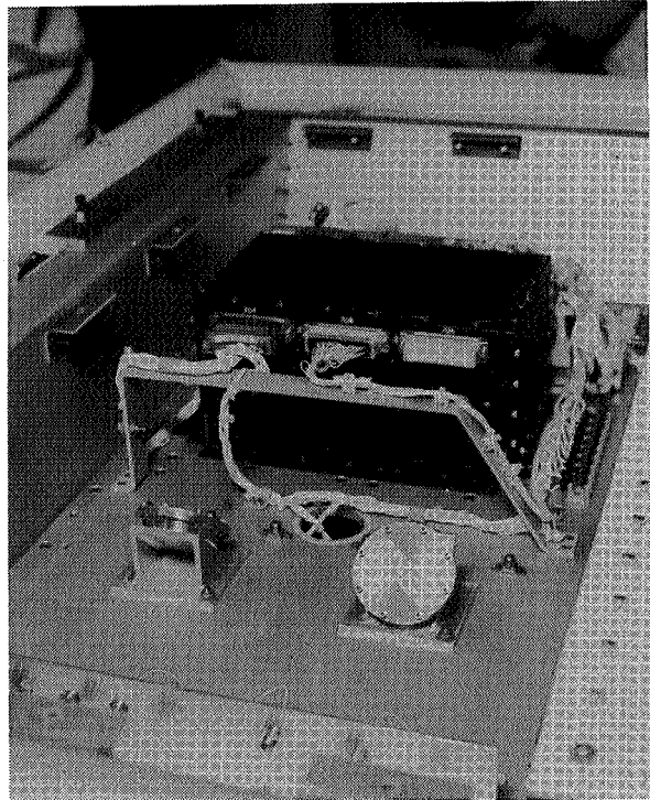
Figure 6. Location and orientation of dosimeters
