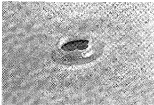
FIGURE 24. MICROMETEOROID IMPACT ON SILVER/TEFLON RADIATOR
