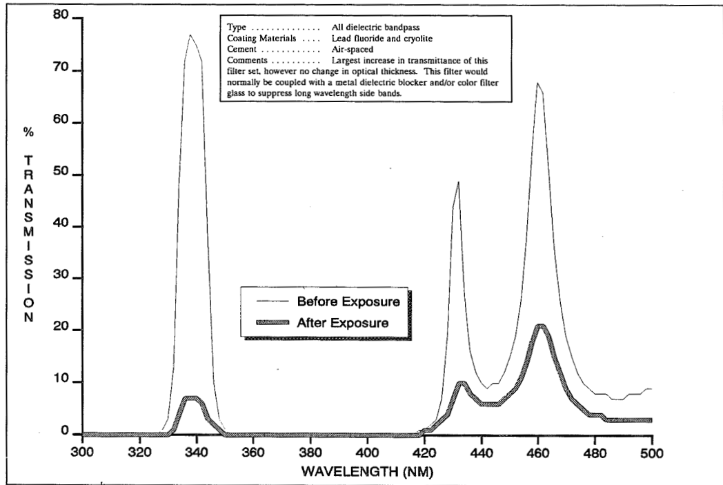
LDEF Filter No. 8
