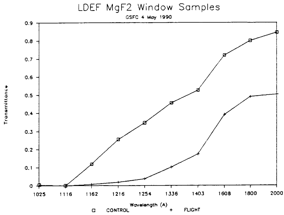
Figure 19. Vacuum ultraviolet transmission of center (front surface) of MgF2 window.
