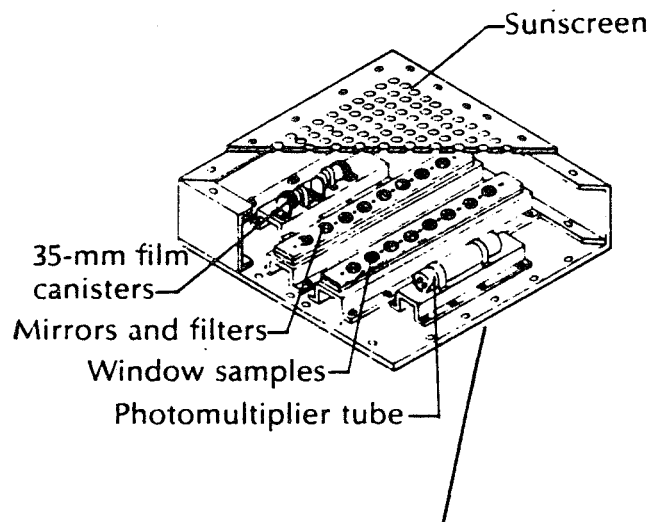
Figure 3. Drawing of Experiment S0050-1.
