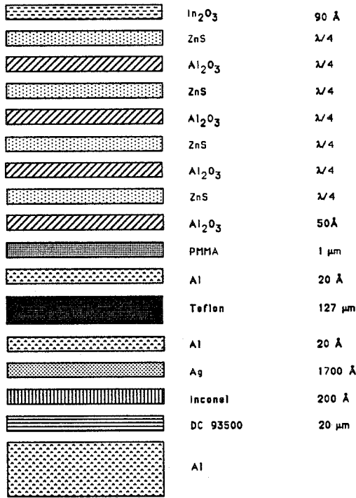
Figure 6: Configuration SSM/IF/LS
