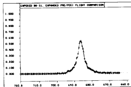
08-11 Exposed 14.5um 0.7% HBW Split-Spacer Fabry-Perot Bandpass Filter Detailed Pre/Post Flight Transmission Measurement (11.9 - 15.4um) (Equivalent to sample 08-10 above)
