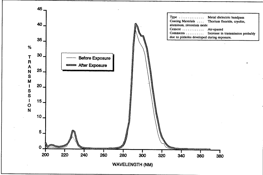
LDEF Filter No. 3
