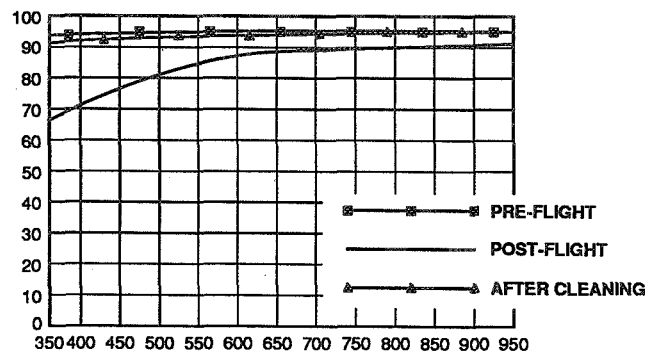
SPECTRAL TRANSMISSION OF UNCOATED FUSED SILICA
