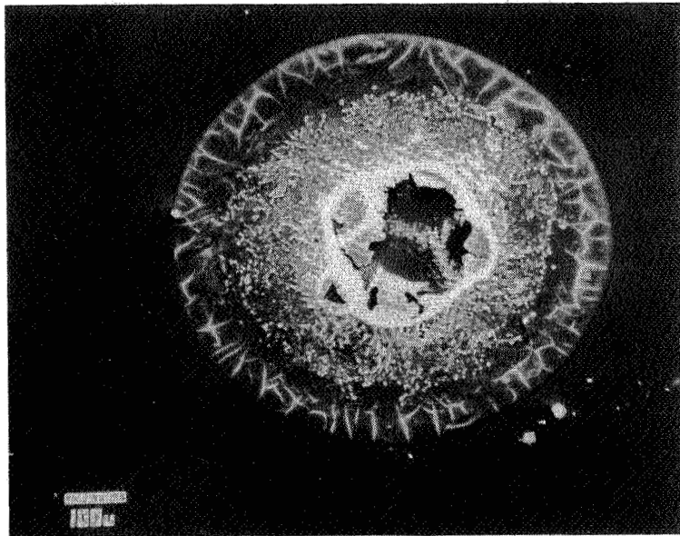
Figure 8. Conglomerate micrometeoroid or debris impact on aluminum oxide coated Kapton flown on STS-8.
