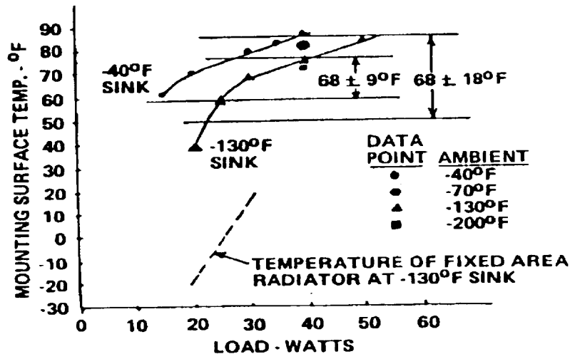
Figure 5. Thermal Vacuum Test
