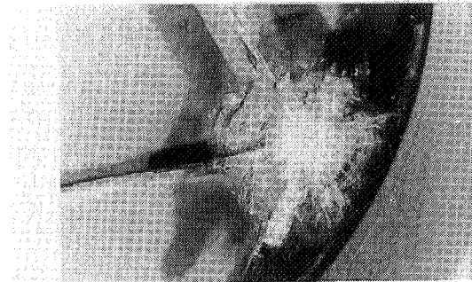
Fig 10. Micrometeorite impact damage on Calcium Fluoride filter.
