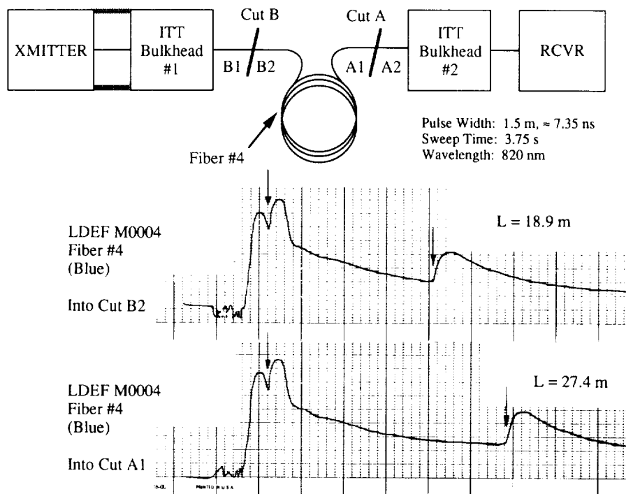
Optical time domain reflectometry analysis of impactor location on WL EXP 701 fiber optic Link #4
