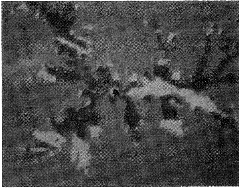
FIGURE 7. Optical micrograph showing a dendrite on zinc sulfide/aluminum oxide design (sample #3).
