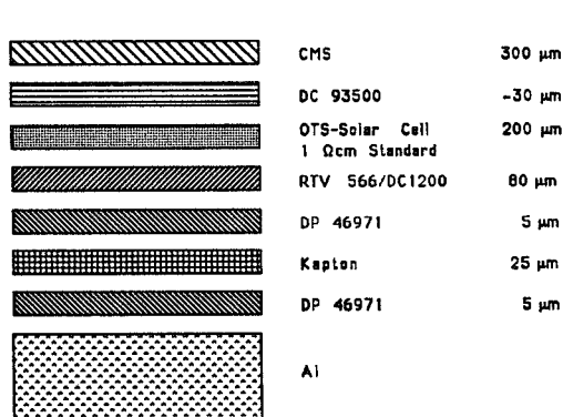
Figure 11: Configuration OTS solar cell module
