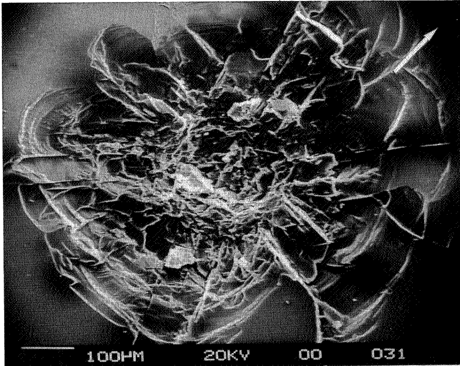
Figure 3. Scanning Electron Microscope Photograph Of The Impact Crater From A Micrometeoroid Collision With A Large-Area Silicon Infrared Detector. The Arrow Indicates Flight Direction. No Measurable Changes In Junction Leakage Or Capacitance Were Found In These Devices (Photo by Dr. John Sparrow).
