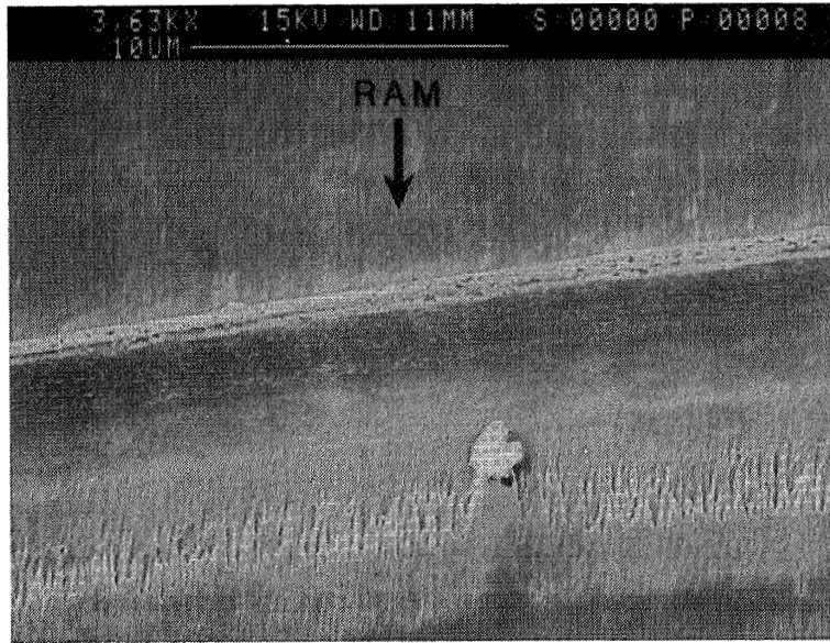
Figure 4. Uncoated Kapton flown on LDEF showing shadowing of the surface behind a particle.
