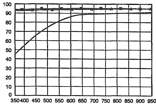
SPECTRAL TRANSMISSION OF UNCOATED ULE™ SAMPLE
