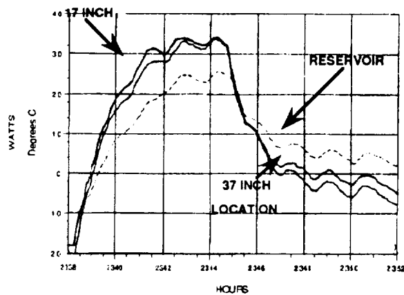
Figure 9. Unit B Evaporator
