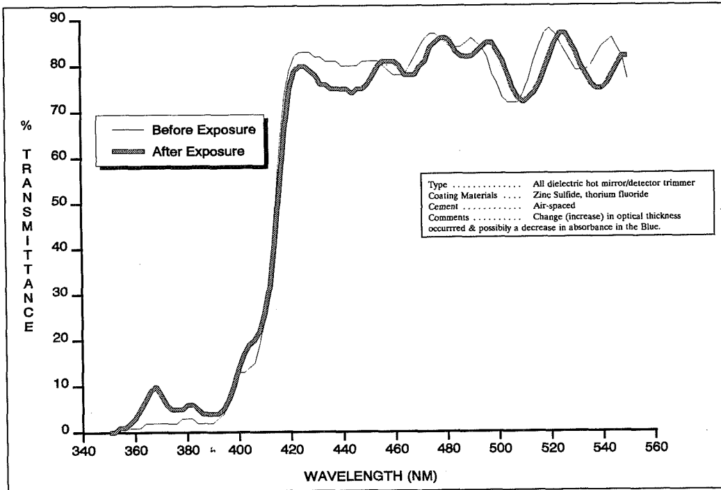
LDEF Filter No. 6
