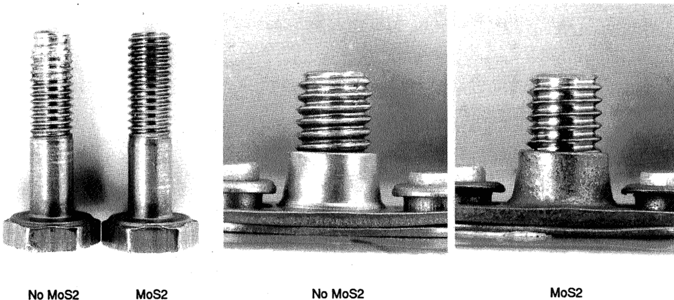
Figure 7. (Left) - Comparison of Thread Conditions of AO175 Tray Bolts Removed From Nut Plates. Undisturbed Assemblies Were Cross-Sectioned as Shown in Figure 8. Note Thread Galling Damage on Fastener That Had MoS2 Removed (Center).
