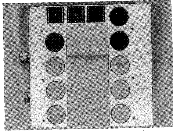
Figure 4: Coatings/solar cells experiment
