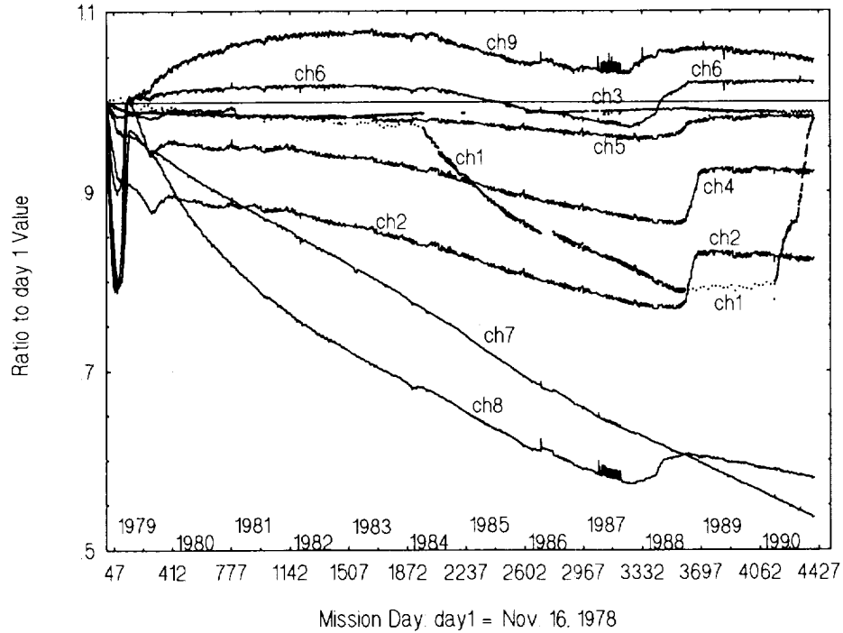
Figure 1. Daily data from 9 solar sensing channels of the Nimbus 7 ERB experiment normalized to the first day value for a 12 year period, Nov. 16, 1978 to Nov. 30, 1990
