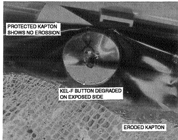
FIGURE 20. PROTECTED EDGE OF MLI BLANKET
