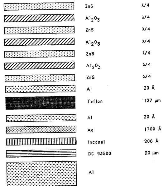
Figure 5: Configuration SSM/IF
