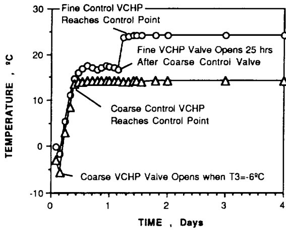
FIGURE 8. EXPERIMENT START-UP TRANSIENT
