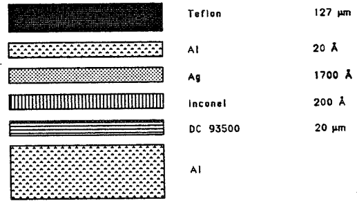
Figure 7: Configuration SSM
