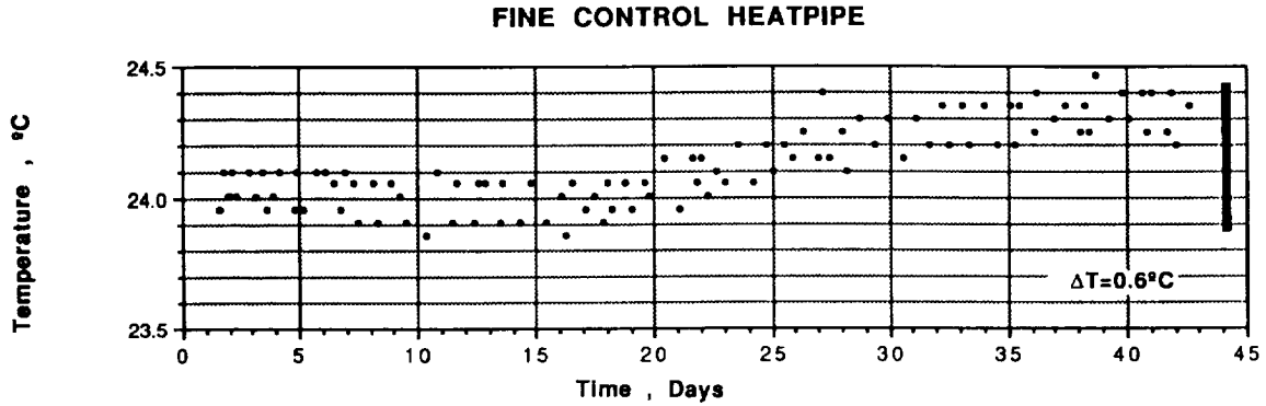
FIGURE 13. FINE CONTROL VCHP TEMPERATURE DATA
