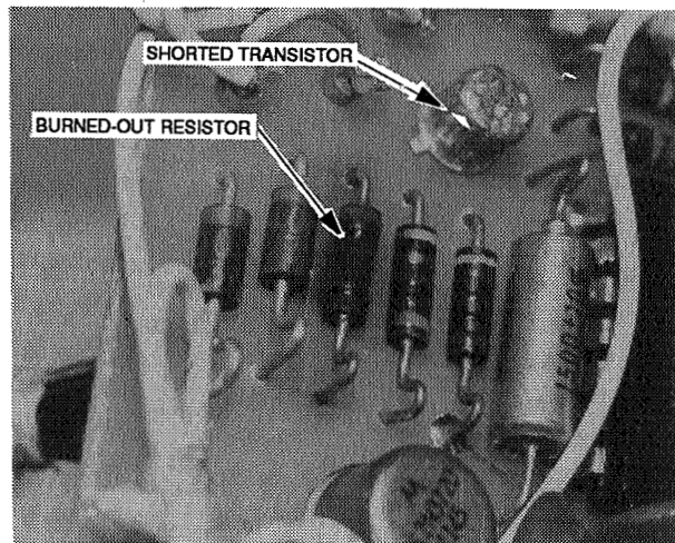
FIGURE 25. FAILED ELECTRONICS COMPONENTS IN VI CIRCUIT
