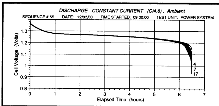
Figure 16: Pre-flight Capacity Discharge
