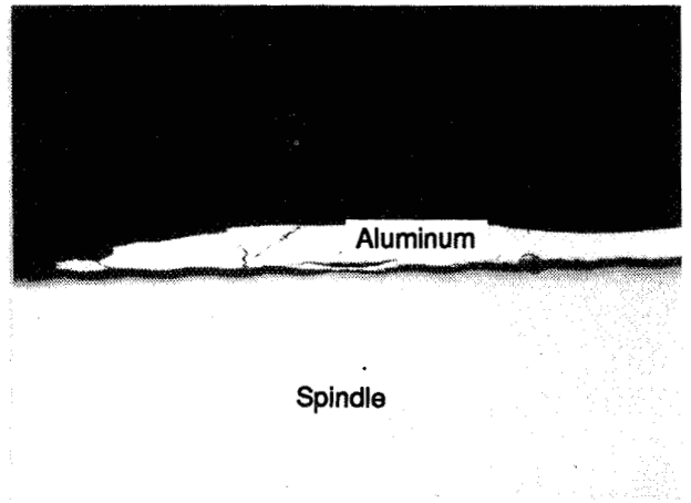
Figure 12. Galling and Adhesion of ESB Aluminum on Spindle
