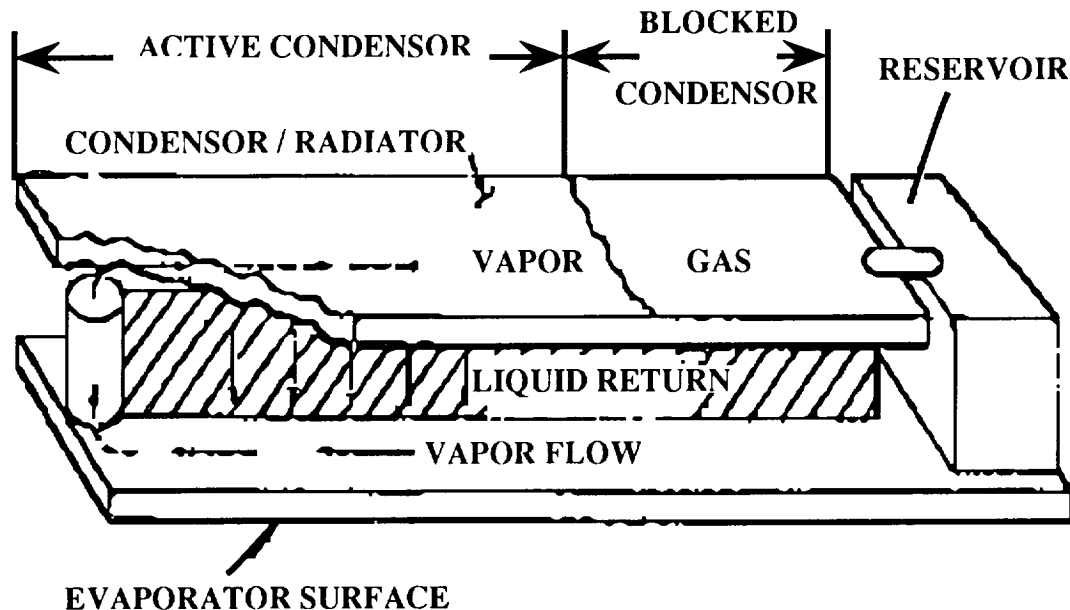
Figure 2. Liquid/Vapor Flowpaths
