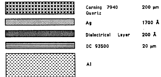
Figure 8: Configuration OSR
