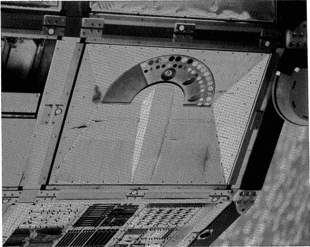
Figure 7 - TCSE Condition during LDEF Retrieval
