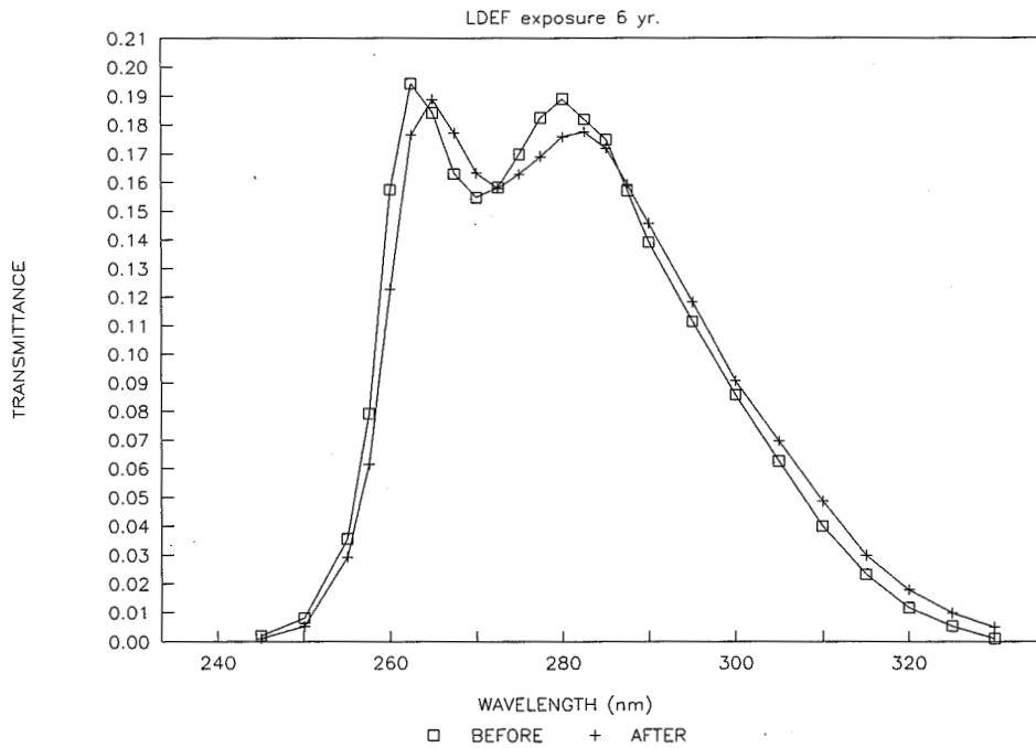
Figure 12. Spectral transmittance of interference filter 10S
