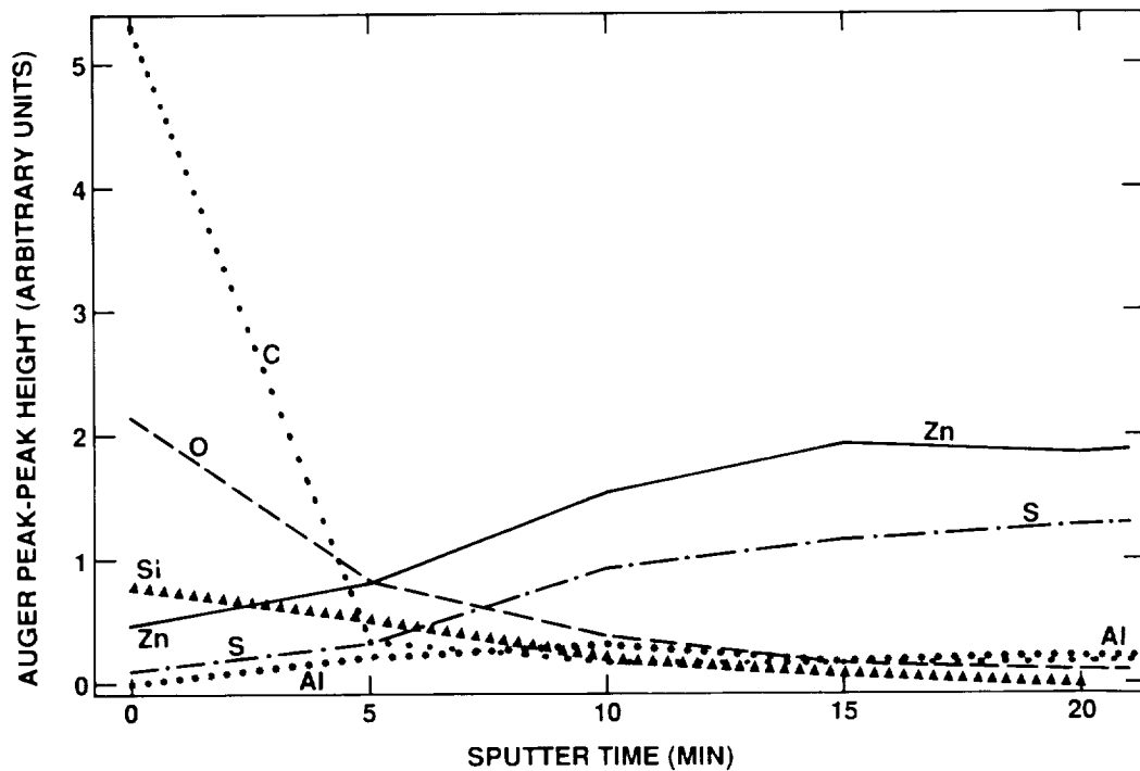
FIGURE 5. Enlargement of the surface region of data from figure 4 showing possible 200-300Å oxide layer.
