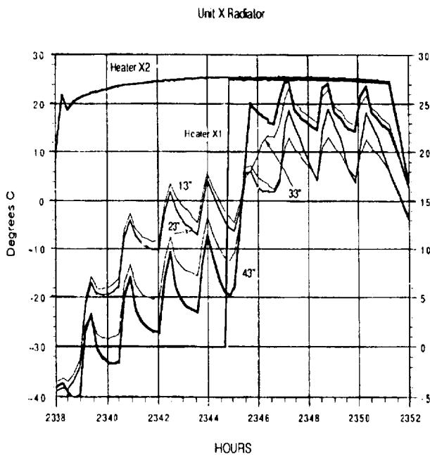
Figure 10. Unit X Radiator
