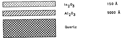
Figure 14: Configuration QCM(In 2 O 3 )
