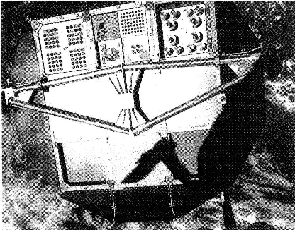
Fig.1 View on the side- (above) and the earth-tray (below) of the LDEF-satellite in orbit with BIOSTACK-units, containing thousands of Arabidopsis seeds and of Sordaria spores.
