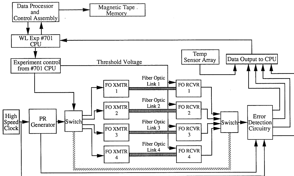
Configuration of experiment hardware used to measure the performance of the four active digital optic links contained in WL Experiment #701 (M0004). The experiment measured the temperature at various locations within the tray volume and the performance of the fiber optic links by measuring the Signal-to-Noise Ratio and Bit-Error Rate of each link.
