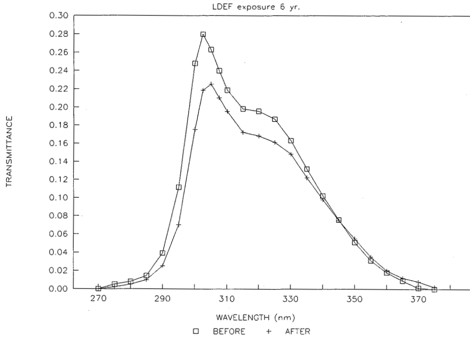
Figure 11. Spectral transmittance of interference filter 9S
