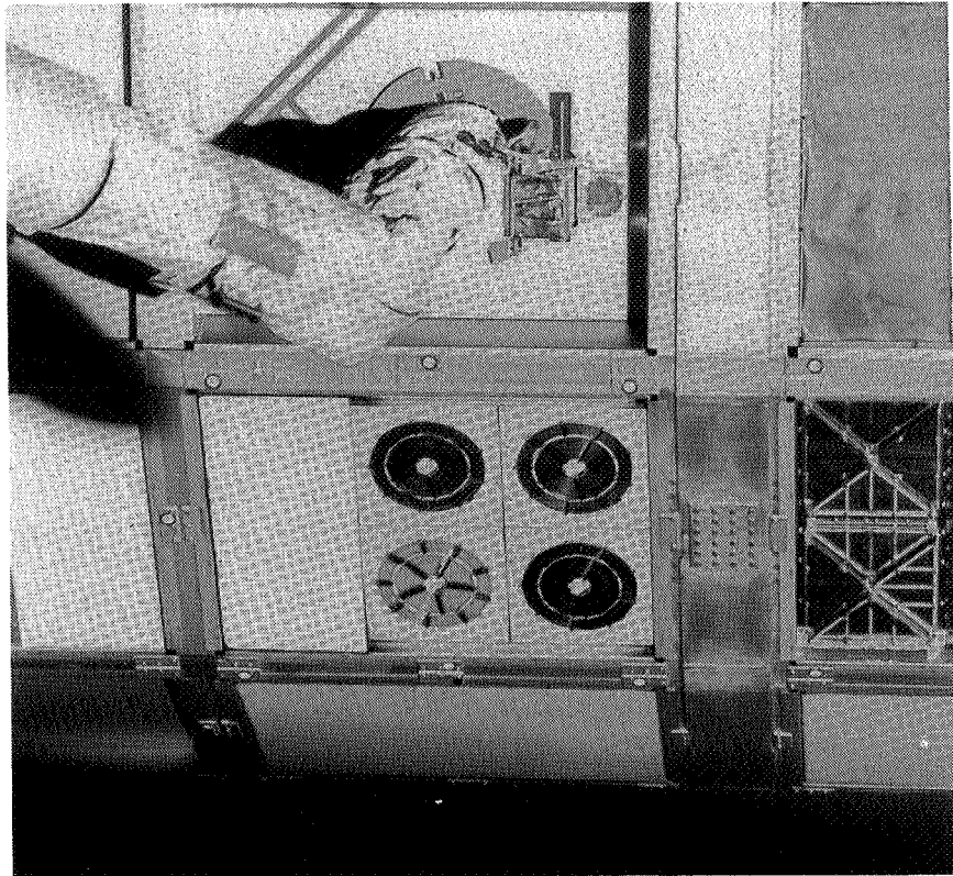
Figure 1. A photograph of the complete tray mounted on LDEF, taken during the retrieval by STS-32 in January 1990 (Courtesy of LDEF Project Office).
