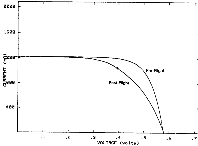
Figure 4 - ILLUMINATED PERFORMANCE OF CELL M-9
