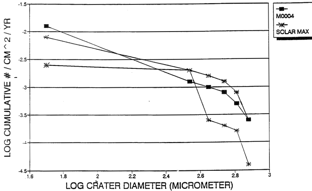
Figure 7b. Comparison [9] of WL EXP and Solar Max Satellite impactor flux data
