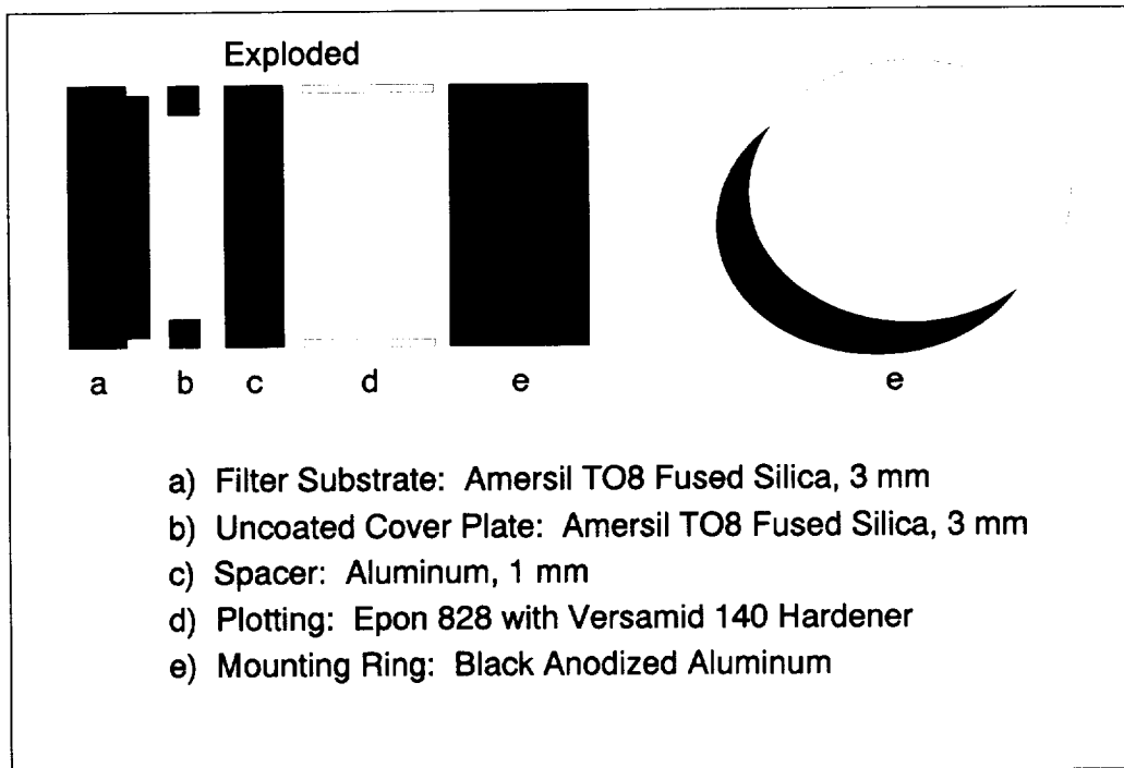
LDEF Filters, Air-Spaced Construction
