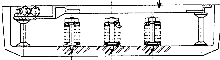
Layout of the 8 washer "spools" within the box.
