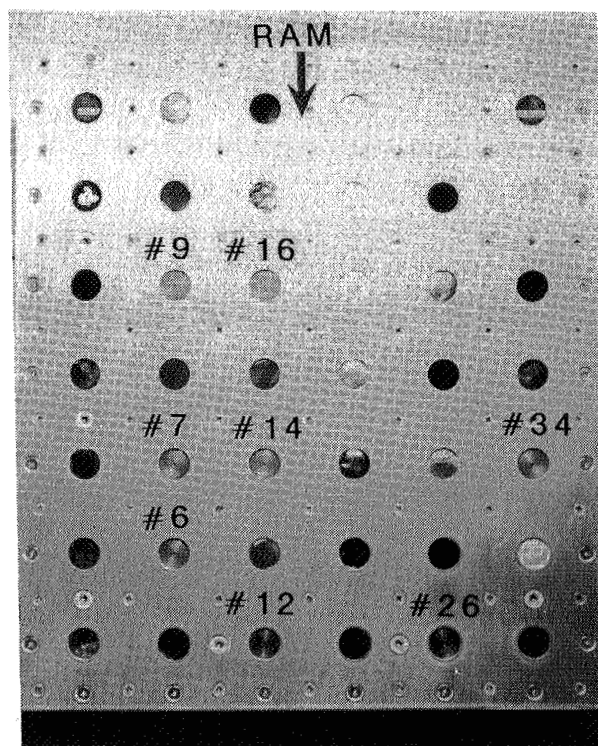
Figure 1. Location of LDEF tray in relation to the directed ram atomic oxygen arrival direction.
