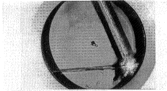
B8-2 Calcium Fluoride Substrate (Uncoated) Micrometeorite impact has caused cleaving of the substrate. crater consists of finely shattered material containing no residual debris.
