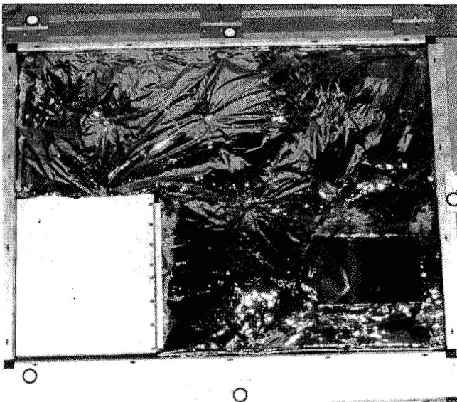
FIGURE 18. CVCHPE EXPERIMENT AFTER FLIGHT
