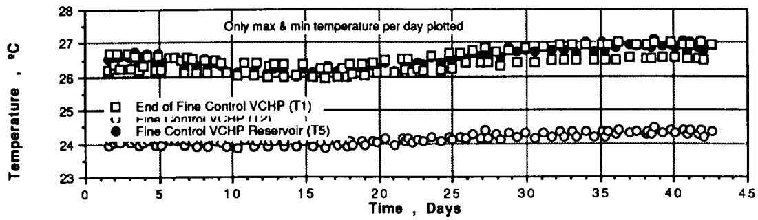
FIGURE 13. FINE CONTROL VCHP TEMPERATURE DATA
