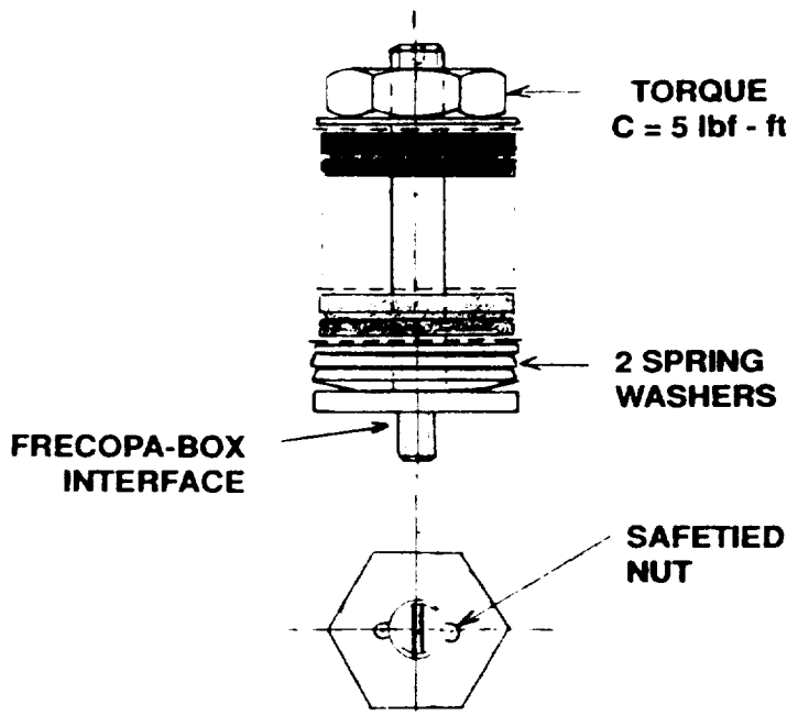
Final spool assembly
