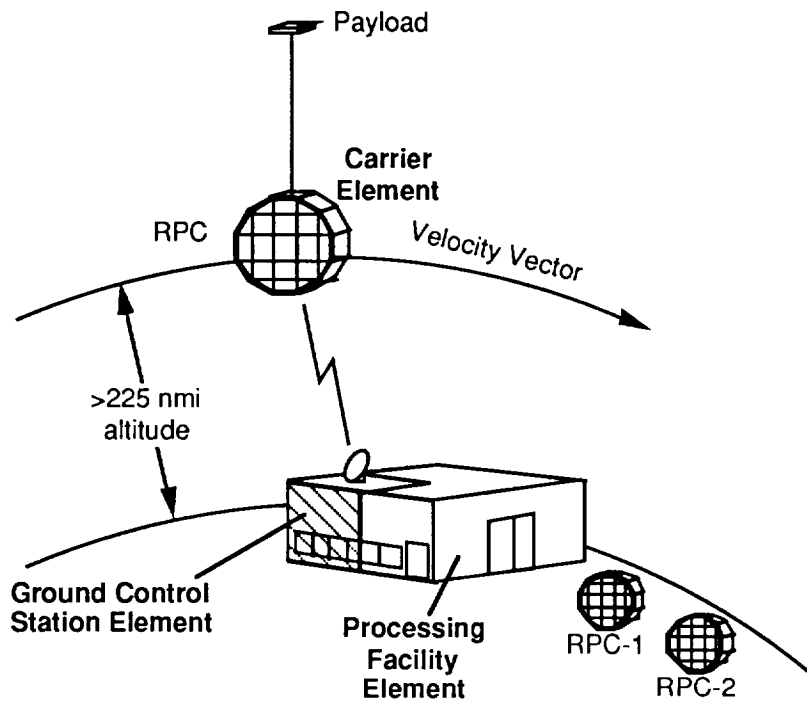
Figure 1. Retrieval Payload Carrier Program Elements
