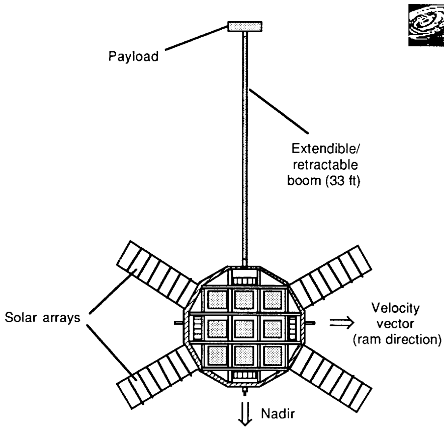
Figure 5. Deployed RPC
