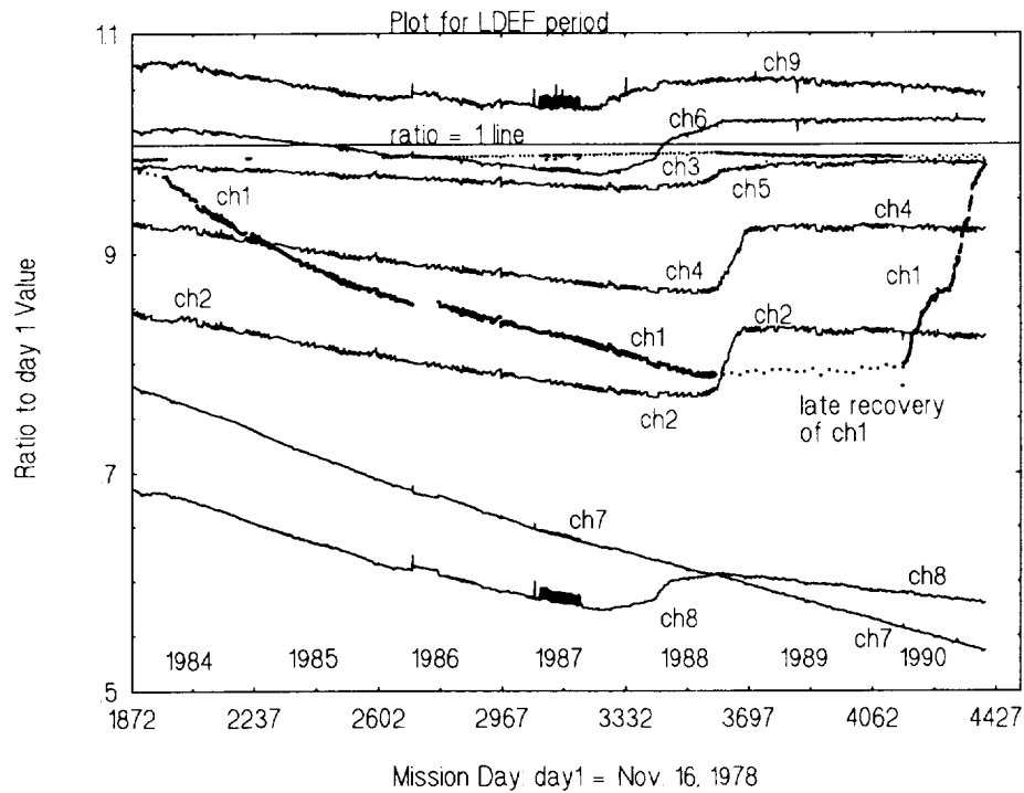
Figure 2. Normalized daily data as in Figure 1. for the period of the LDEF mission, 1984-1990. The cleaning effect of the onset of solar cycle 22 is shown.
