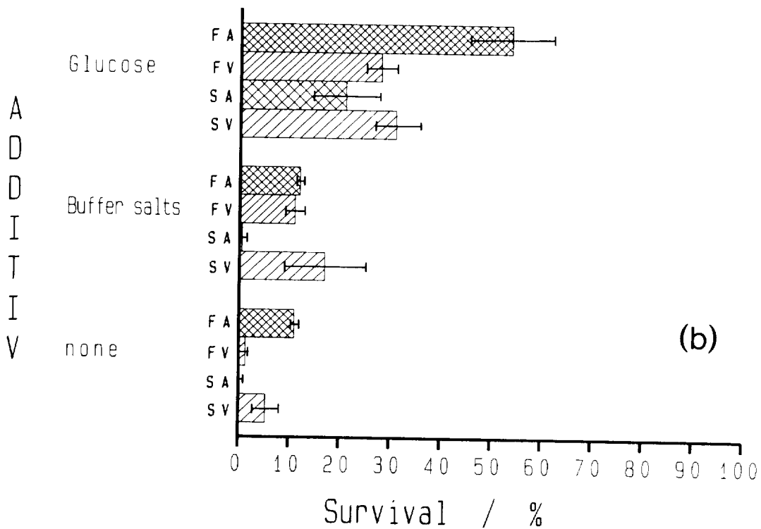
Fig. 2. Survival of Bacillus subtilis spores in multilayers (a) or in a monolayer (b) after nearly 6 years in space during the LDEF mission and ground control data. The spores were shielded against solar optical radiation. Protective substances (5 % glucose or 1.4 % buffer salts) were added to some of the samples during preparation. F = flight samples; S = samples of the simulation experiment on ground; A = samples kept at atmospheric pressure; V = samples in vacuum.
