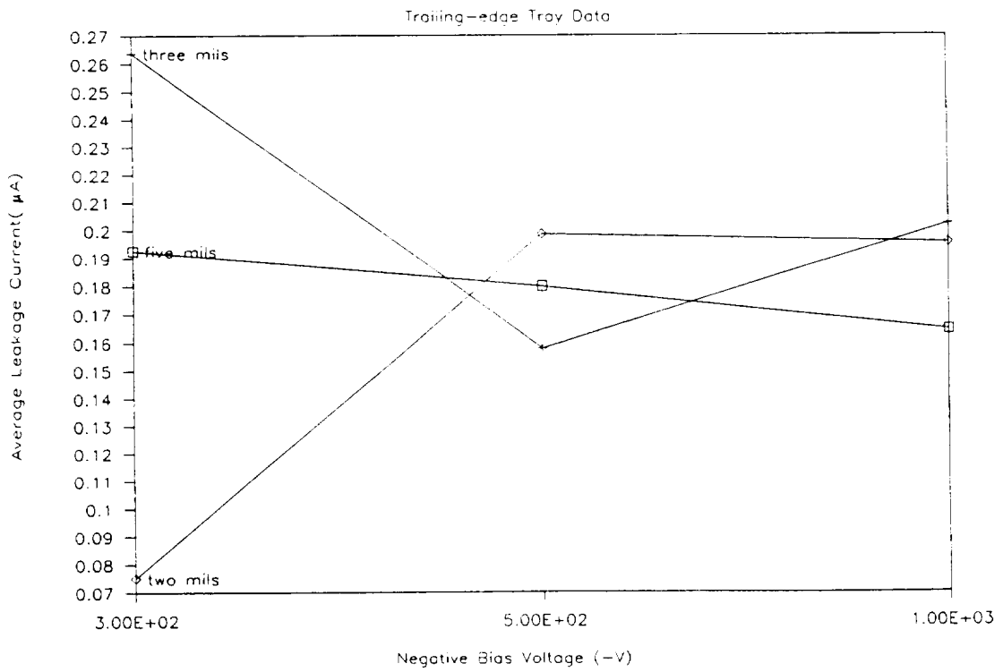
Figure 5. LDEF Average Leakage Currents Collected at the Negatively Biased Samples for Both TRW Trays.
