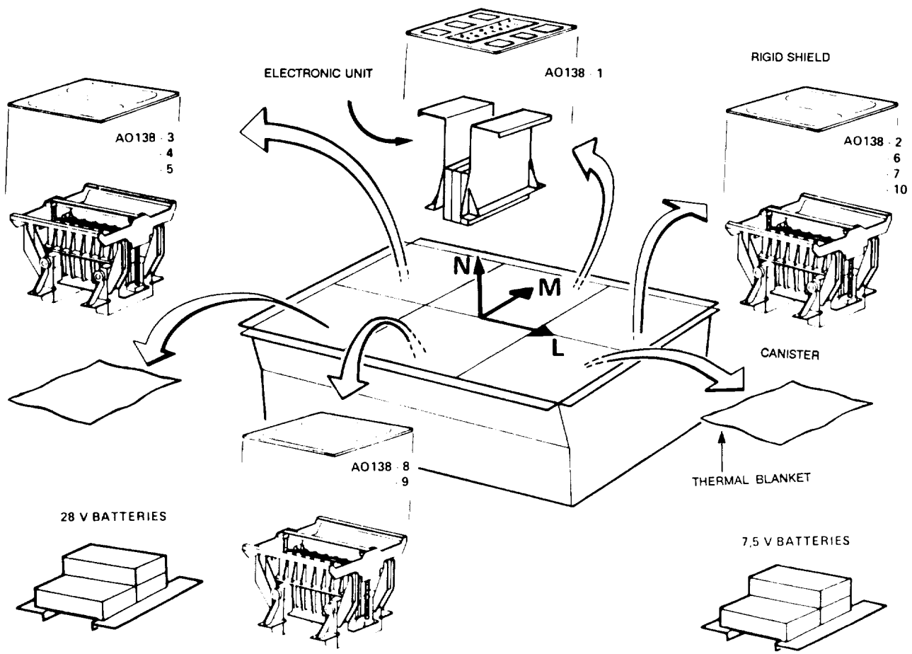
Fig. 2. EXPLODED VIEW OF FRECOPA EXPERIMENTS AO-138
