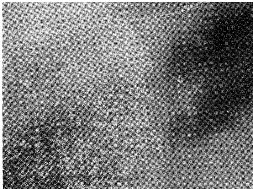
Figure 4. Photograph of MgF 2 window, back surface, 40X.
