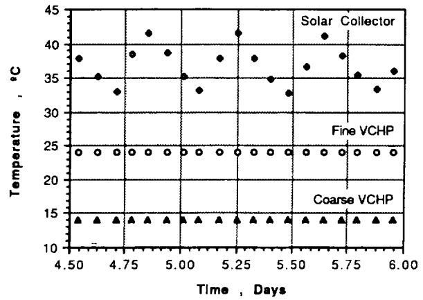
FIGURE 9. ORBITAL TEMPERATURE VARIATIONS
