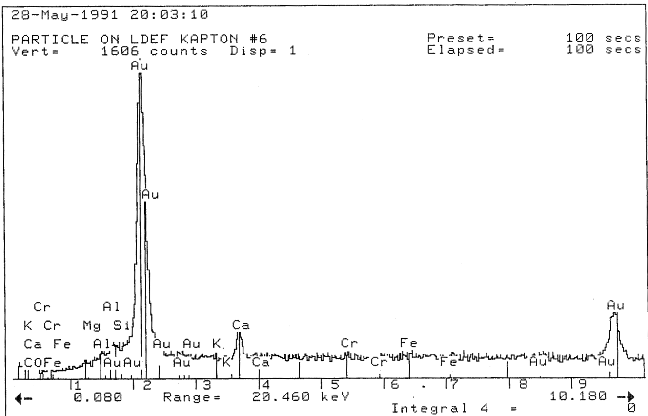
Figure 9. Energy dispersive X-ray analysis of particle left in an impact site on uncoated Kapton.
