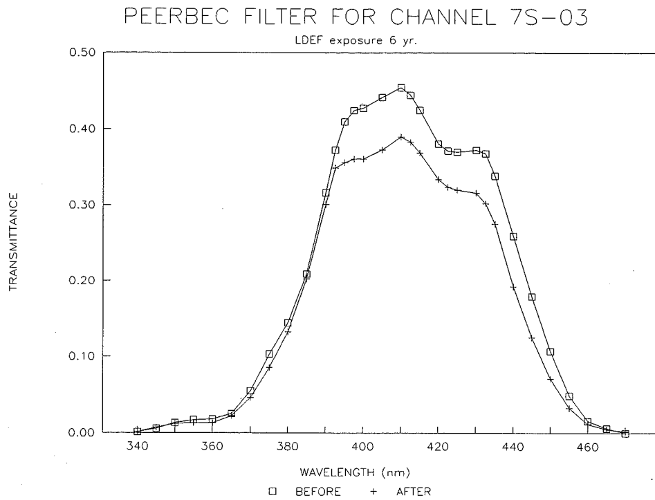
Figure 9. Spectral transmittance of interference filter 7S
