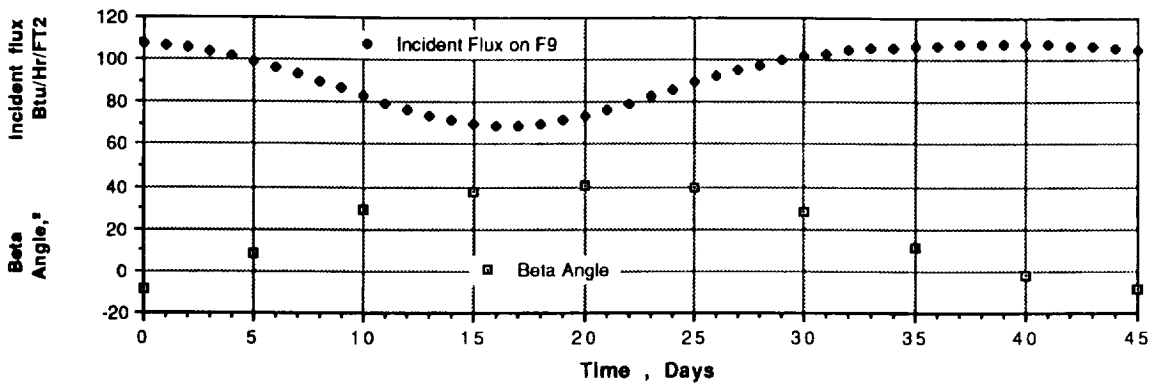
FIGURE 10. BETA ANGLE AND HEAT FLUX
