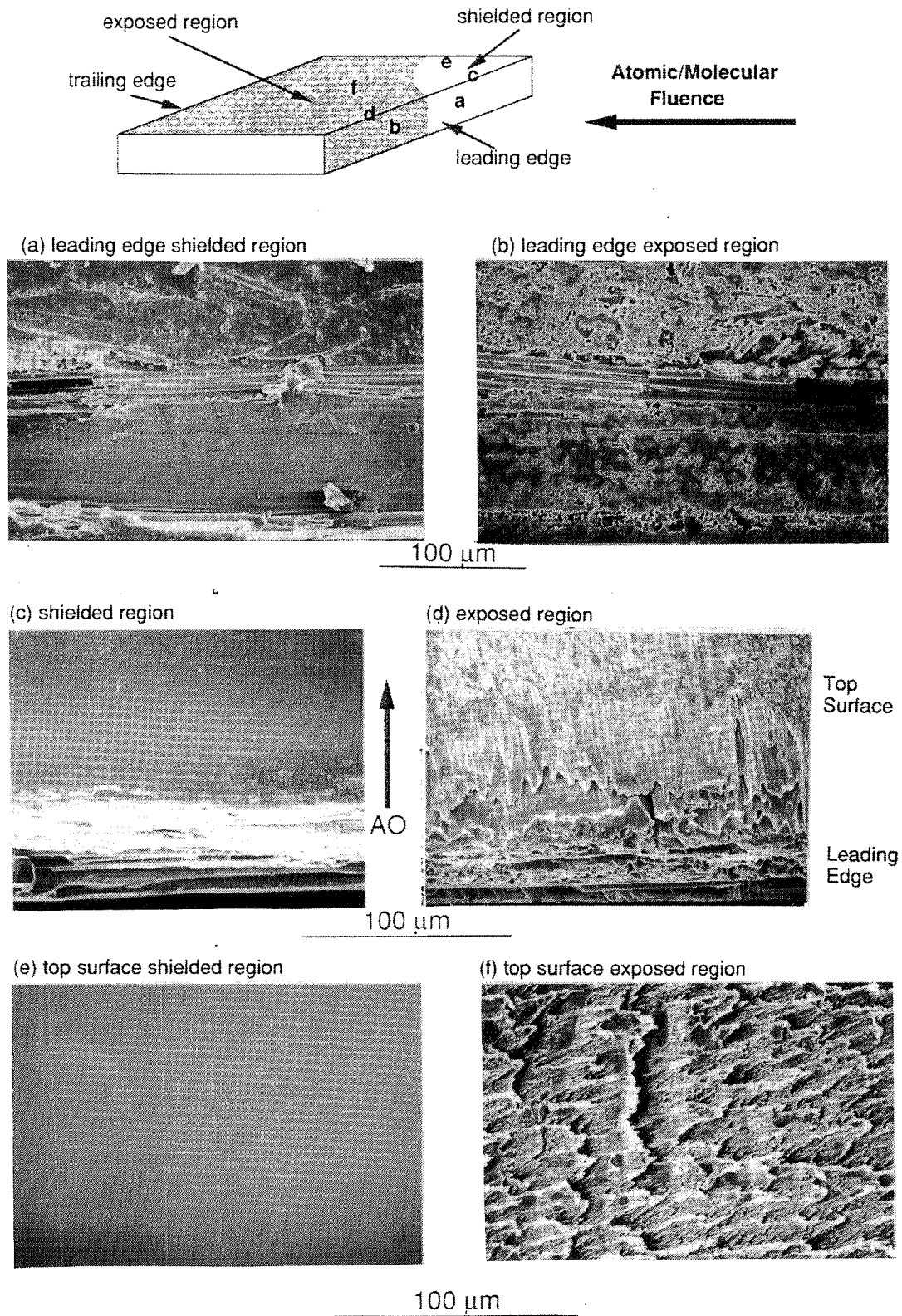
Figure 6. SEM photomicrographs of flight space glass/Kapton.
