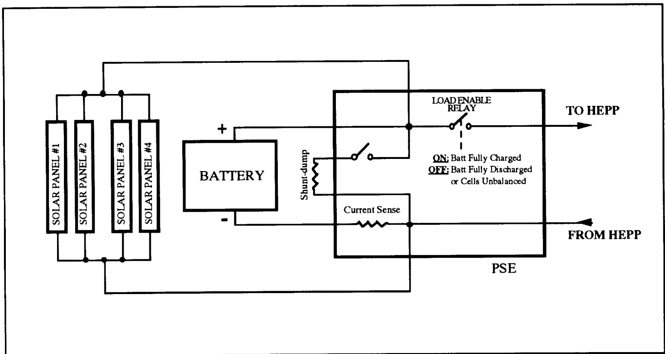
Figure 4: Block diagram of power system
