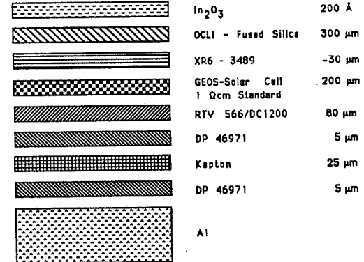
Figure 12: Configuration GEOS solar cell module
