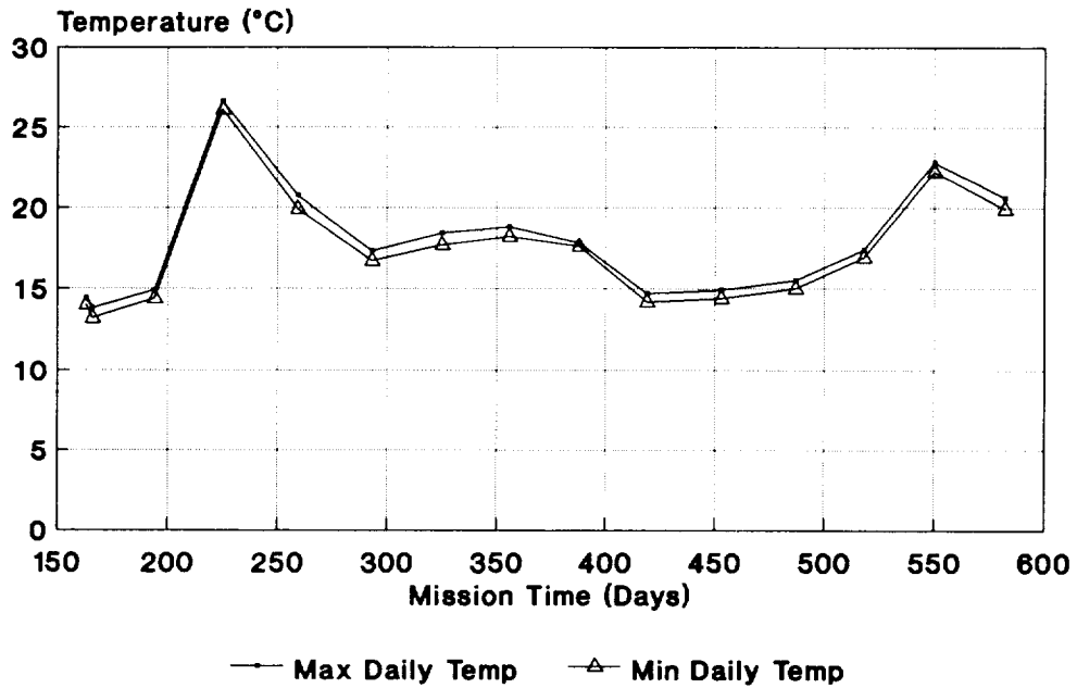
Figure 10 - Battery Temperature
