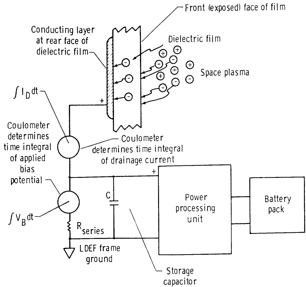
Figure 3. High Voltage Drainage Experiment Configuration.
