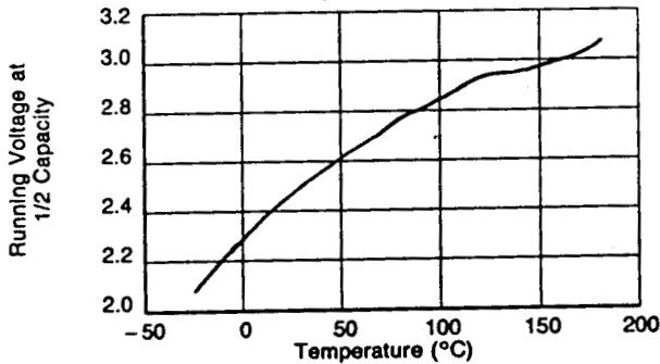
Running Voltage vs. Temperature (56 Ohm Discharge)
