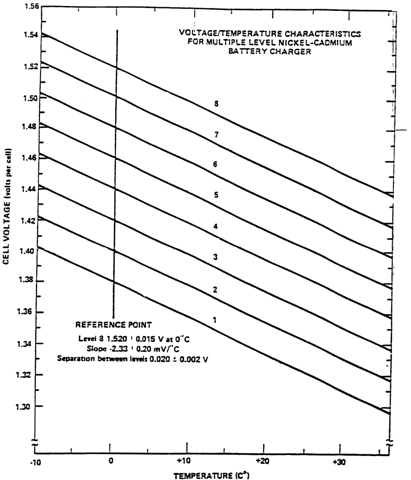
Figure 3. Cell Voltage Limit Versus Temperature
