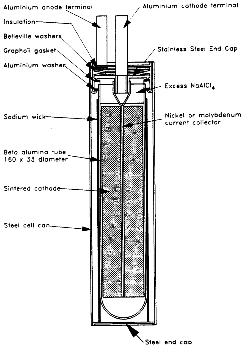
Fig. 5 PROTOTYPE SPACE SODIUM NICKEL CLORIDE CELL
