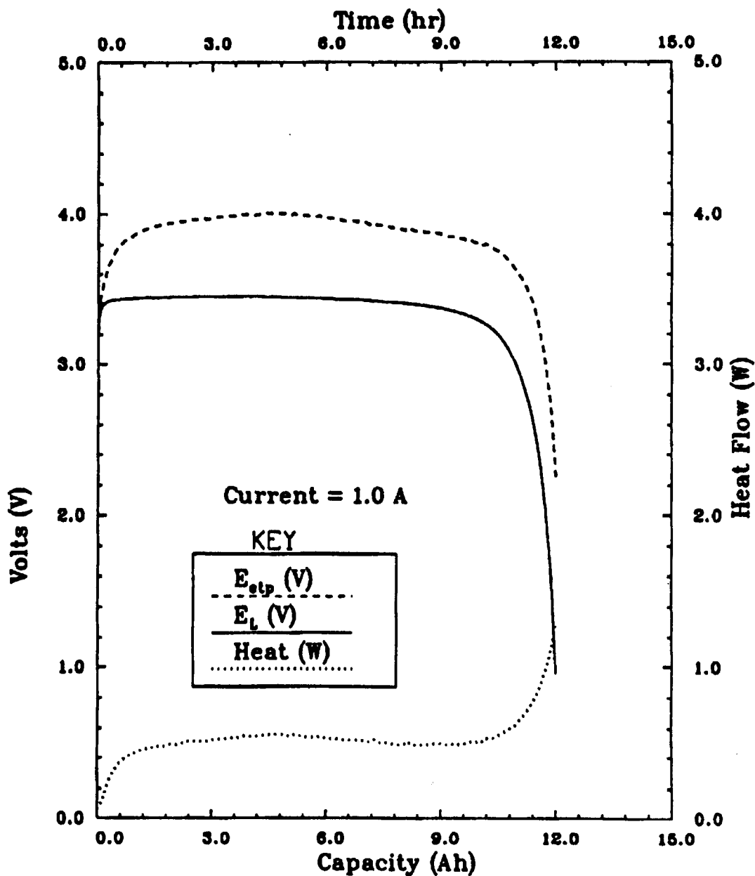
Fig. d7: Effective thermoneutral Potential, load voltage and rate of heat generation for a Li/SOCl 2 cell at 60° C.
