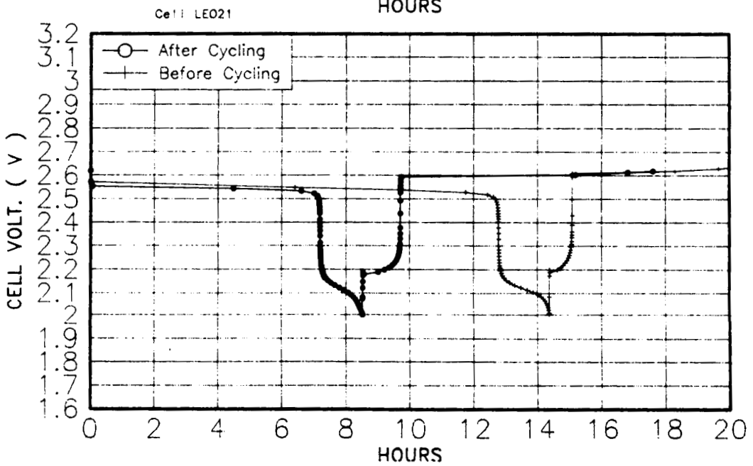
Fig. 8 CELL CAPACITY AT 1 A RATE BEFORE & AFTER 2810 CYCLES
