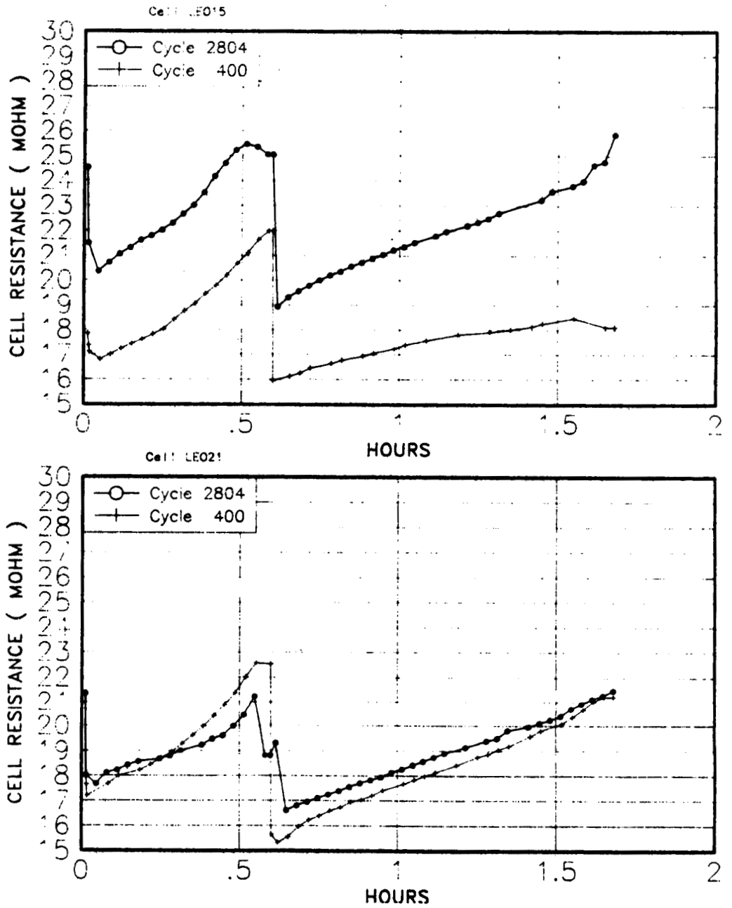
Fig. 10 CELL INTERNAL RESISTANCE DURING LEO CYCLES
