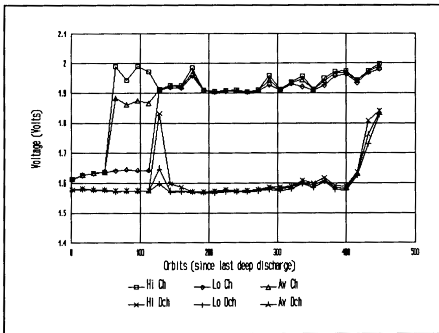
Figure 12 -- EOC/EOD Hi/Lo/Av cell voltages vs. orbits (since last deep discharge) during the 11th month of LEO cycling for pack 4.
