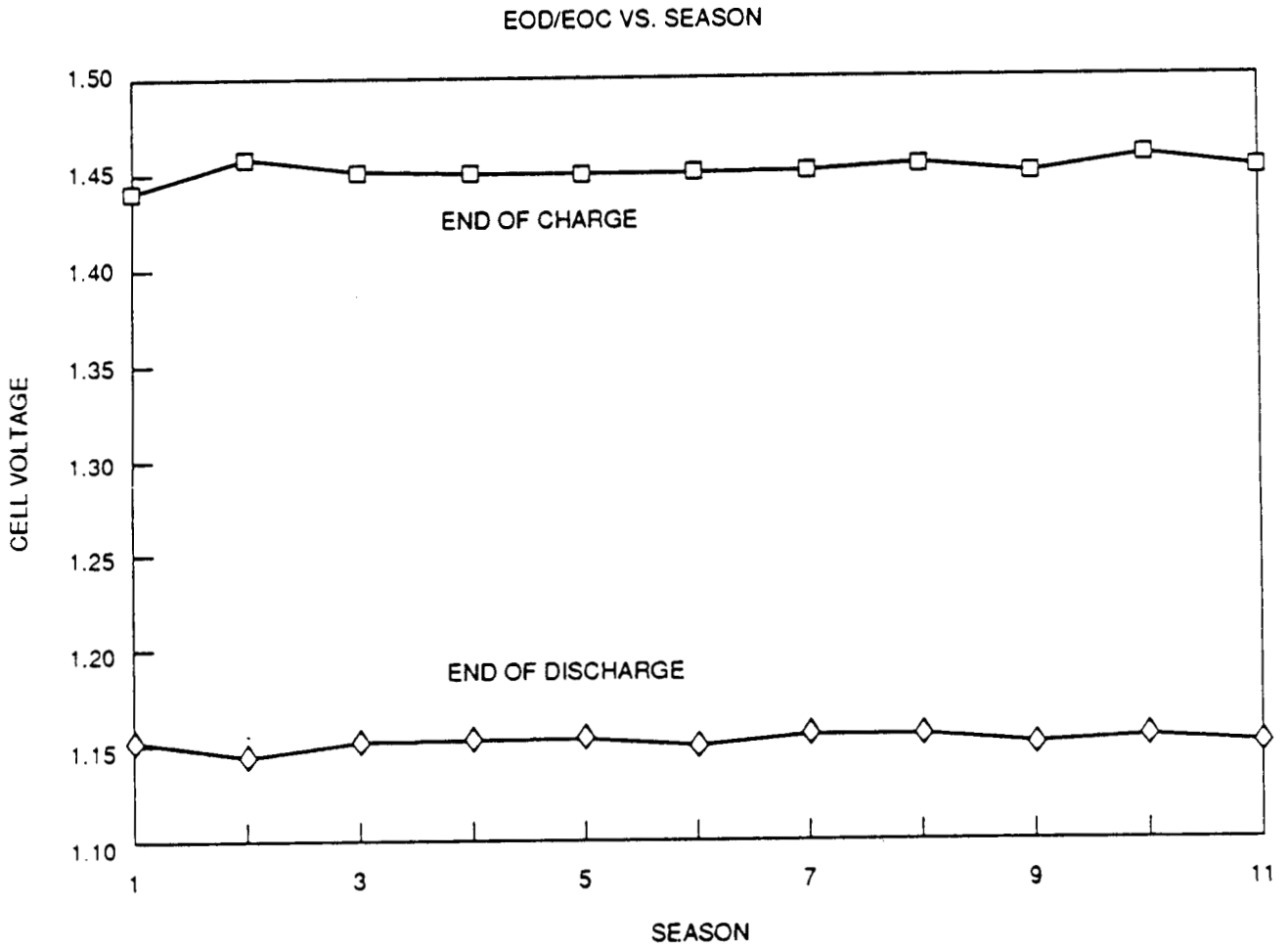
Figure 4 BSB life test realtime eclipse season 14-day solstice test temperature 10^{\circ} \pm 3^{\circ}C .
