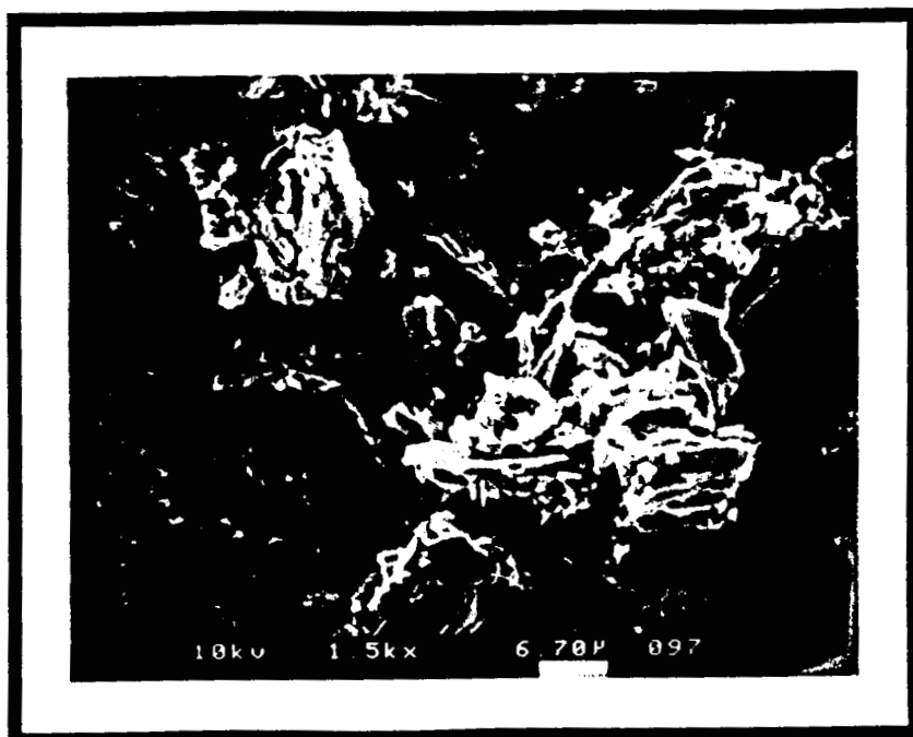
RT Reaction Product From Li/1M LiAsF 6 in DMSI (CF x ) n Hg Cell
