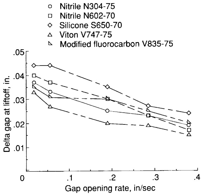
Figure 7. Resiliency behavior of candidate O-ring materials at 60°F.
