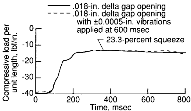
(b) Compressive load trace.
