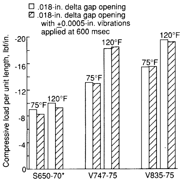
Figure 16. Residual load values of candidate materials at 23.3-percent squeeze at 75°F and 120°F.
