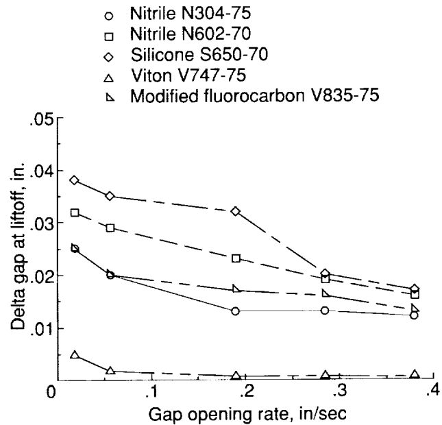
Figure 10. Resiliency behavior of candidate O-ring materials at 30°F.
