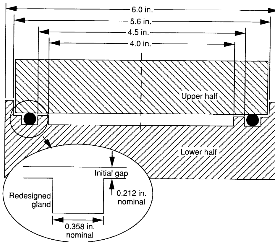
(b) Schematic of face seal fixture.
