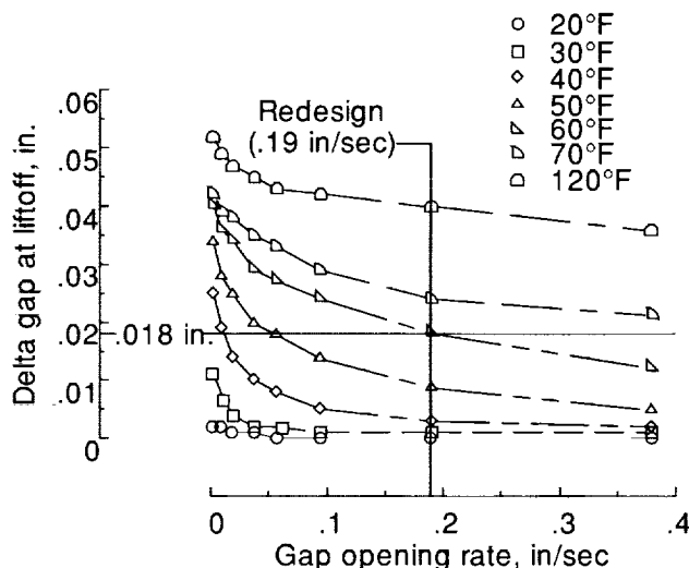
Figure 14. Viton response at redesign joint deflection and gap opening rate.
