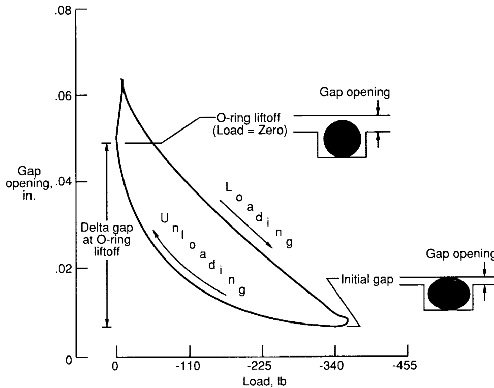
Figure 4. Format of O-ring resiliency test data.
