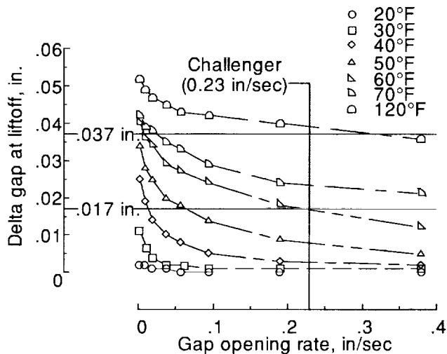
Figure 13. Viton response at Challenger's joint deflection and gap opening rate.
