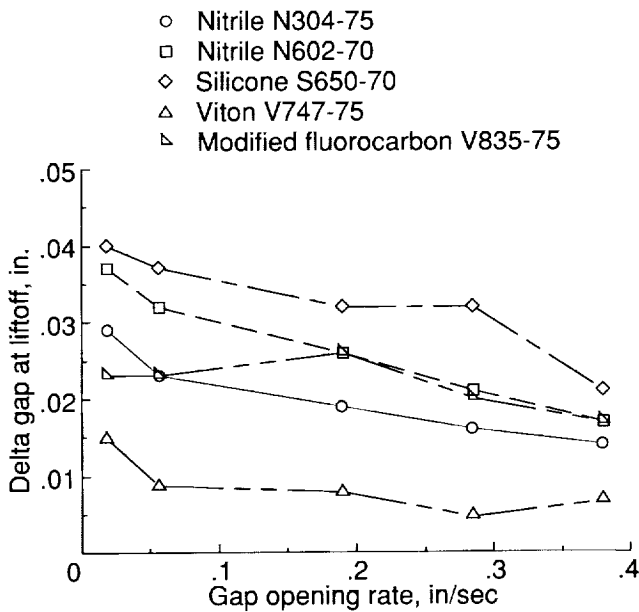
Figure 9. Resiliency behavior of candidate O-ring materials at 40°F.
