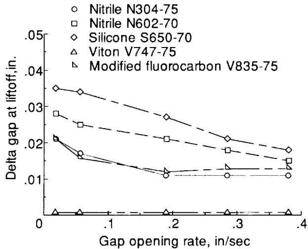
Figure 11. Resiliency behavior of candidate O-ring materials at 20°F.
