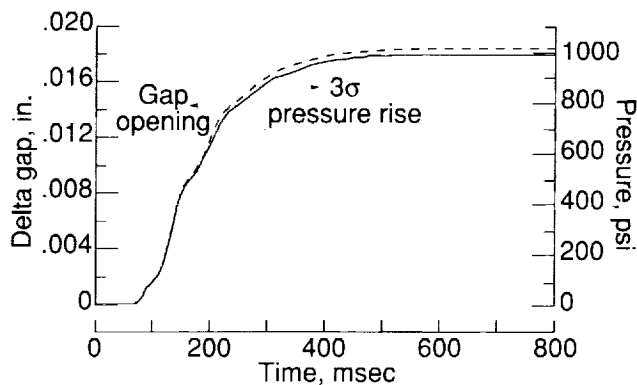
Figure 5. Displacement history and 3\sigma pressure rise for field joint deflection test.
