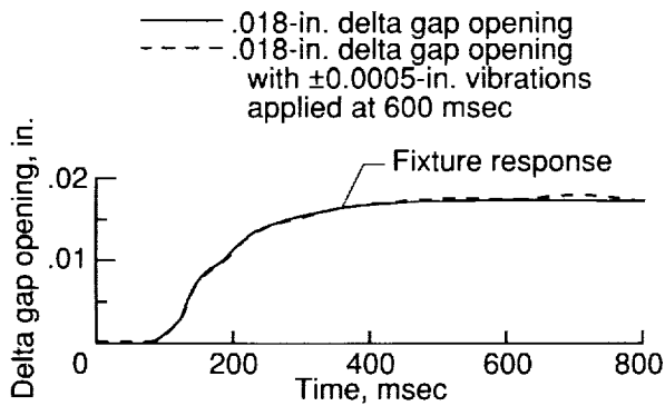
(a) Displacement response of fixture to programmed delta gap openings.
