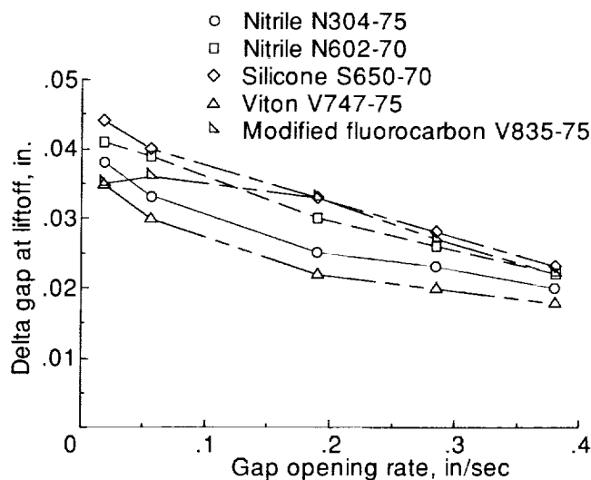
Figure 6. Resiliency behavior of candidate O-ring materials at 70^{\circ}\text{F} .
