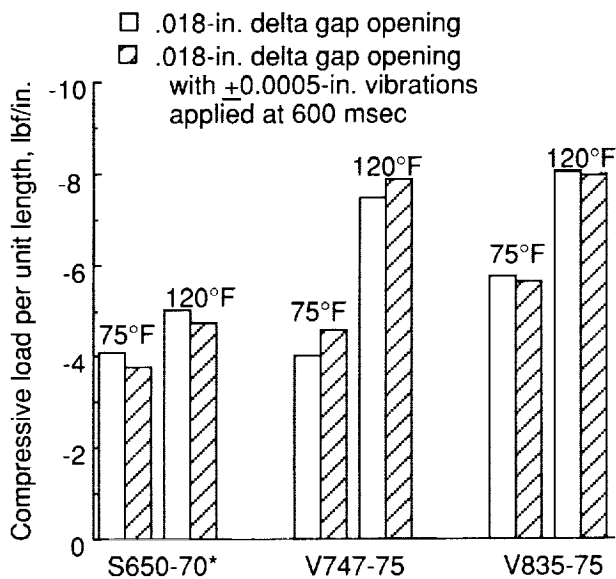
Figure 15. Residual load values of candidate materials at 16.2-percent squeeze at 75°F and 120°F.
