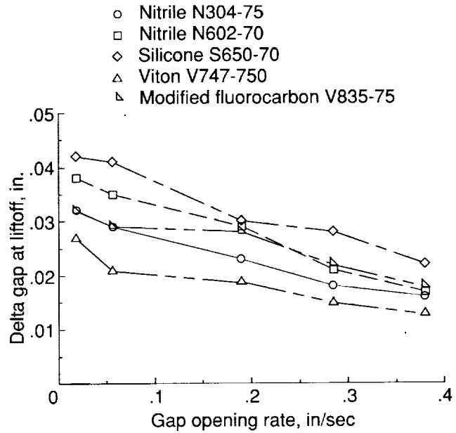
Figure 8. Resiliency behavior of candidate O-ring materials at 50°F.
