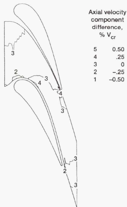
(b) Axial velocity component difference, (|V_{p,z}| - |V_{g,z}|)/V_{cr} , percent (0.5- \mu m diameter particles).
