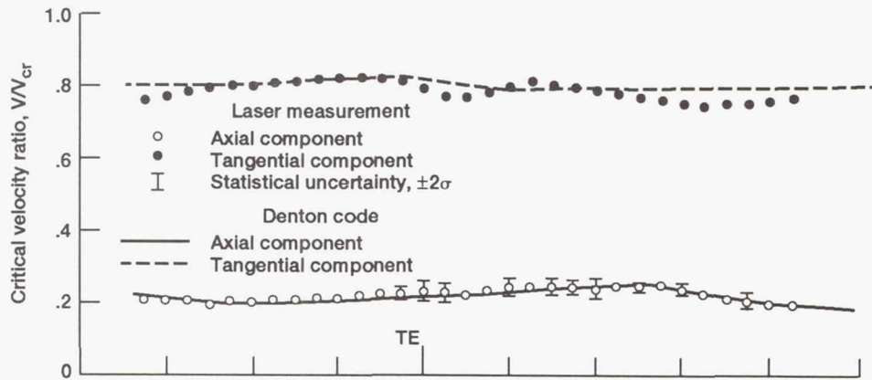
(b) Radial position, R , 50 percent of span from hub.
