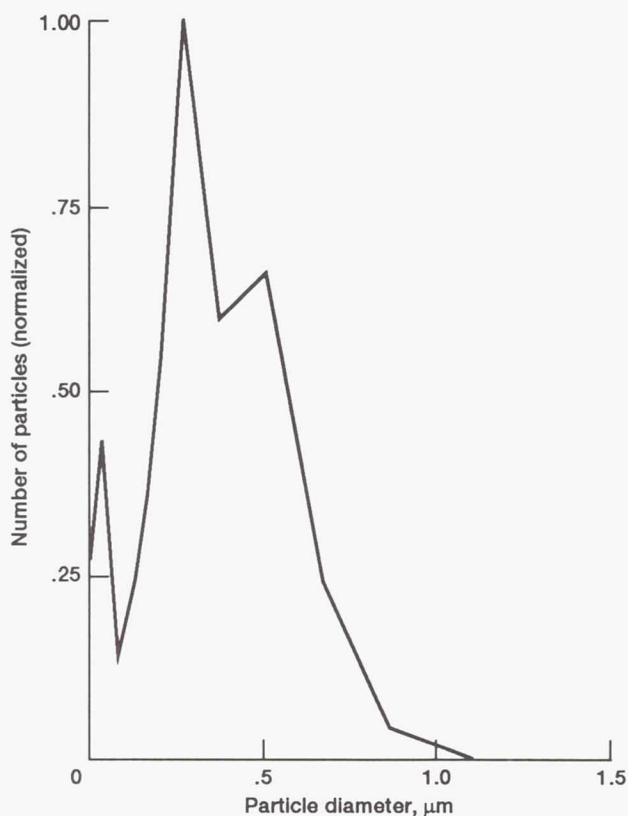
Figure 5.—Measured seed particle size distribution.
