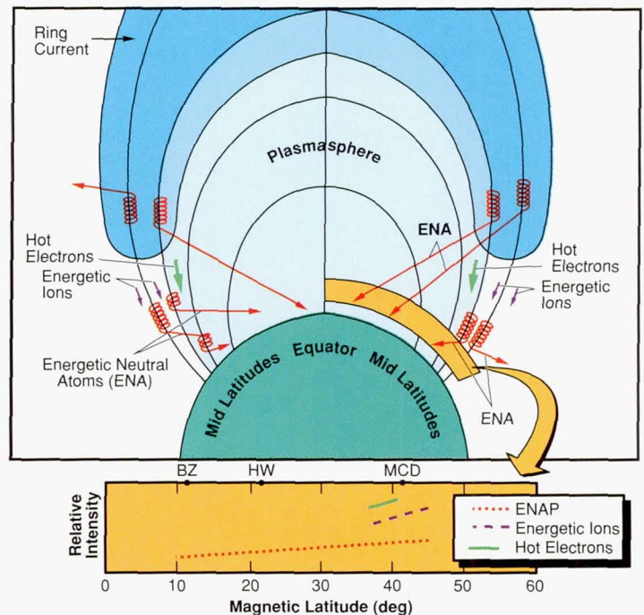
Energetic ions in the ring current are neutralized when they collide with hydrogen in the outer regions of Earth's space. When the resulting energetic atoms rain down into the thermosphere, they create low-latitude auroras that the ISO instrument will detect. The enlarged segment of the illustration charts relative intensities as recorded by ground stations in Brazil (BZ) and Hawaii (HW) and at the McDonald Observatory (MCD) in Texas.
