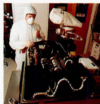
The ATMOS instrument's intricate optical equipment is checked during this preflight inspection.
