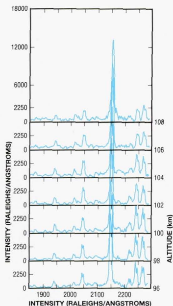
On Spacelab 1, the nitric oxide spectral signature was observed simultaneously by the ISO at 2-km (1.2-mi) intervals between 96 and 108 km (59.5 and 66.9 mi).
