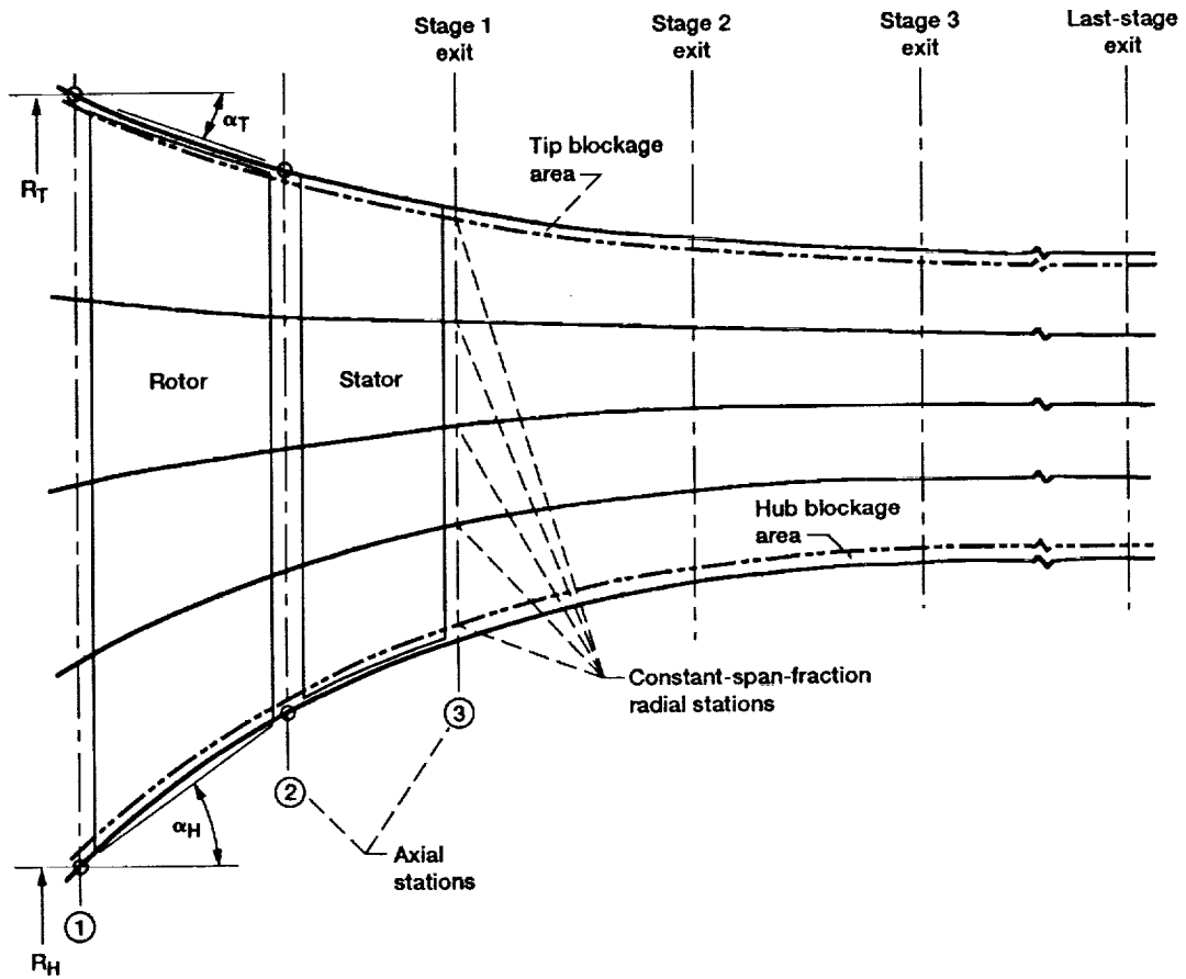
(a) Meridional flowpath.
