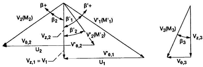
(b) Stage velocity diagram.
