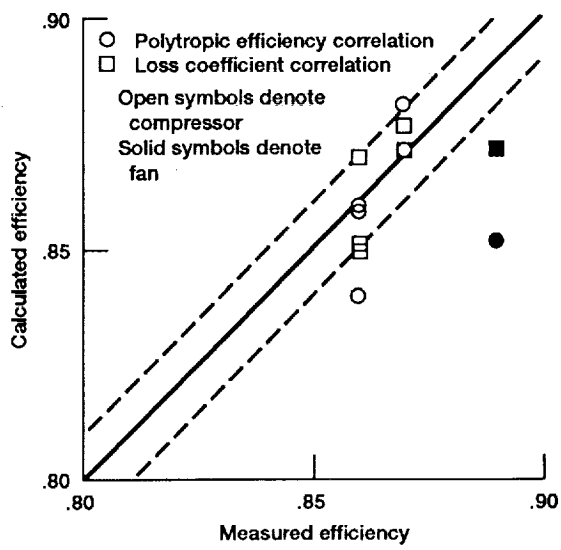
Figure 4.—Comparison of measured and calculated efficiencies.
