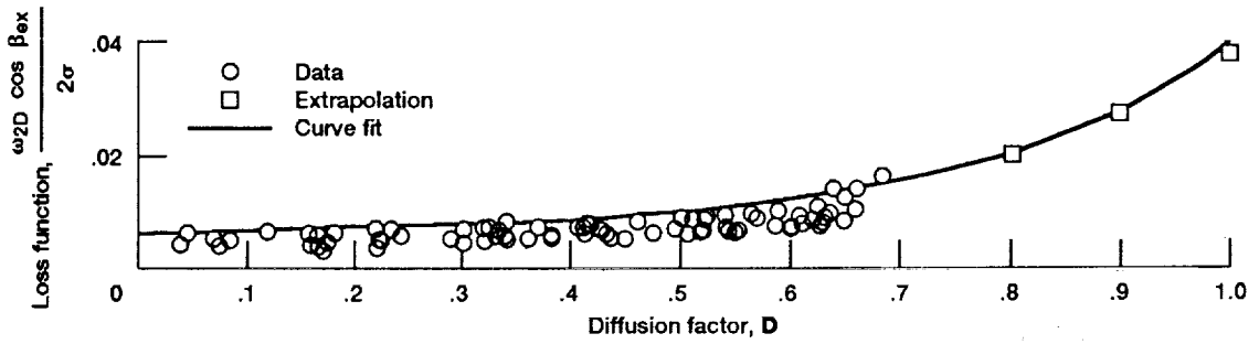
Figure 3.—Variation of loss function with diffusion factor.
