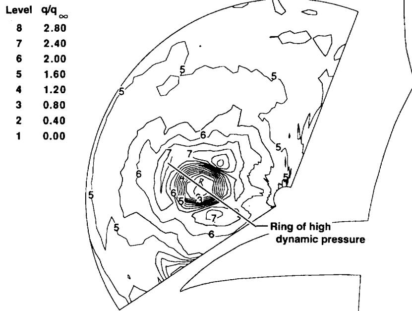
(c) Normalized dynamic pressure contours.
