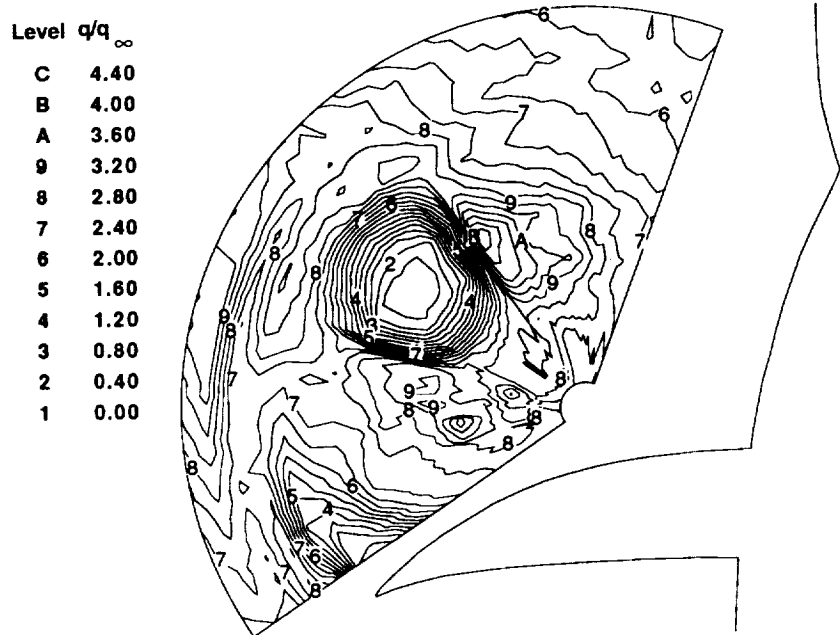
(e) Normalized dynamic pressure contours, \alpha \approx 30^\circ .
