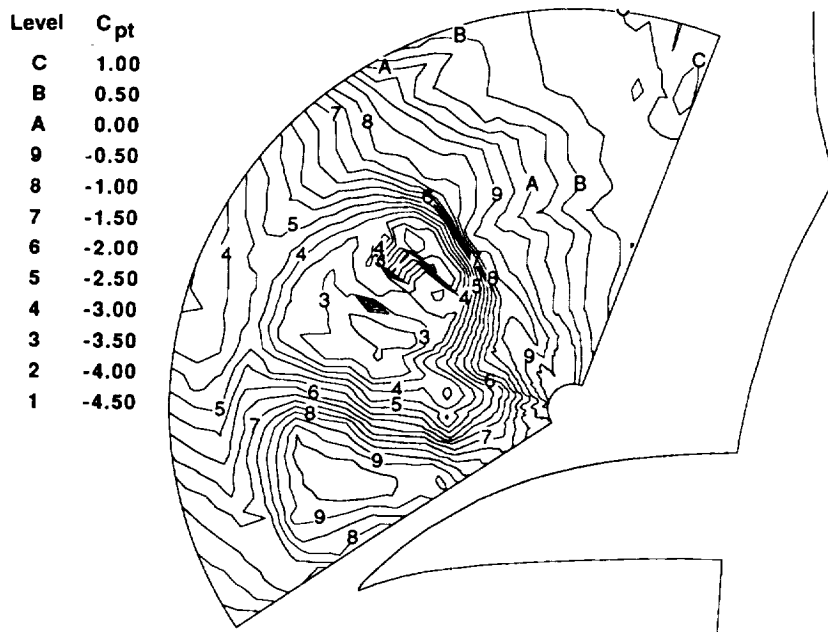
(b) Total pressure coefficient contours.
