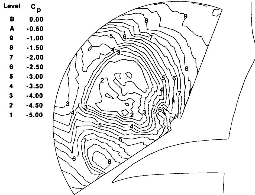
(a) Static pressure coefficient contours, flight data.
