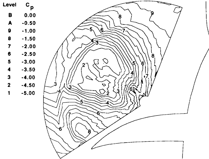
(a) Static pressure coefficient contours.
