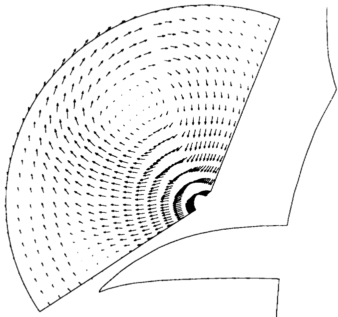
(h) Crossflow velocity vectors, \alpha \approx 36^\circ .
