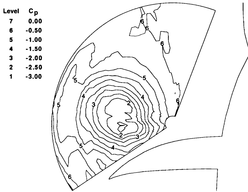
(a) Static pressure coefficient contours, flight data.
