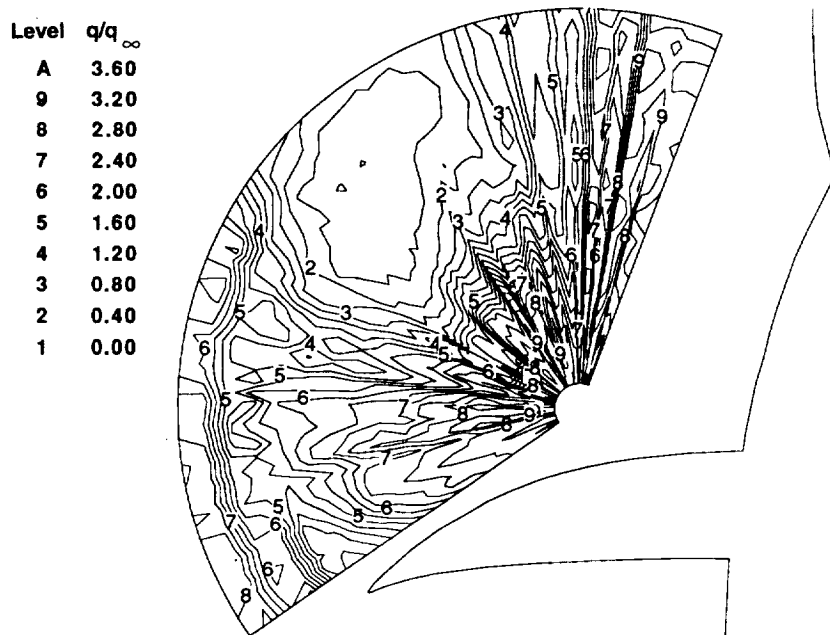
(i) Normalized dynamic pressure contours, \alpha \approx 48^\circ .
