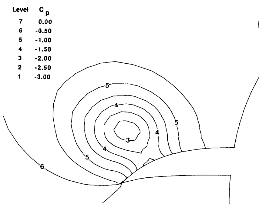
(b) Static pressure coefficient contours, computational solution.
