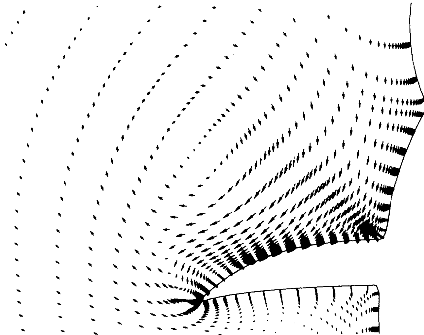
(f) Crossflow velocity vectors, computational solution.
