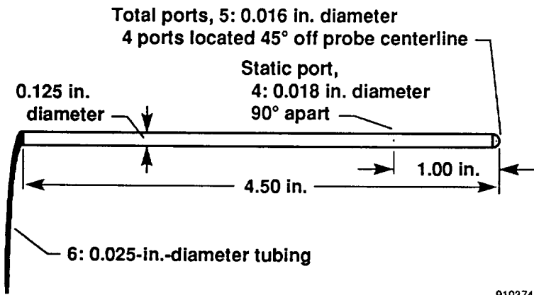
(a) Hemispherical-tipped five-hole probe.
