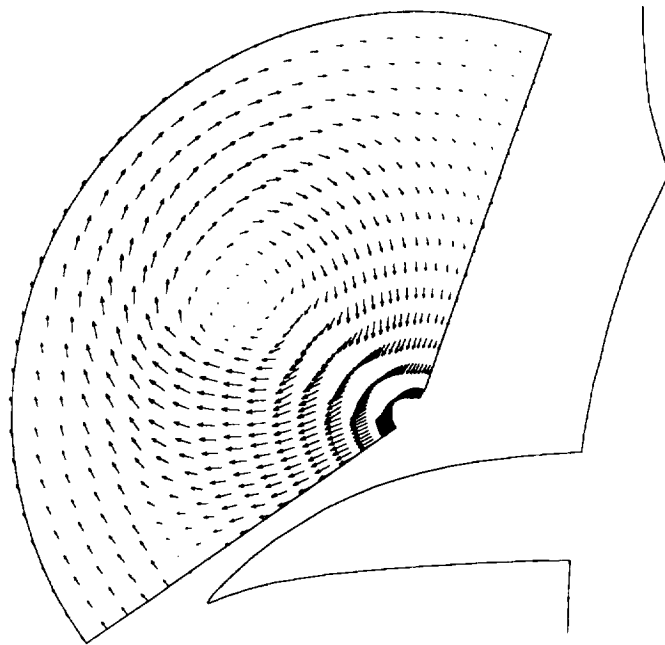
(e) Crossflow velocity vectors, flight data.
