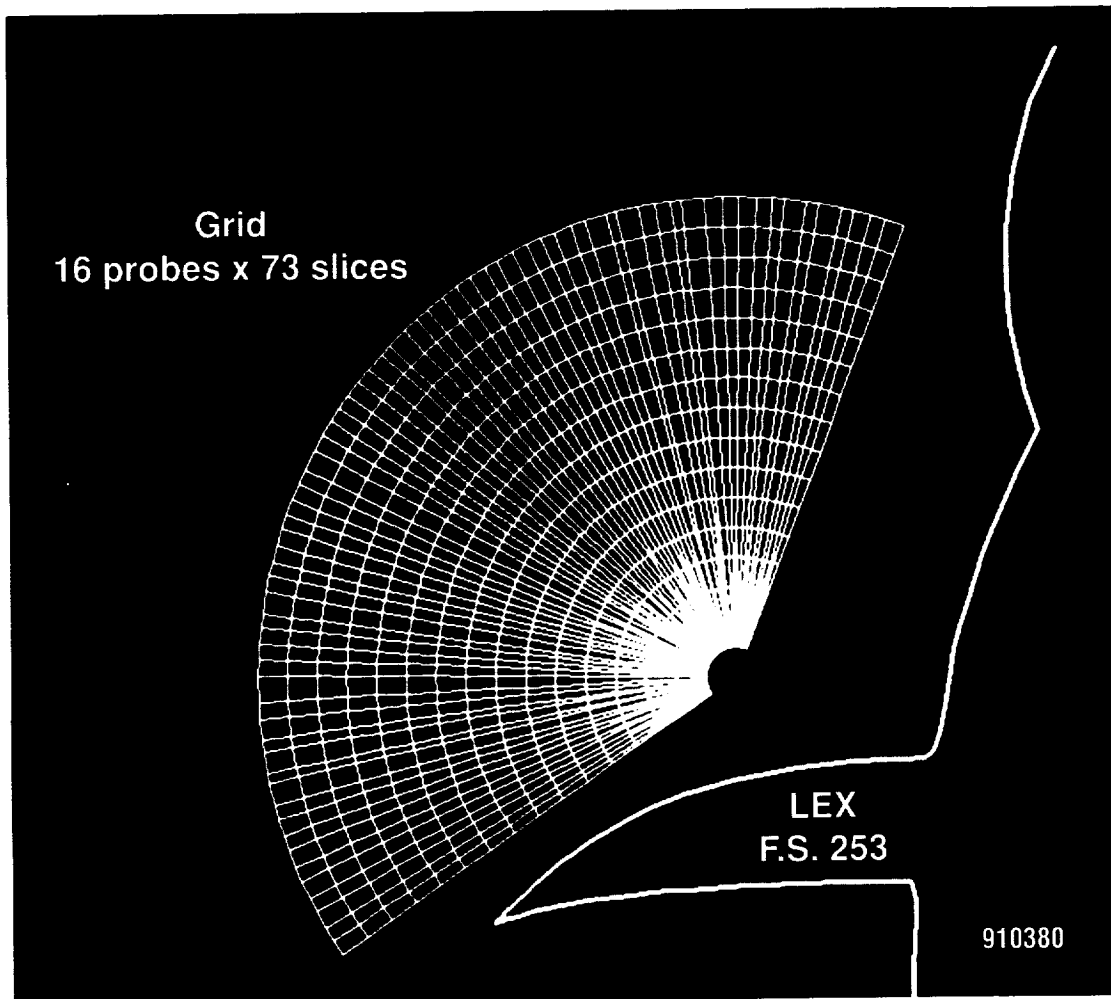
Figure 5. Grid of measured data points.
