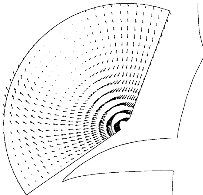
(j) Crossflow velocity vectors, \alpha \approx 48^\circ .
