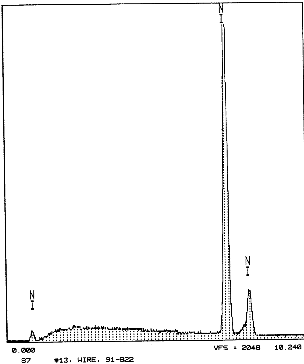
Figure 103. EDAX spectrum of a wire from sample A-14, metallic bits.
