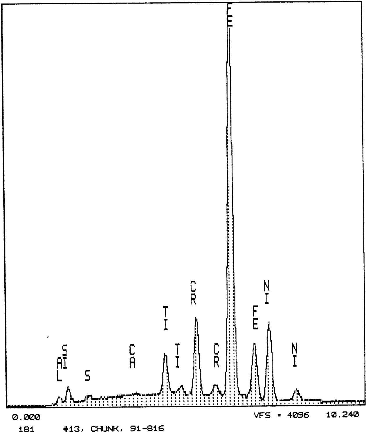
Figure 97. EDAX spectrum of a chunk from sample A-14, metallic bits.
