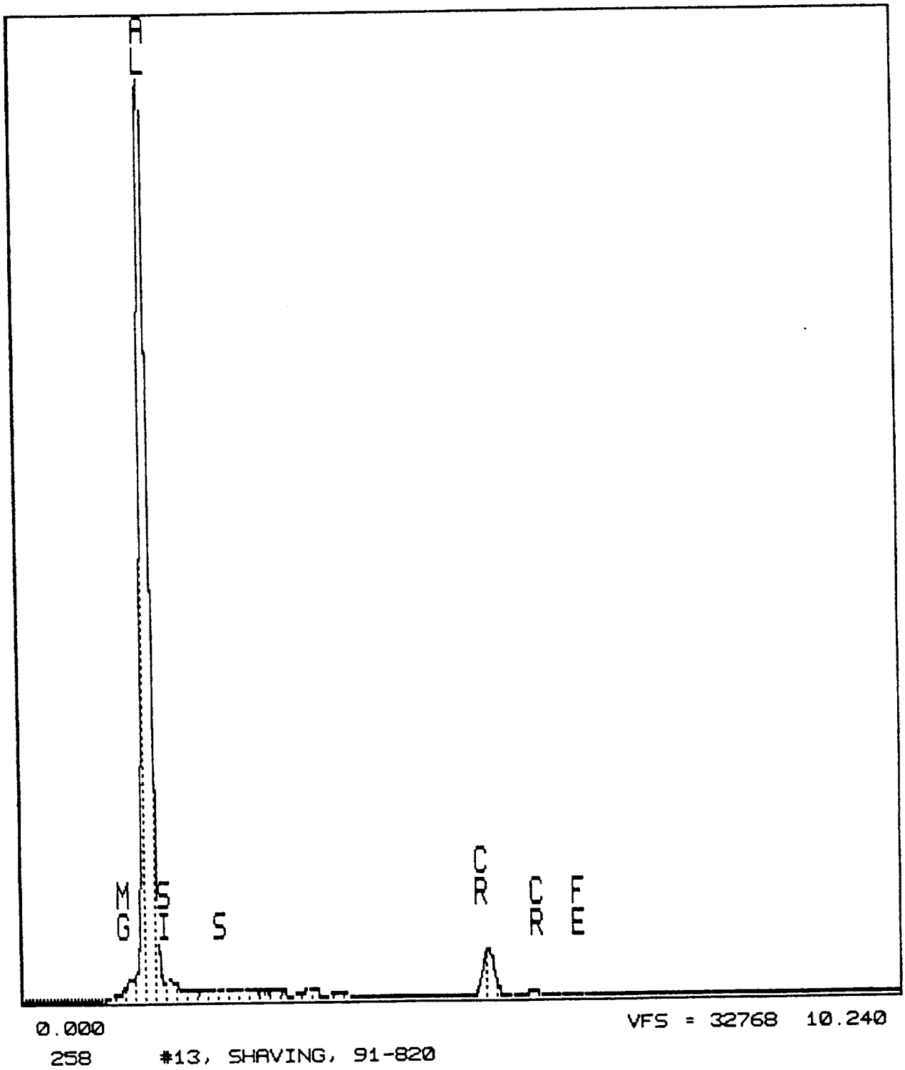
Figure 101. EDAX spectrum of a shaving from sample A-14, metallic bits.
