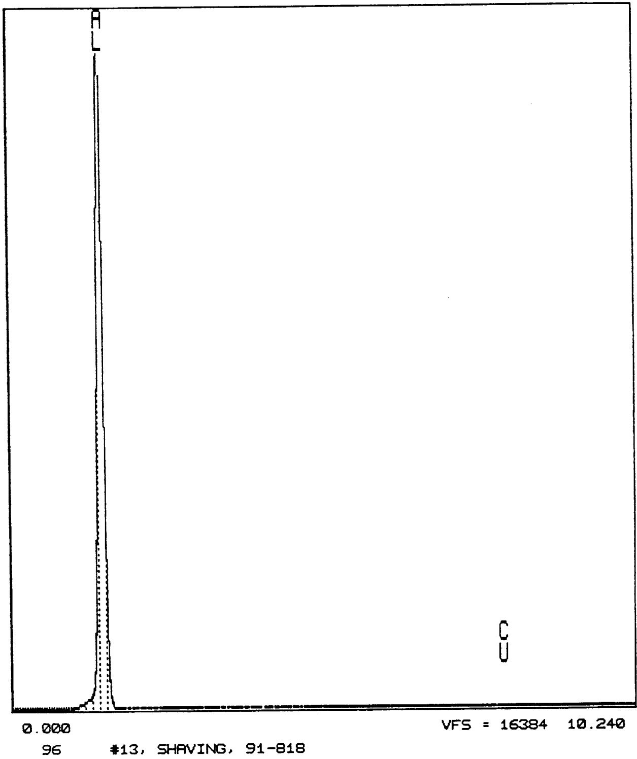
Figure 99. EDAX spectrum of a shaving from sample A-14, metallic bits.
