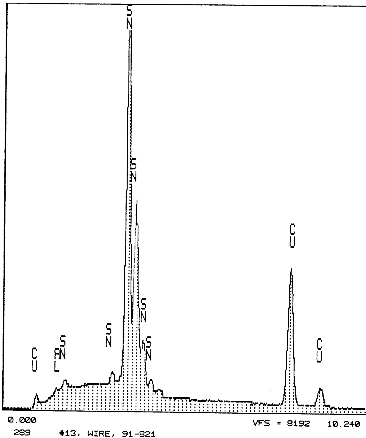
Figure 102. EDAX spectrum of a wire from sample A-14, metallic bits.
