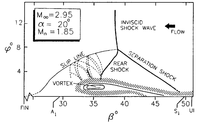
Fig. 2 - Map of Conical Flowfield Structure (Ref. 10).
