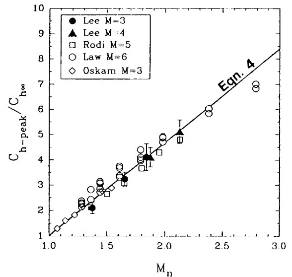
Fig. 16 - New Peak Heating Correlation.
