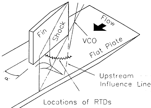
Fig. 1 - Sketch of Test Geometry.
