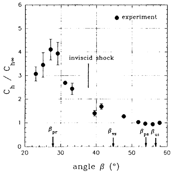
Fig. 13 - C_h/C_{h\infty} vs. \beta for Mach 3, \alpha = 20^\circ .
