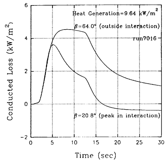
Fig. 9 - Comparison of Conduction Loss Calculation (Mach 4, \alpha = 16^\circ ).
