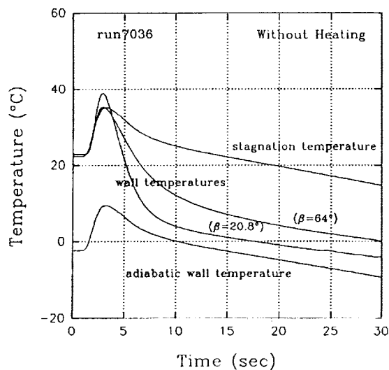
Fig. 7 - Temperature Variations Without Heating (Mach 4, \alpha = 16^\circ ).
