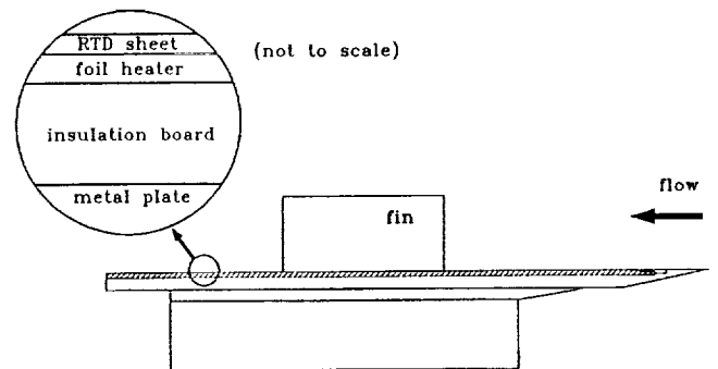
Fig. 3 - Sketch of Multilayer Construction of Flat Plate.
