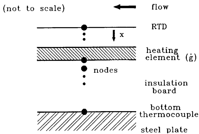
Fig. 6 - Diagram for Computation of Conduction Loss.
