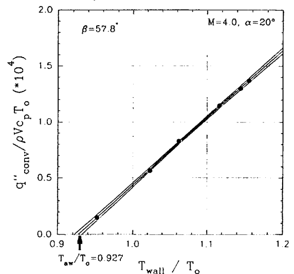
Fig. 10 - Example Determination of Adiabatic Wall Temp.
