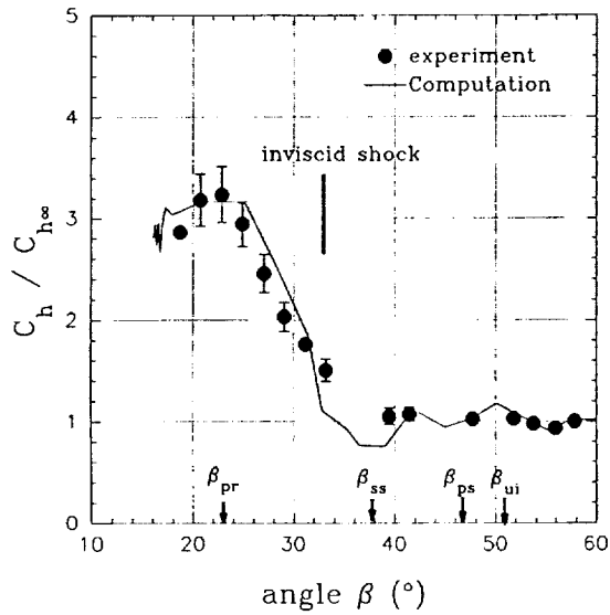
Fig. 12 - C_h/C_{h\infty} vs. \beta for Mach 3, \alpha = 16^\circ .
