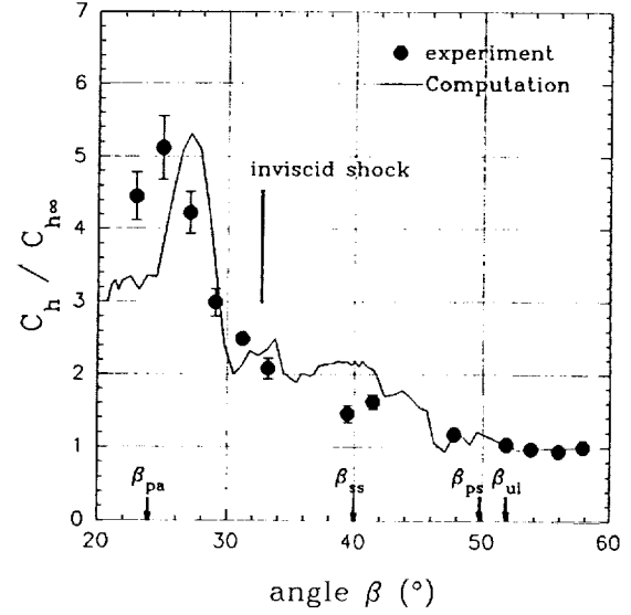
Fig. 15 - C_h/C_{h\infty} vs. \beta for Mach 4, \alpha = 20^\circ .
