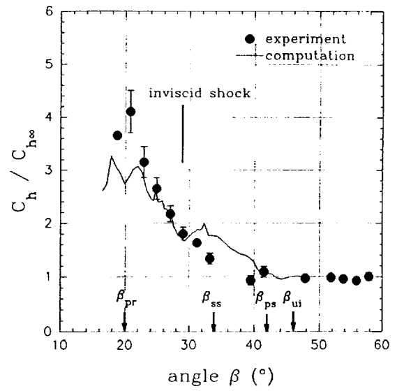
Fig. 14 - C_h/C_{h\infty} vs. \beta for Mach 4, \alpha = 16^\circ .
