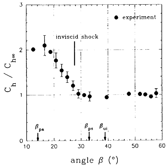
Fig. 11 - C_h/C_{h\infty} vs. \beta for Mach 3, \alpha = 10^\circ .
