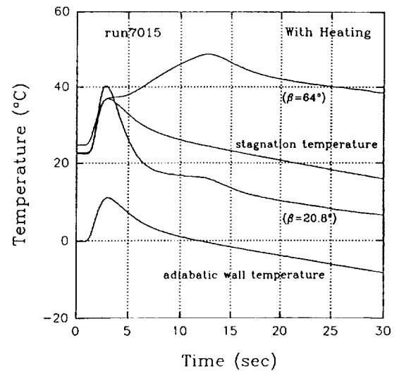
Fig. 8 - Temperature Variations With Heating (Mach 4, \alpha = 16^\circ ).
