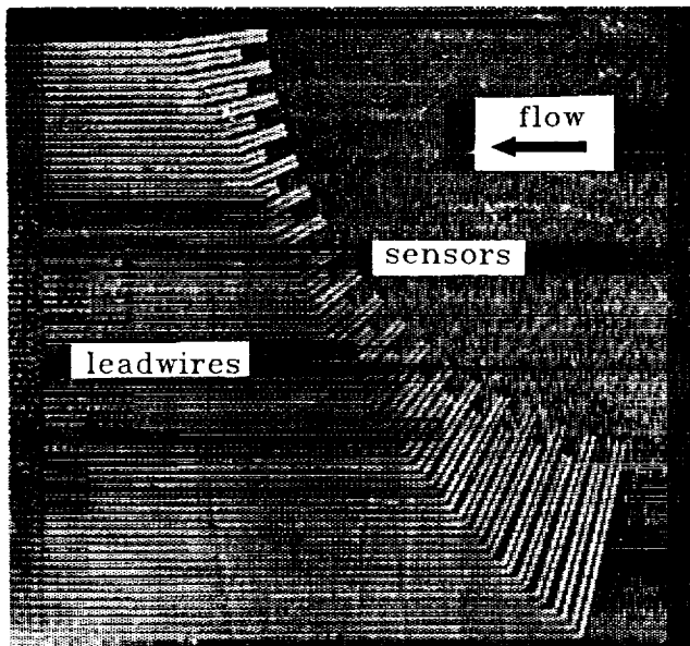
Fig. 5 - Image of 37 RTD Sensors Installed on Plate.
