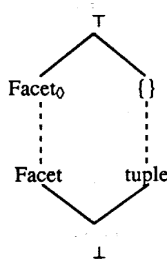
Figure 1. The reuse type lattice
