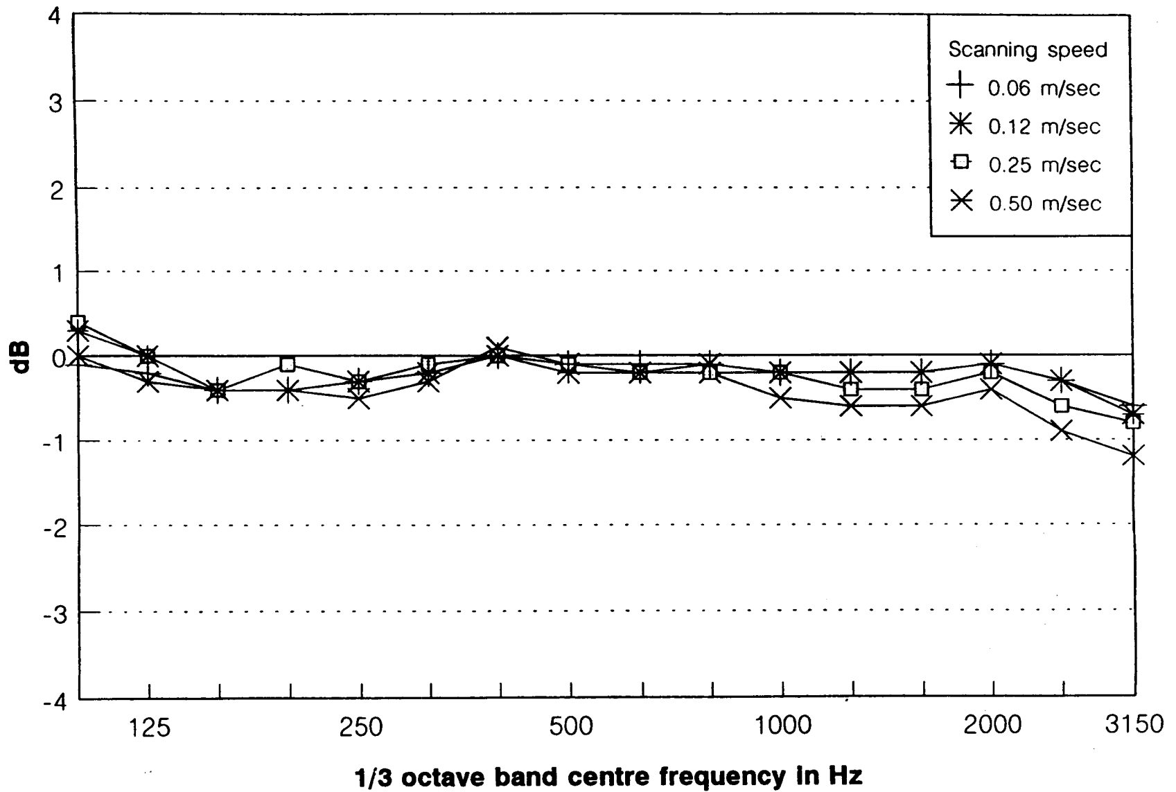
DIFFERENCE IN SOUND POWER LEVELS between manual scanning and discrete-points methods measurement surface: 0.5 m
