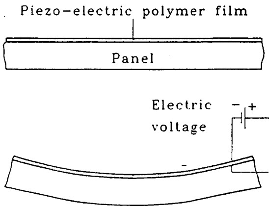
Figure 22: Principle of piezo-electric polymer film attached to a panel
