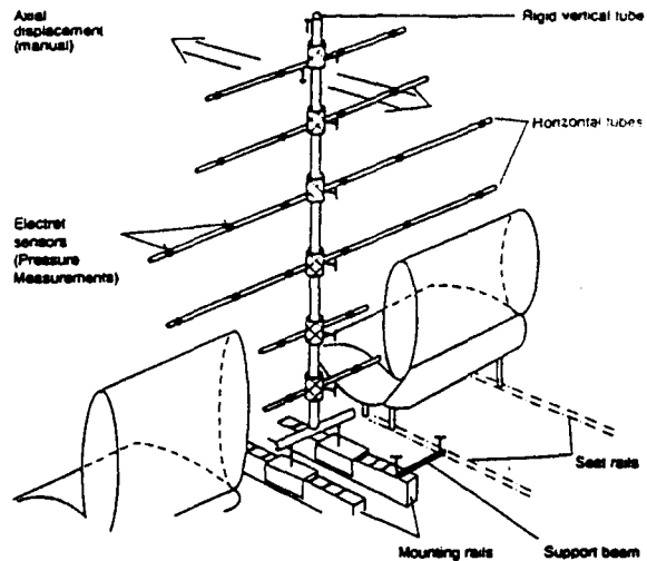
Figure 2: Microphone antenna for in-flight interior noise surveys
