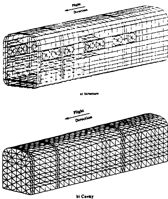
Figure 12: Dornier 228 fuselage and cavity finite element idealization
