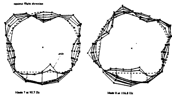
Figure 8: Selected eigenmodes of the ATC
