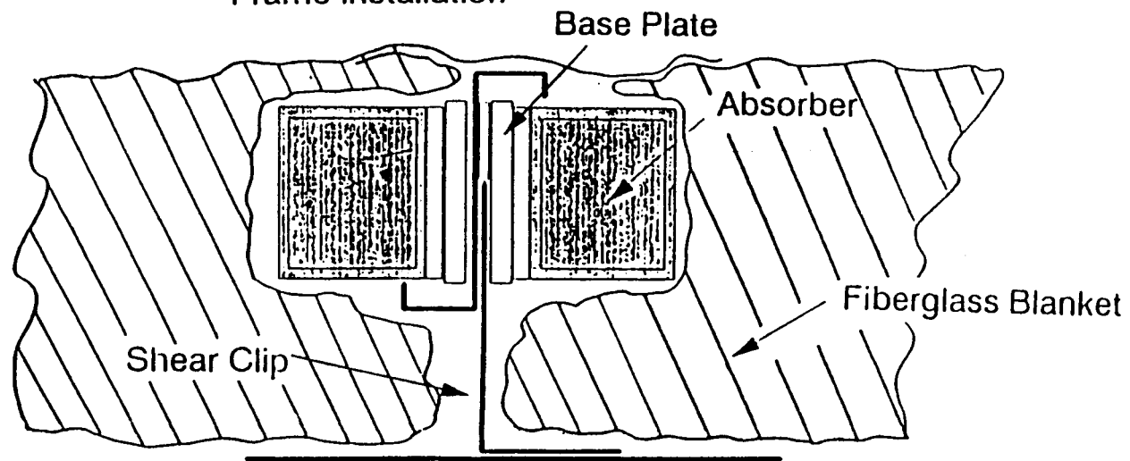
Frame Installation
