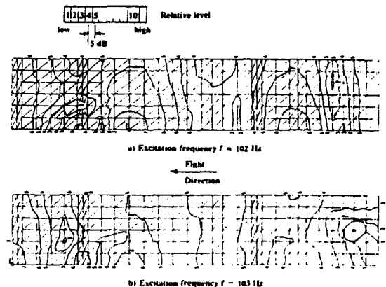
Figure 18: Calculated noise distribution in the plane of the passenger heads of Dornier 228
