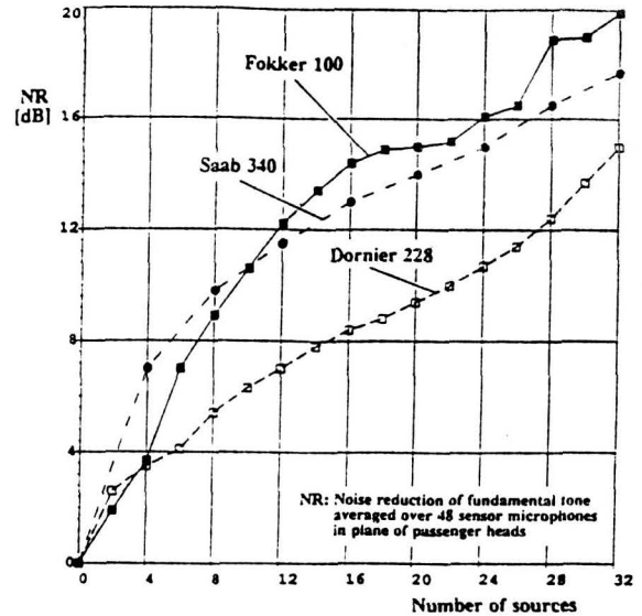
Figure 9: Determined noise reduction (NR) for active noise control based on actuator ground testing
