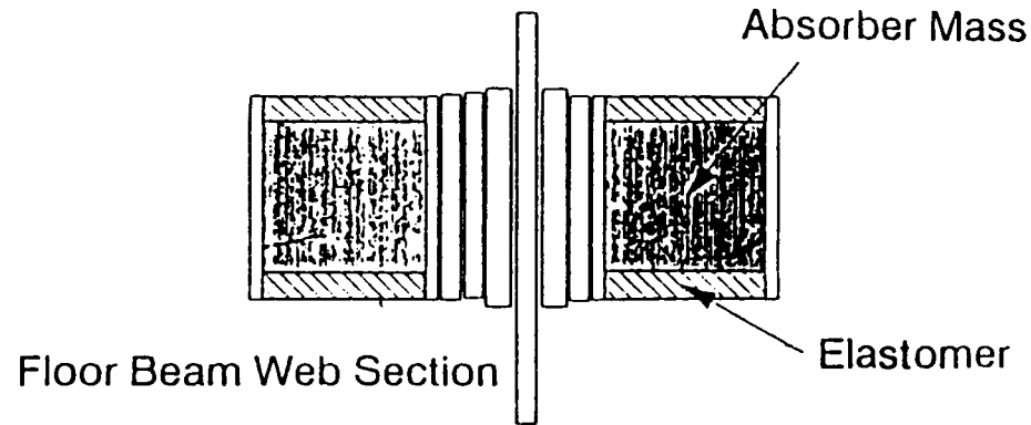
Floor Beam Installation
