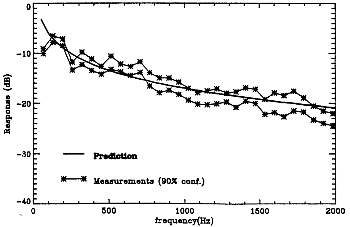
Plate 1 Base 4mm (Vout/Vin) 16 May 1991 - A.S.A.N.C.A. Box
