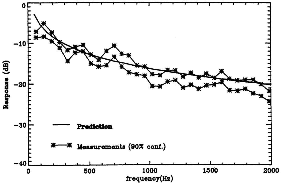
Plate 2 Roof 4mm (Vout/Vin) 16 May 1991 - A.S.A.N.C.A. Box
