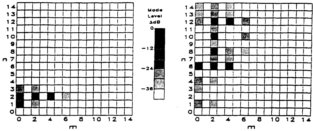
(b) Two piezo actuators, \Delta\theta_2 = 5^\circ
