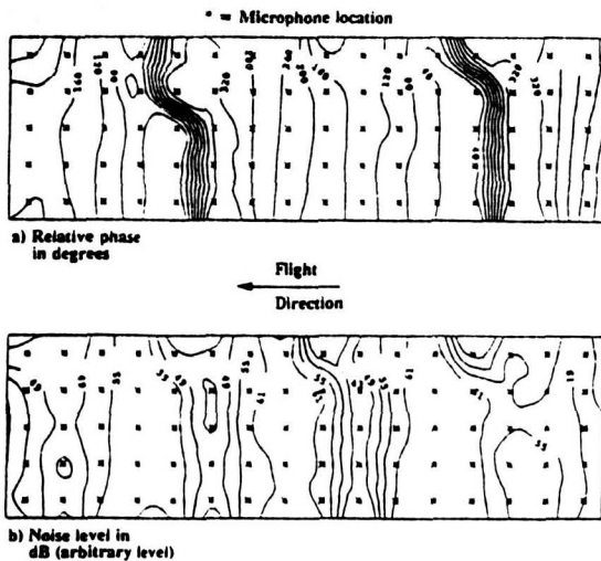
Figure 7: Measured secondary noise field of a speaker at the rear cabin wall of the Dornier 228
