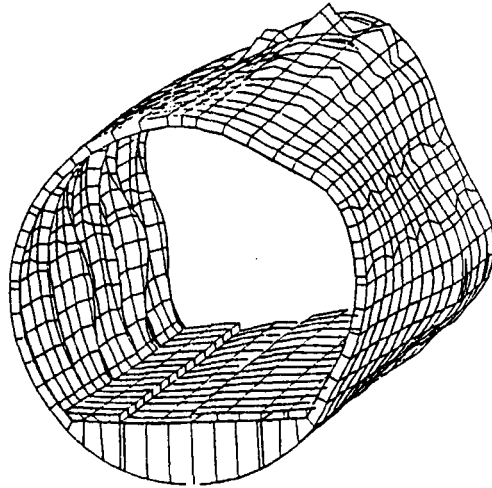
Figure 15: Structural part of coupled Mode 17 of Saab 340 ( f = 85.5 Hz)
