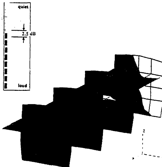
Figure 3: Noise distribution measured in Dornier 228 (1xBPF)
