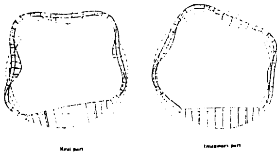
Figure 21: Calculated structural part of coupled response of Saab 340 for 1xBPF due to right propeller
