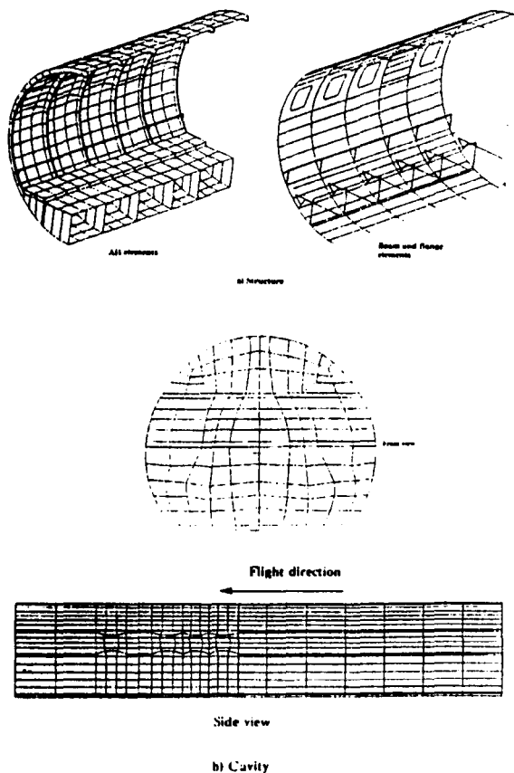
Figure 13: Saab 340 fuselage and cavity finite element idealization
