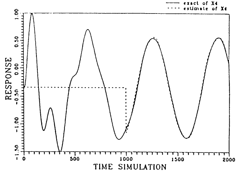
Dynamic Simulation Comparison of Exact and Estimate for X4 (Neural Observer turned on at instant k=1000)
