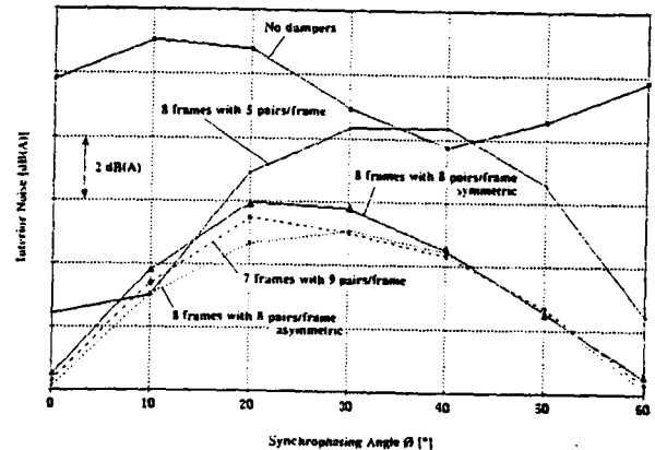
Figure 14: Total averaged interior noise levels for simulated propeller noise (1050 RPM)
