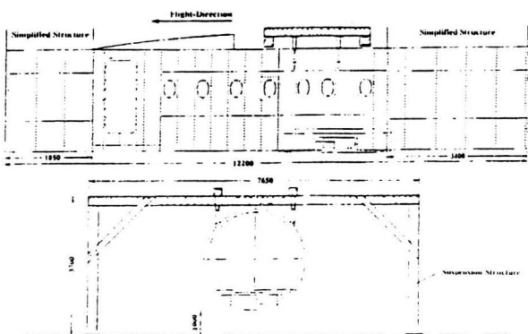
Figure 2: Structure and suspension of the ATC
