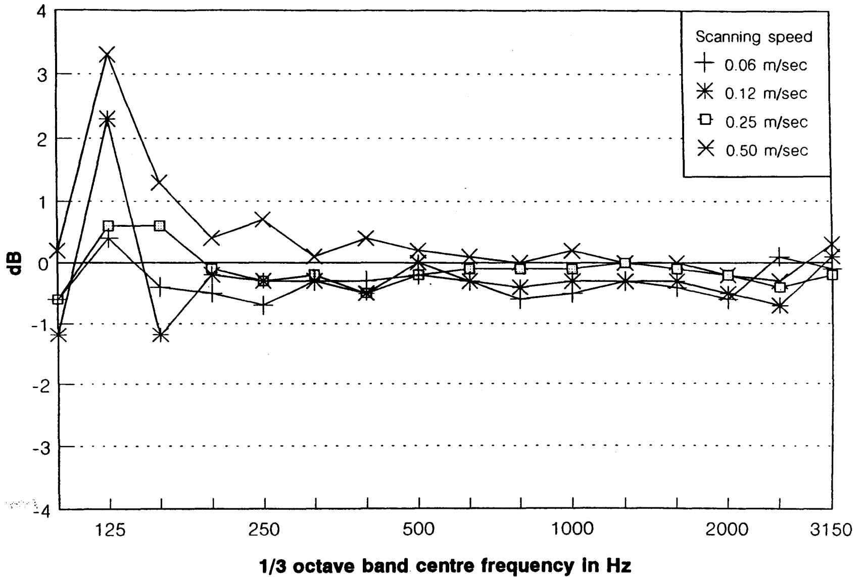
DIFFERENCE IN SOUND POWER LEVELS between mechanical scanning & discrete-points methods measurement surface: 0.25 m
