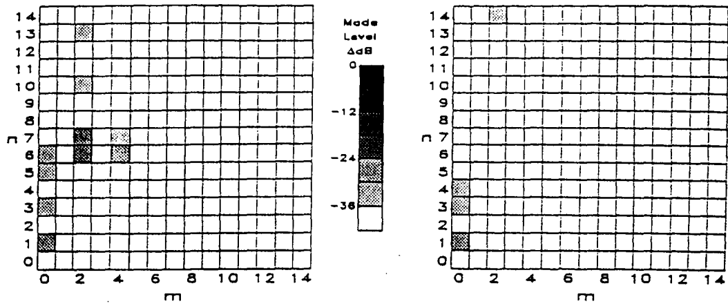
(a) Single piezoactuator, \Delta\theta_2=90^\circ
