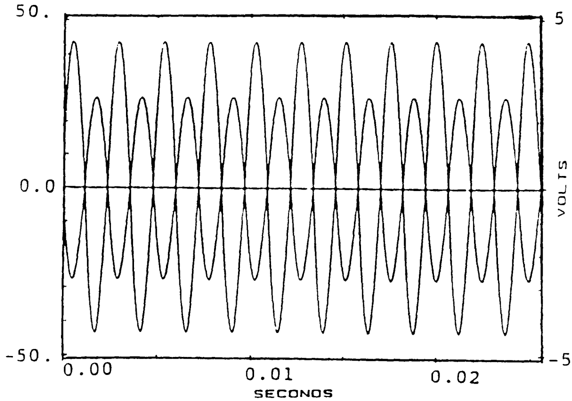
RECORDED INPUT AND OUTPUT SIGNALS AT 410 HZ FROM ACTUATOR 1 AND SENSOR 5
