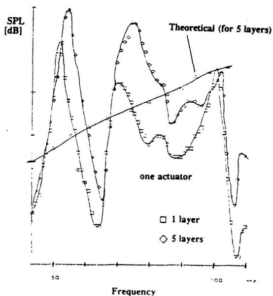
Figure 25: Radiated noise levels of the first trim panel integrated PVDF actuator design
