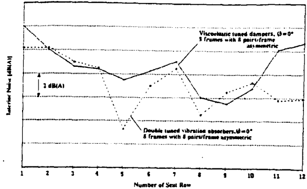
Figure 17: Interior noise distributions averaged at the passenger ear positions for simulated propeller noise (1050 RPM)
