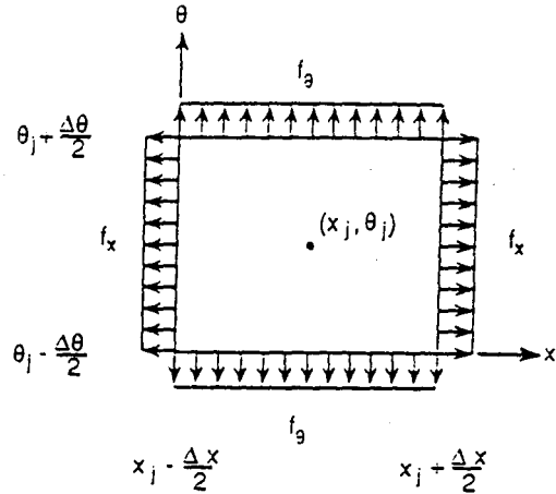
Figure 2. Piezo actuator force model
