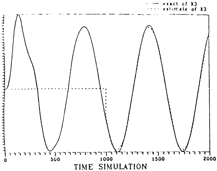
Dynamic Simulation Comparison of Exact and Estimate for X3 (Neural Observer turned on at instant k=1000)
