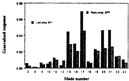
Generalised response at BPF, comparison between left and right propeller contributions.
