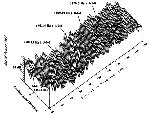
Figure 17: Predicted frequency dependent average noise levels inside Dornier 228 versus fuselage axial direction
