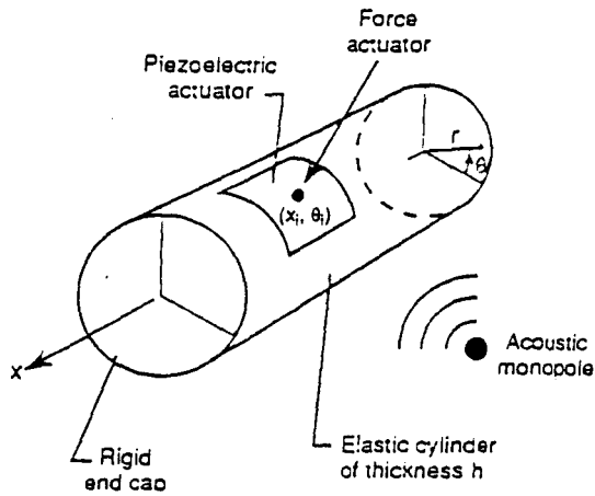
Figure 1. Schematic of fuselage model
