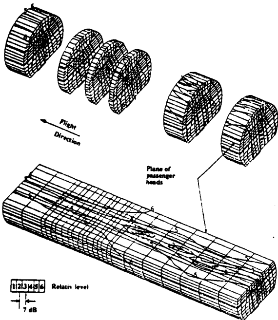
Figure 20: Predicted acoustic part of coupled response of Saab 340 for 1xBPF due to right propeller
