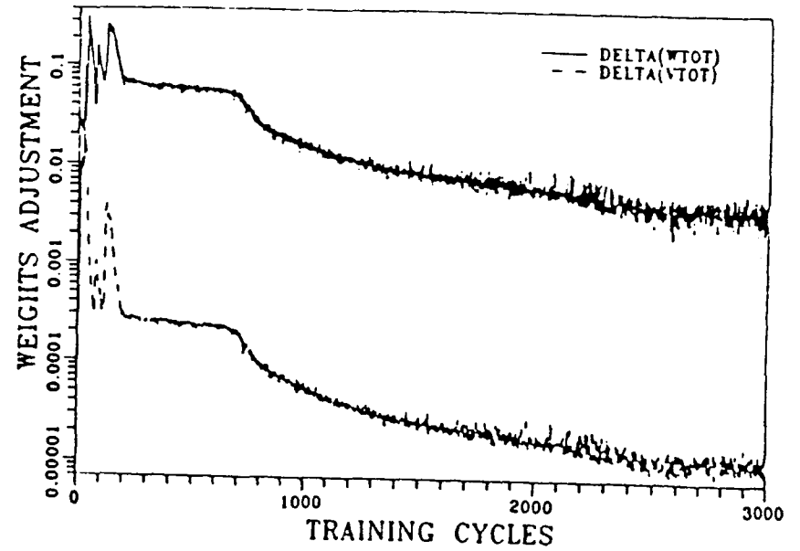
Weights Adjustment vs. Training Cycles
