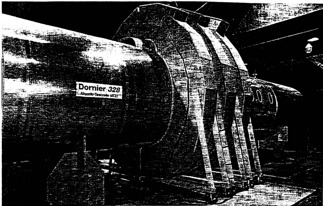
Figure 1: The Dornier 328 Acoustic Test Cell (ATC)
