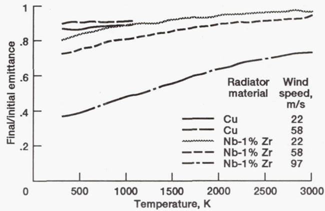
Figure 5.—Degradation of initially clear radiator samples subjected to dust laden wind.
