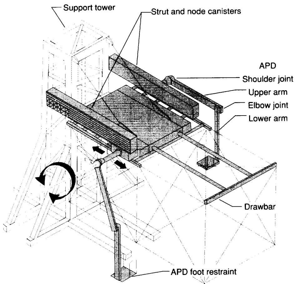
(b) Mock-up.
