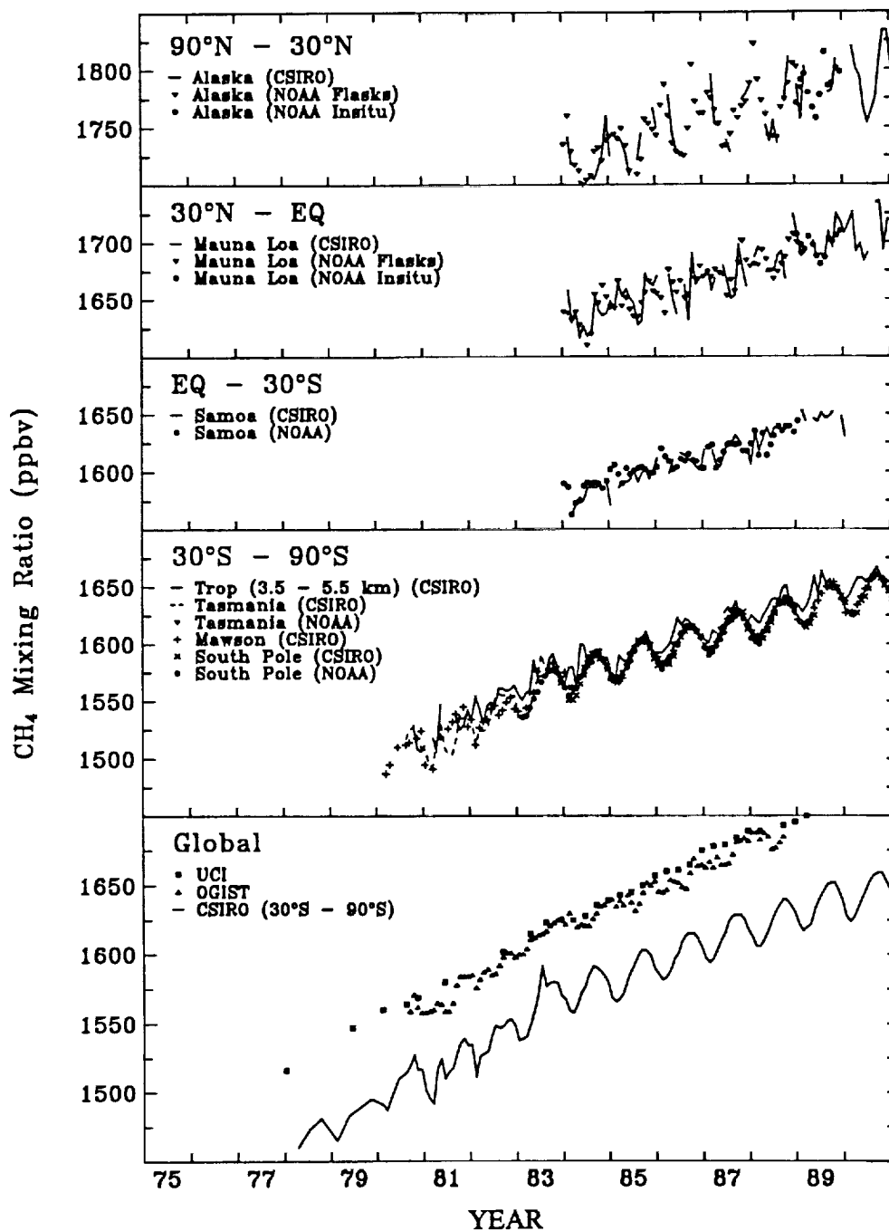
Figure 1-8 Methane observations (ppbv) in the four semihemispheres (NOAA: Steele et al. , 1987; Lang et al. , 1990a, b. CSIRO: Fraser et al. , 1986a, 1990; Fraser, 1991. OGIST: Khalil and Rasmussen, 1990a. UCI: Blake and Rowland, 1988; Rowland, 1990; Blake and Rowland 1991). The CSIRO (30°S-90°S) data are averages of Cape Grim (41°S) and Mawson (67°S) data. Some of the data are unpublished and are subject to revision. Data should not be used for further analysis without consulting the principal investigators: CSIRO, P. Fraser; UCI, D. Blake.
