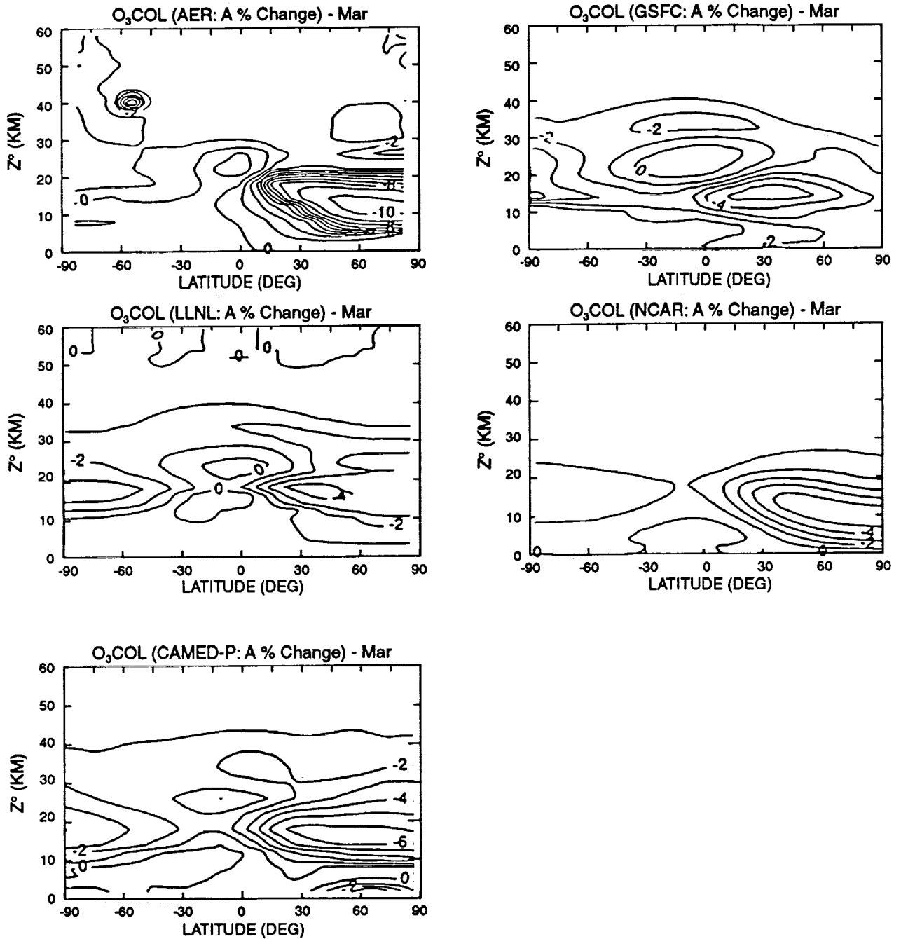
Figure 9-4 Calculated percent changes in the local concentration of O 3 as functions of latitude and height for a fleet of Mach 2.4 supersonic aircraft with EI(NO x ) = 15. The annual fuel use is 70 × 10 9 kg/year. The latitudinal distribution of fuel use is given in Figure 9-1. The percent change is calculated relative to a 2015 atmosphere with a subsonic fleet. The contour interval is one percent.
