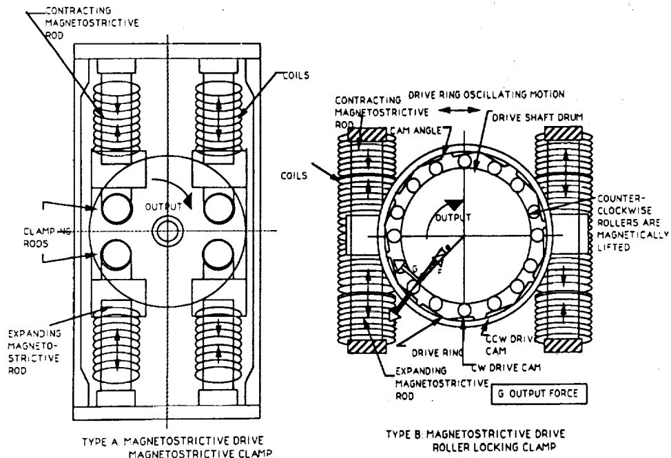
FIG. 3 MAGNETOSTRICTIVE DIRECT DRIVE MOTOR COMPETING DESIGN CONCEPTS
