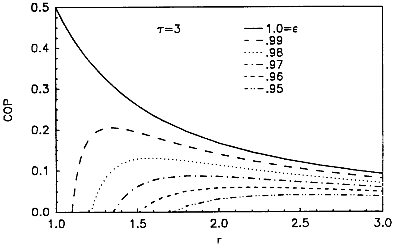
Figure 2.2.1-5 Coefficient of Performance of an Orifice Pulse Tube as a Function of Expansion Ratio at \tau=3 .
