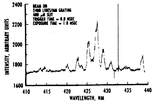
Fig. 13. Spectrometer/array detector spectrum for Run 8010.
