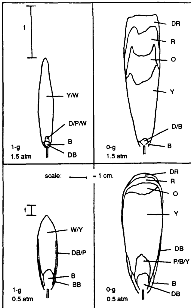
Fig. 6. Effects of pressure on normal-gravity and microgravity flames of propane burning in quiescent air (21% oxygen in nitrogen). For details, see Fig. 4. From Babadori et al. (1990b).
