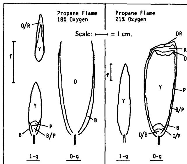
Fig. 5. Effects of oxygen concentration on normal-gravity and microgravity flames of propane at 1 atm; nozzle radius = 0.074 cm and fuel-flow rate = 0.96 cc/sec. The various colors indicated in the diagram are as follows: B (blue), D (dark), DR (dull red), O (orange), P (pink), R (red), W (white), and Y (yellow). The bars show the range of normal-gravity flame flicker ( f ). From Babadori and Stocker (1989).
