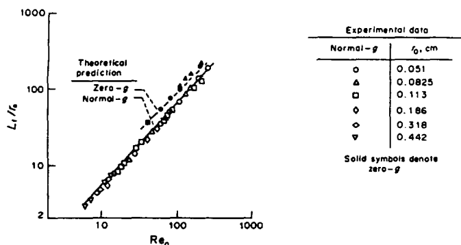
Fig. 8. Comparisons between the theoretical predictions (Edelman et al., 1973) and experimental results (Cochran and Masicca, 1970; Cochran, 1972) for nondimensional flame height (height/nozzle radius) vs. jet Reynolds number (jet velocity \times nozzle radius/fuel kinematic viscosity); methane-air flames at 1.0 atm. From Edelman et al. (1973).
