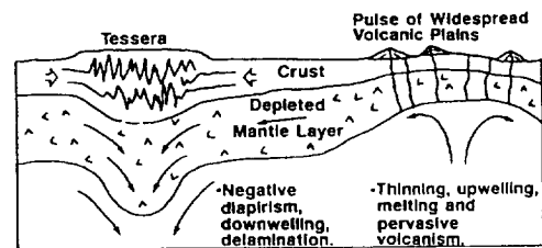
Fig. 2. Instabilities that develop in a depleted layer.
