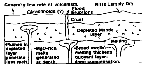
Fig. 1. Stationary thick depleted mantle layer.
