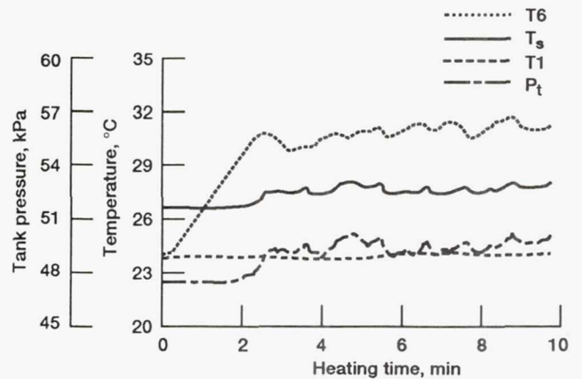
Figure 6.—Heater and liquid temperatures and tank pressure as functions of time: Run no. 19.
