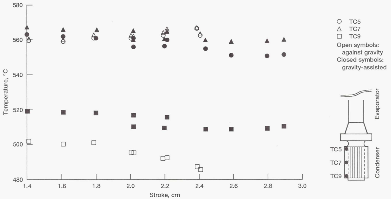
Figure 16.—Condenser temperature profiles for an HP-1000 heat pipe operating against gravity and in gravity-assisted mode.
