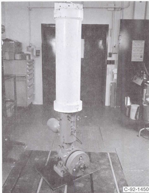
Figure 13.—Philips/STM regenerator test rig.
