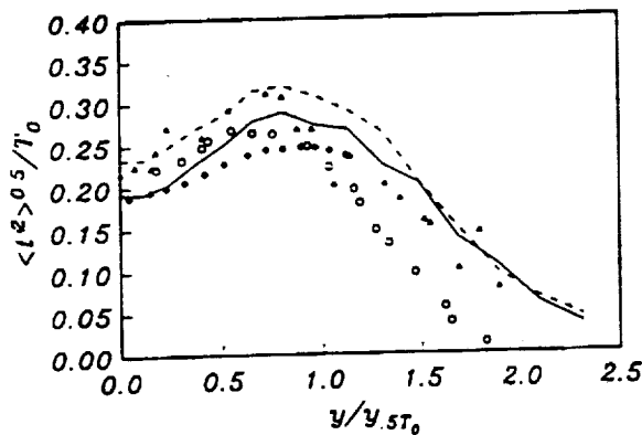
Figure 6. RMS of temperature variance in heated plane jet. — continuous mixing model, - - - modified Curl model, \Delta Antonia et al. (1983), \circ Bashir and Uberoi (1975), \Delta Uberoi and Singh (1975).
