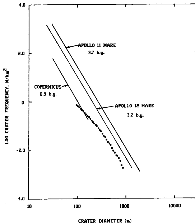
Fig. 4. Crater-frequency distribution for the mare basalt flows of Mare Smythii (squares), shown in comparison to those of the Apollo 11 and 12 landing sites and the crater Copernicus (from BVSP, 1981). Position of the Smythii curve indicates that these lava flows are significantly younger than those of the Apollo 12 site (the youngest sampled lunar lavas); the age of the Smythii flows is probably about 1 to 2 b.y.
