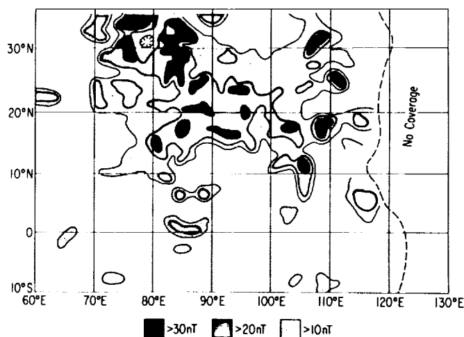
Fig. 5. Amplitude of near-surface magnetic fields in the region of Maria Smythii and Marginis as deduced from the reflection of low-energy electrons (from Hood and Williams, 1988).
