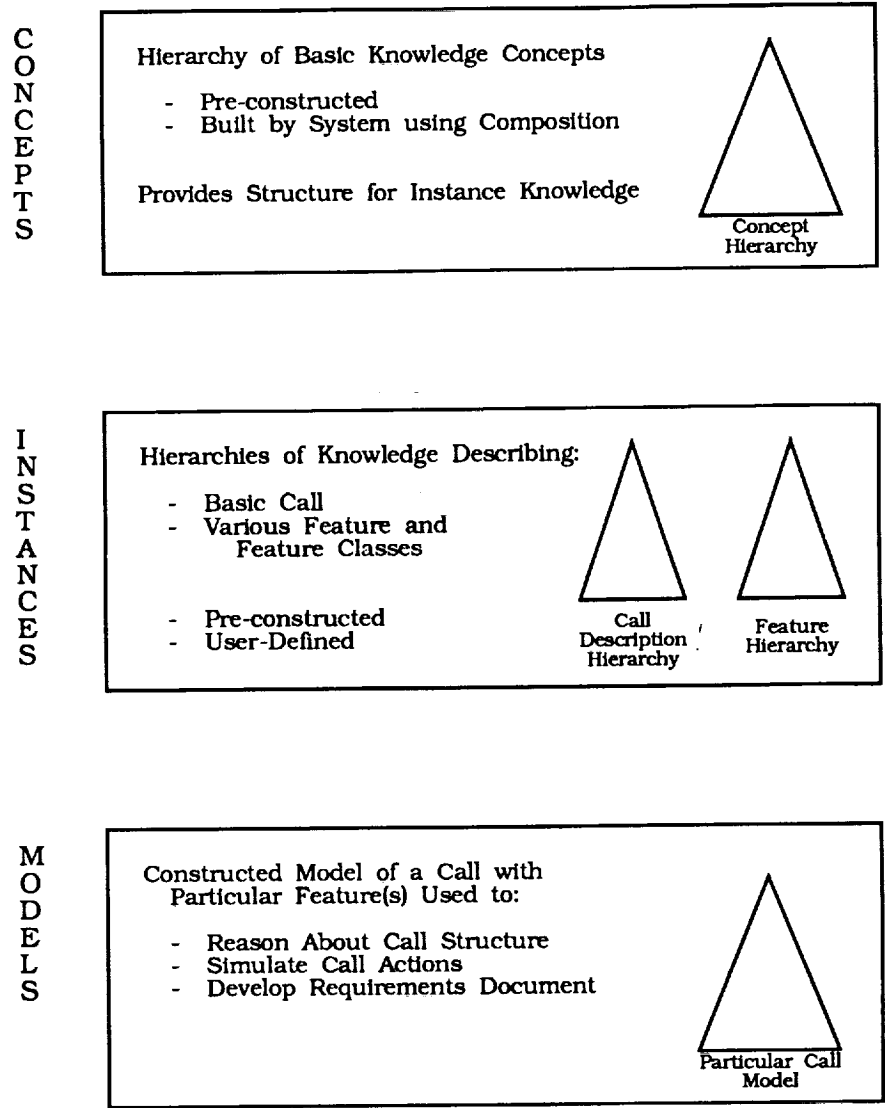
Figure 2. A Conceptual Diagram of the Knowledge Levels within the Call & Feature Knowledge Base
