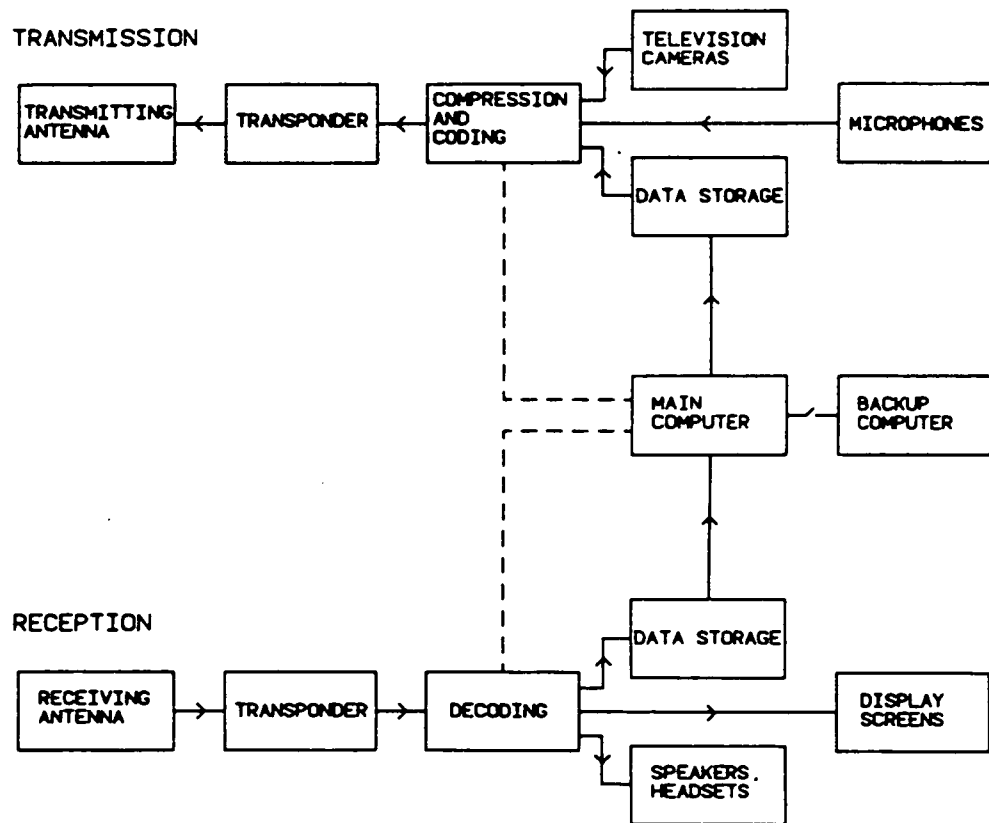
Figure 5-2: Communications System
