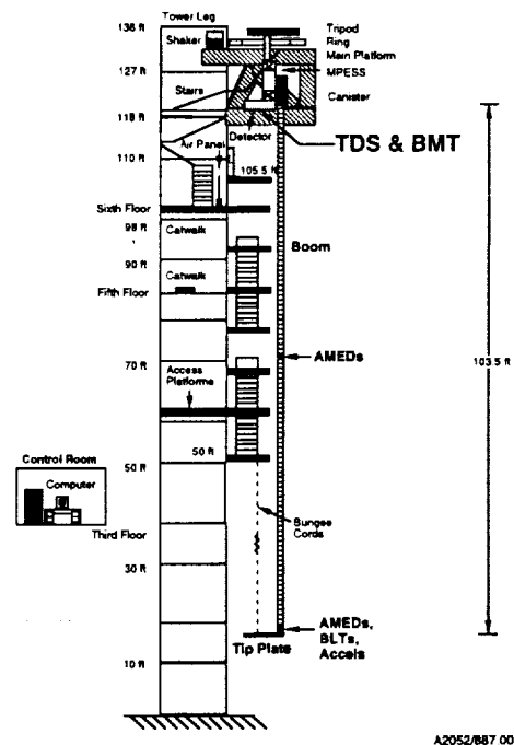
CASES Ground Test Facility (GTF)
