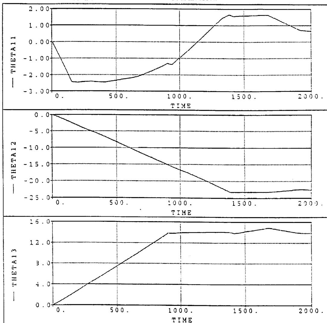
Figure 5-a: Vehicle Attitude w.r.t. LVLH, SSF RCS, SRMS Brakes on at Capture (Scenario 3)
