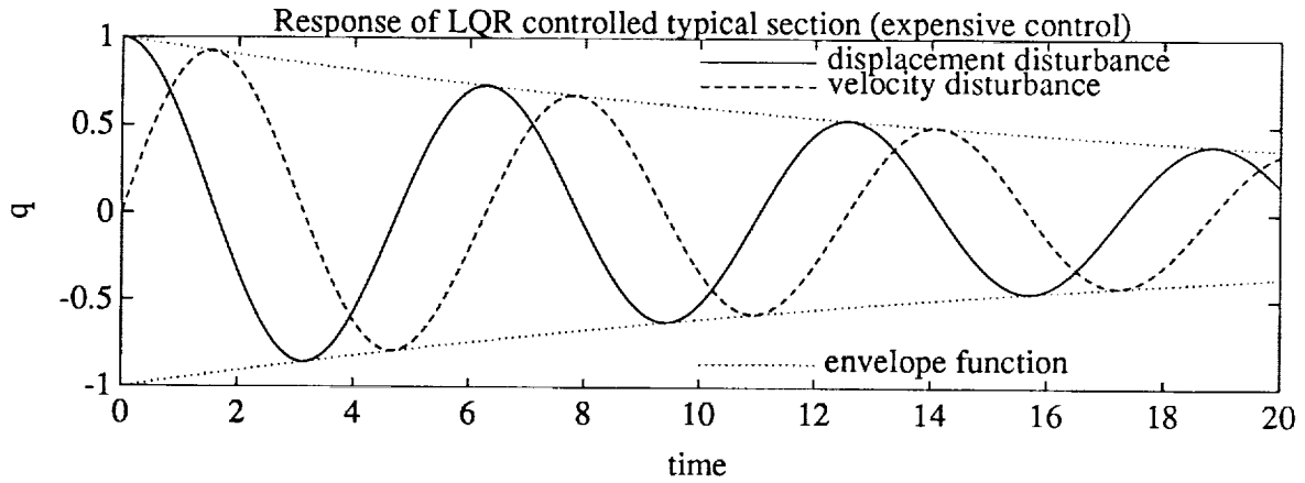
Figure 2: Response of single mass typical section for displacement and velocity disturbances: \omega = 1 , \zeta = 0 , G_d = G_v = 1 , \mathcal{N} = 1 , \rho = 10 .
