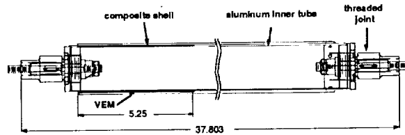
Sketch of V-strut
