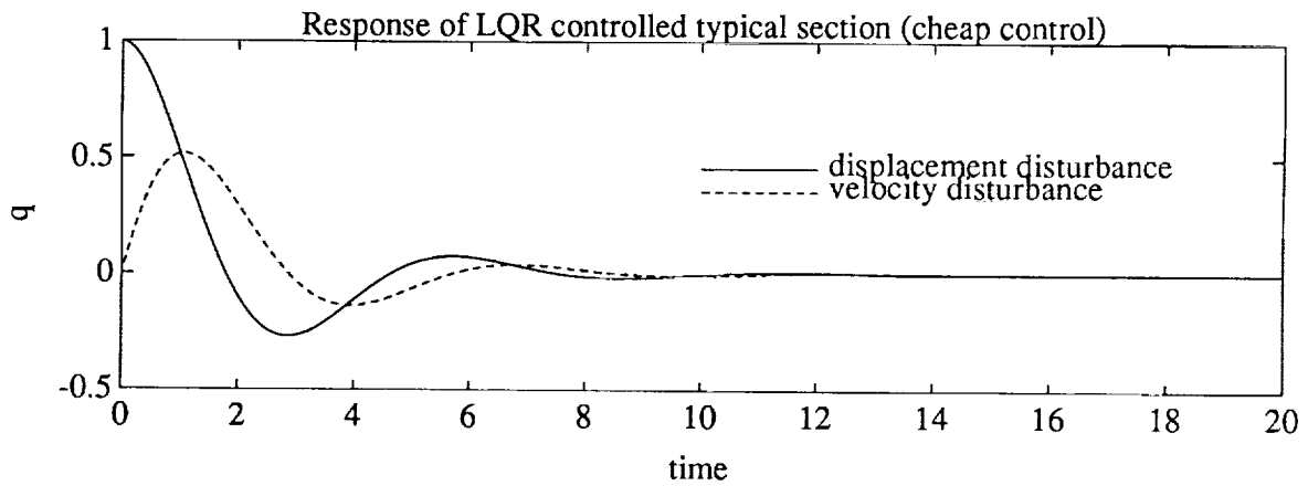
Figure 3: Response of single mass typical section for displacement and velocity disturbances: \omega = 1 , \zeta = 0 , G_d = G_v = 1 , \mathcal{N} = 1 , \rho = 1 .
