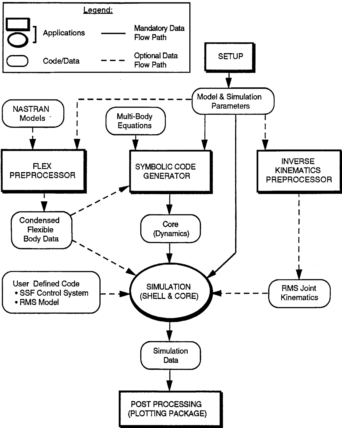
Figure 1: Organization of the SOMBAT Simulation Environment
