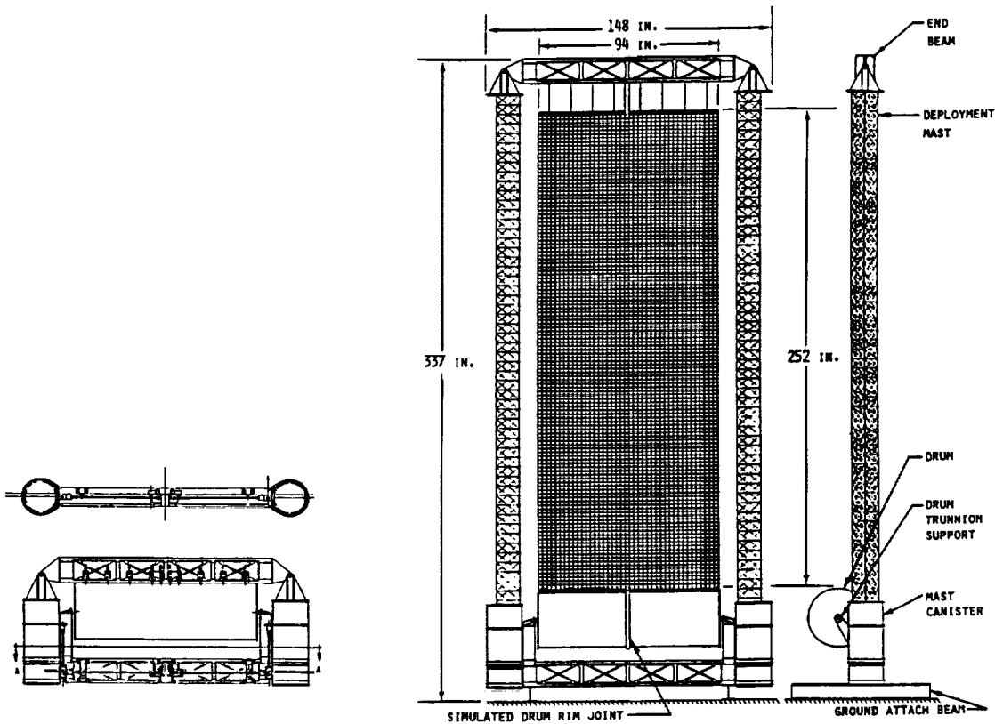
Figure 4. Deployed LADD test article
