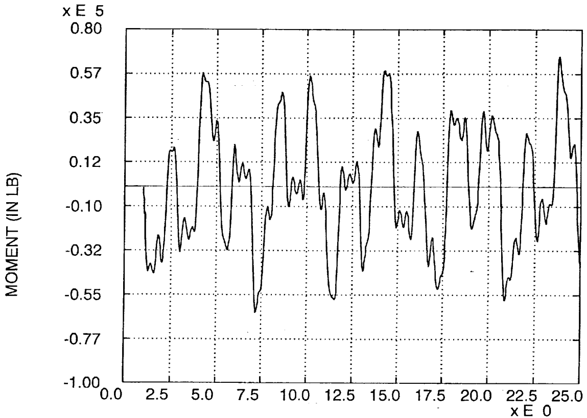
FIGURE 3A. INTERFACE MOMENT W/O CONTROL T(SEC)
