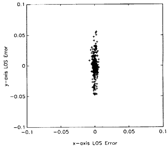
Figure 14: Experimental Closed Loop x-y LOS Error.
