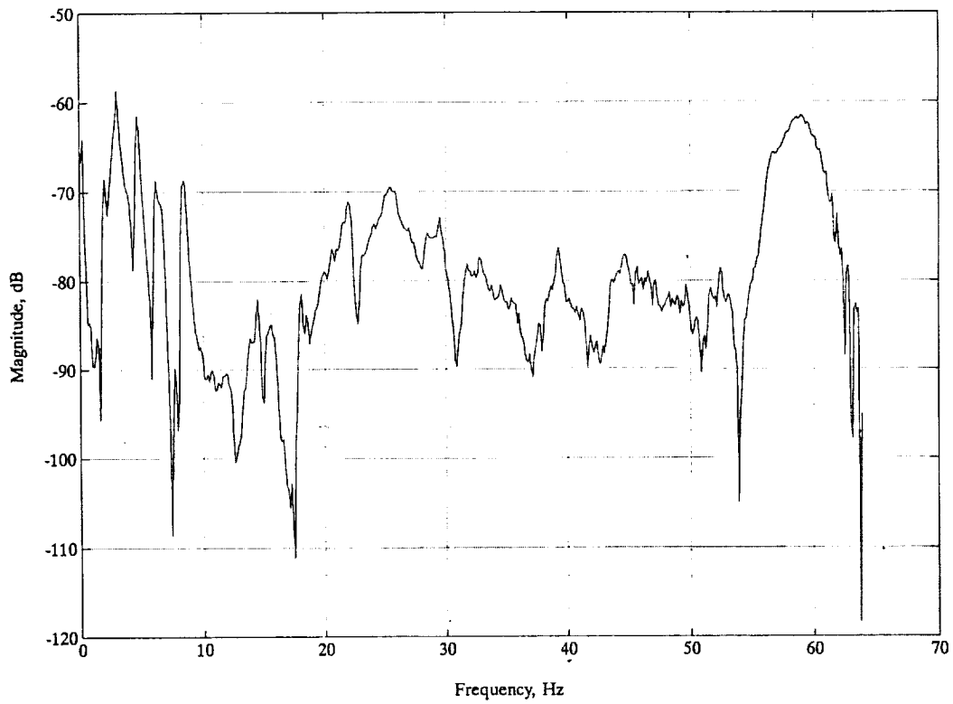
Figure 3. Mid-Boom FRF, (X - Axis)
