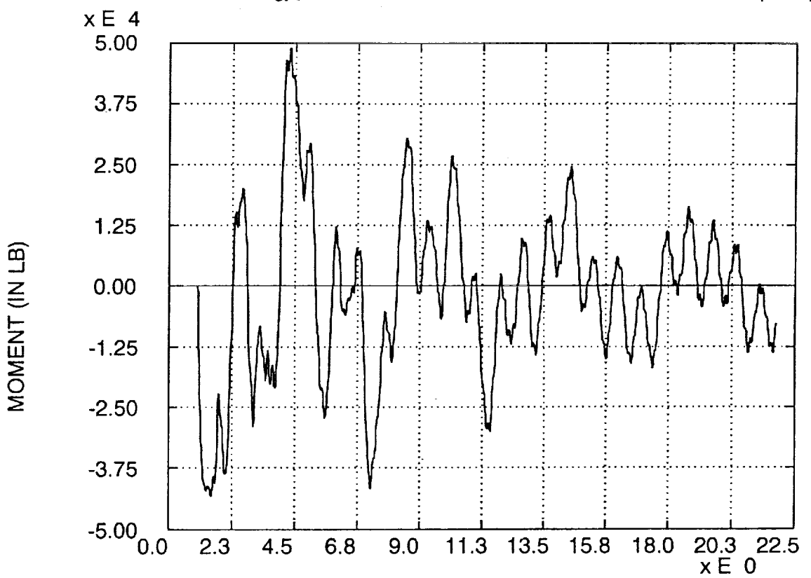
FIGURE 5B. INTERFACE MOMENT-8 MODE INPUT T(SEC)
