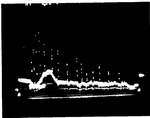
Oscilloscope Picture of BMT X-sensor Showing 15 Targets
