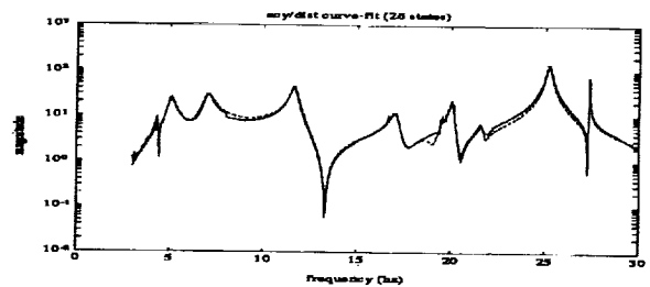
From shaker load cell to \mu g accelerometer at 752Y
