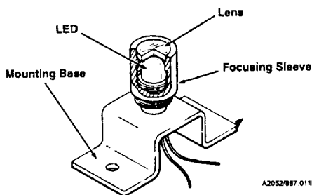
TDS Illuminator/Target
