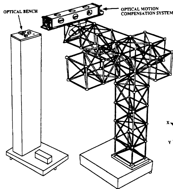
JPL's CSI Phase B Testbed
