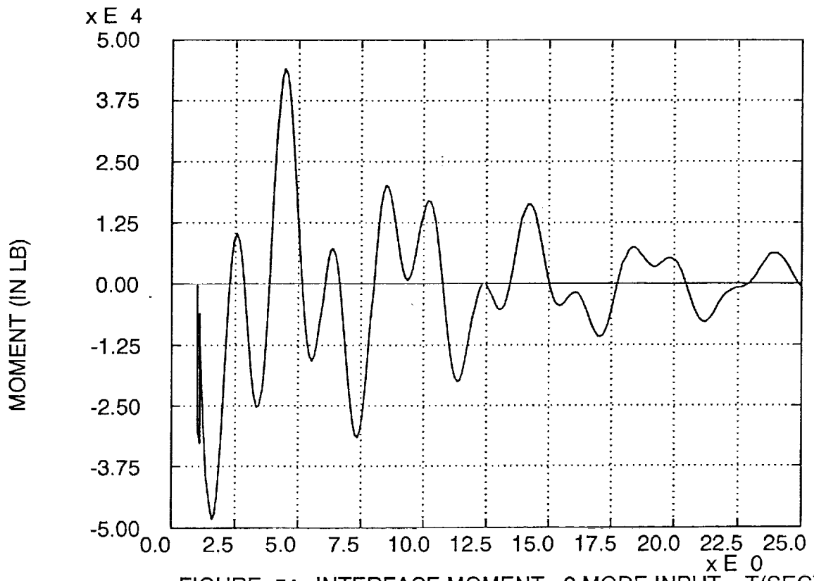
FIGURE 5A. INTERFACE MOMENT - 2 MODE INPUT T(SEC)
