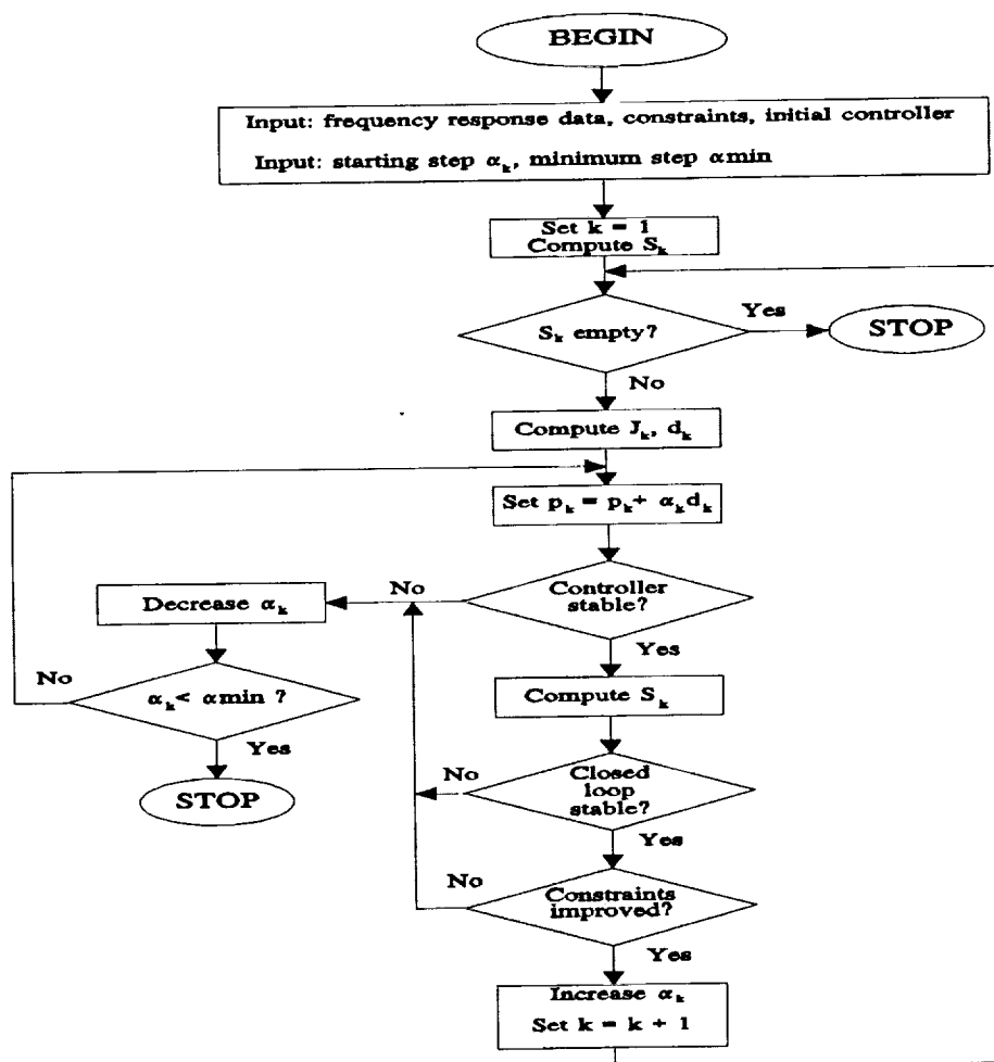
Figure 1: Algorithm Flowchart.
