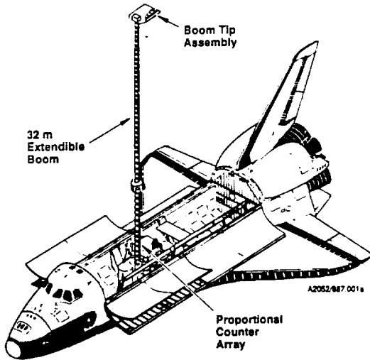
CASES Flight Experiment
