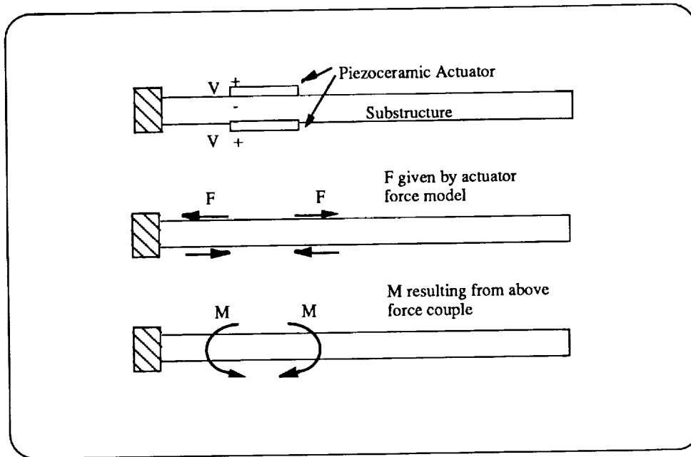
Development of Voltage - Tip Deflection Relationship Figure 2
