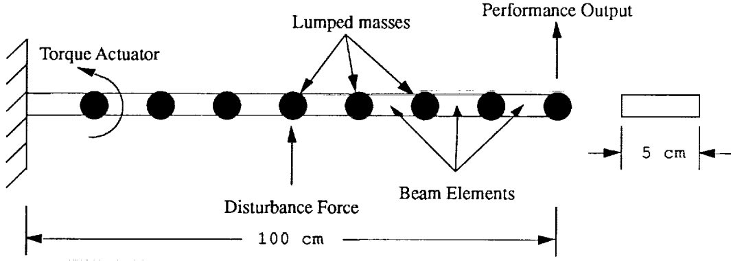
Figure 5: Cantilevered aluminum beam model. E = 73GPa , \rho = 2700kg/m^3
