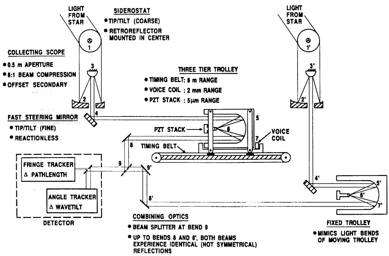
Figure 2. Optical Layout of an Interferometer
