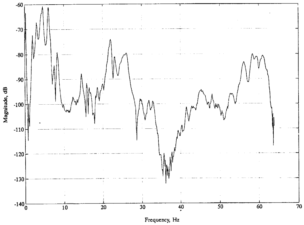
Figure 4. Boom Tip FRF, (X - Axis)
