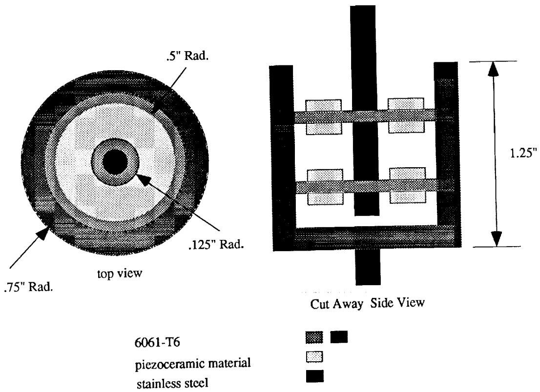
Figure 2. Prototype strut
