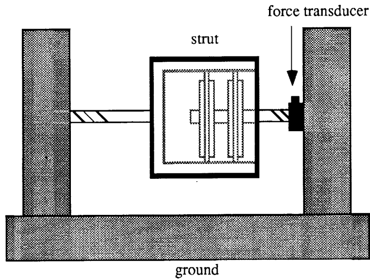
Figure 3. Experimental configuration
