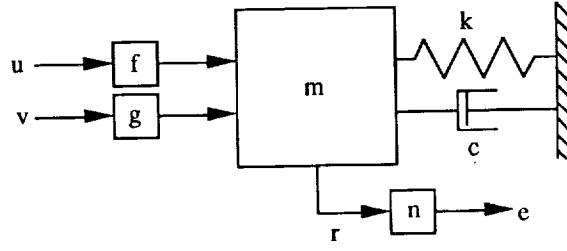
Figure 1: Typical section
