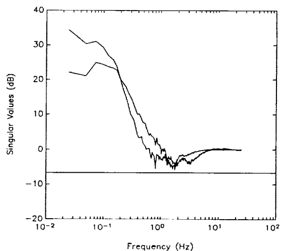
Figure 6: Final Singular Value Frequency Response of (I + GK)_{IMC} .
