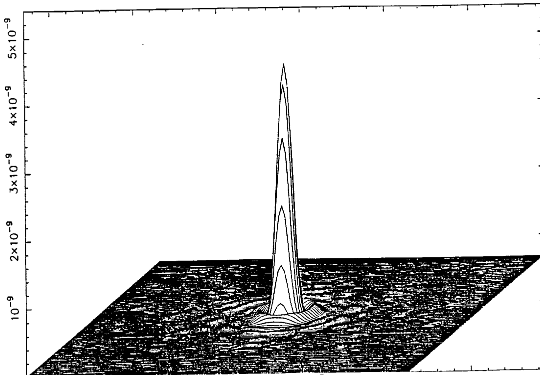
The Unperturbed System Point Spread Function
