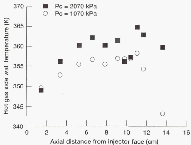
Figure 4.—Comparison of hot-gas side wall temperatures as measured by thermocouples at a depth of 0.076 cm.
