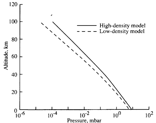
Figure 5. COSPAR vertical pressure profile of Martian atmosphere model.
