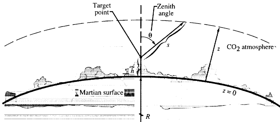
Figure 10. Martian atmosphere geometry and parameters associated with dose calculations at target point.
