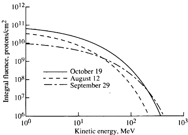
Figure 4. Three large solar flare fluences for 1989 solar proton events; graph based on GOES-7 data.
