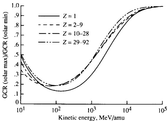
Figure 2. Ratios of galactic cosmic ray differential flux at solar maximum to corresponding flux at solar minimum for selected elemental groups.
