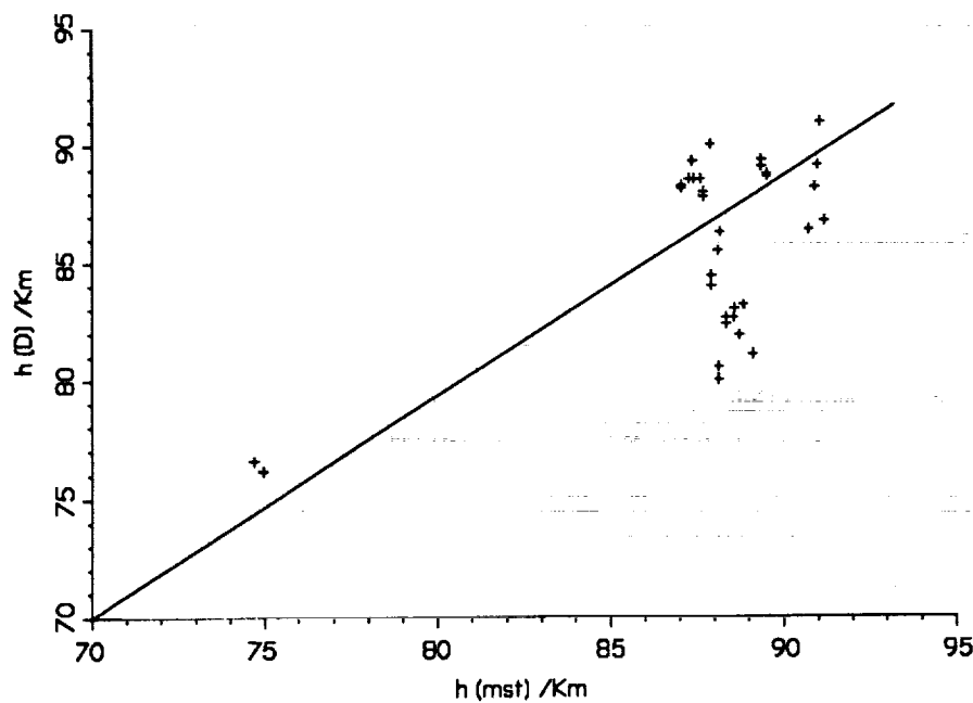
Fig. 1. Diffusion height, h(D) , against true height, h(\text{MST}) for Geminids
