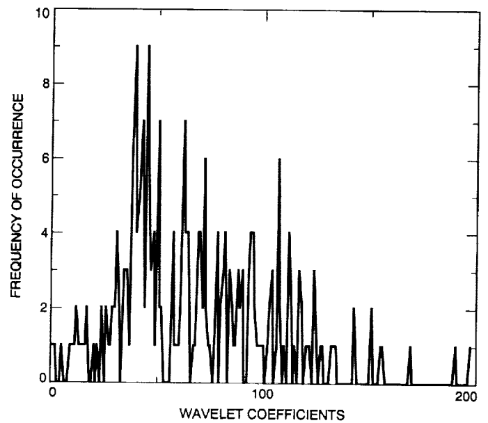
Fig. 4. Level SS-4 wavelet coefficients.
