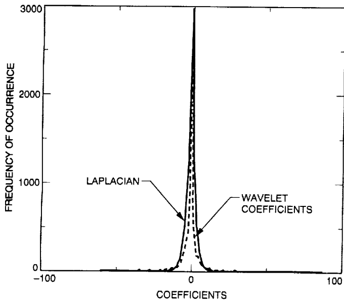
Fig. 1. Level DS-2 wavelet coefficients and Laplacian density.
