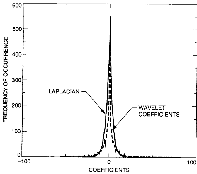
Fig. 2. Level DS-3 wavelet coefficients and Laplacian density.
