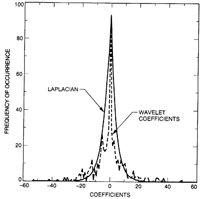
Fig. 3. Level DS-4 wavelet coefficients and Laplacian density.
