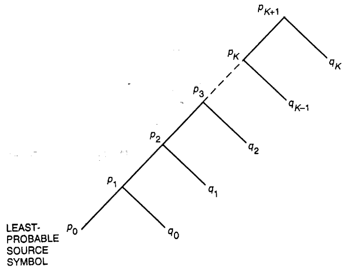
Fig. 2. A portion of an efficient code tree, in which the longest codeword has length \geq K + 1 . p_0 is the least source probability.
