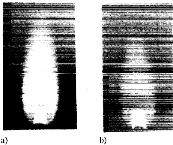
Figure 1. Image of a 7% hydrogen in air premixed flame obtained using a visible to near-infrared intensified array camera. The image is at 0.2 sec following spark ignition in a closed vessel.
