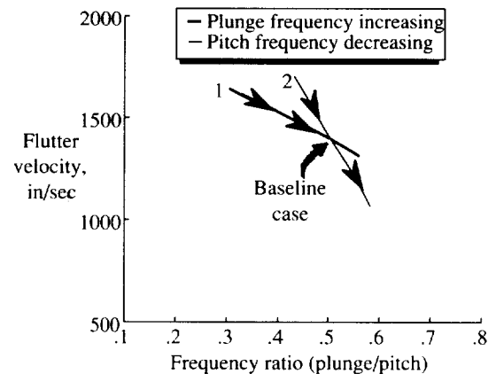
Figure A2. Influence of frequency ratio on the flutter velocity.
